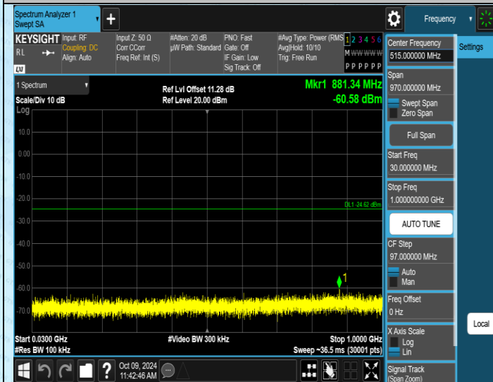
11N40SISO-Ant2-2422-30~1000-PASS
