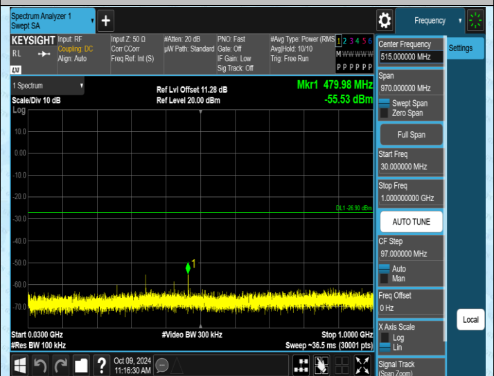
11N40SISO-Ant1-2422-30~1000-PASS
