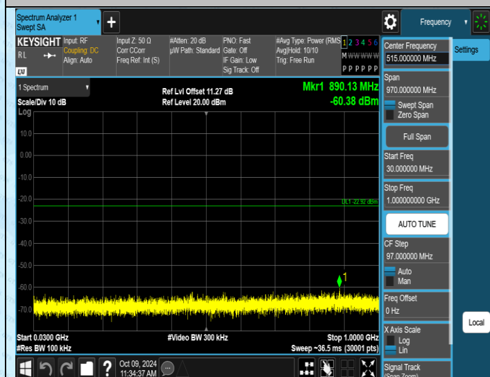
11G-Ant2-2437-30~1000-PASS
