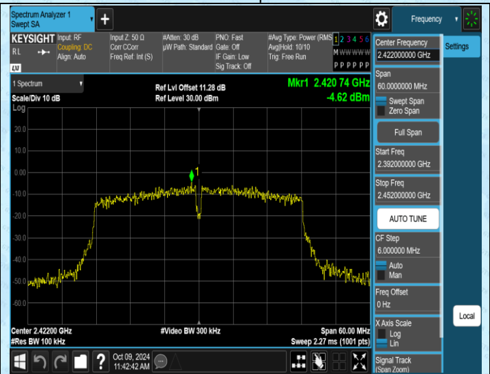
11N40SISO-Ant2-2422-0~Reference-PASS
