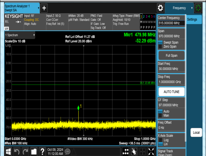
11N20SISO-Ant1-2437-30~1000-PASS
