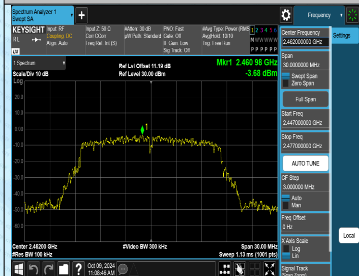
11G-Ant1-2462-0~Reference-PASS
