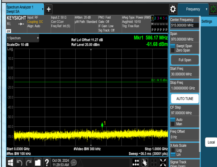
11B-Ant2-2437-30~1000-PASS
