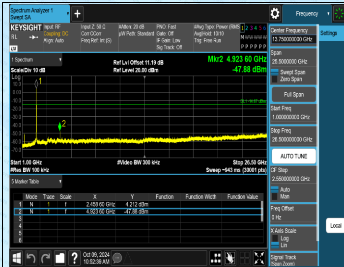
11B-Ant1-2462-1000~26500-PASS
