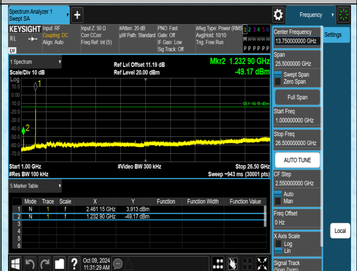
11B-Ant2-2462-1000~26500-PASS
