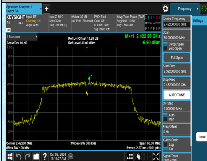
11N40SISO-Ant1-2422-0~Reference-PASS
