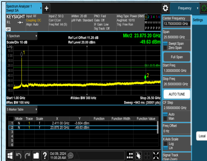
11G-Ant1-2412-1000~26500-PASS
