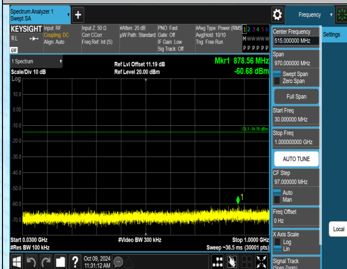
11B-Ant2-2462-30~1000-PASS
