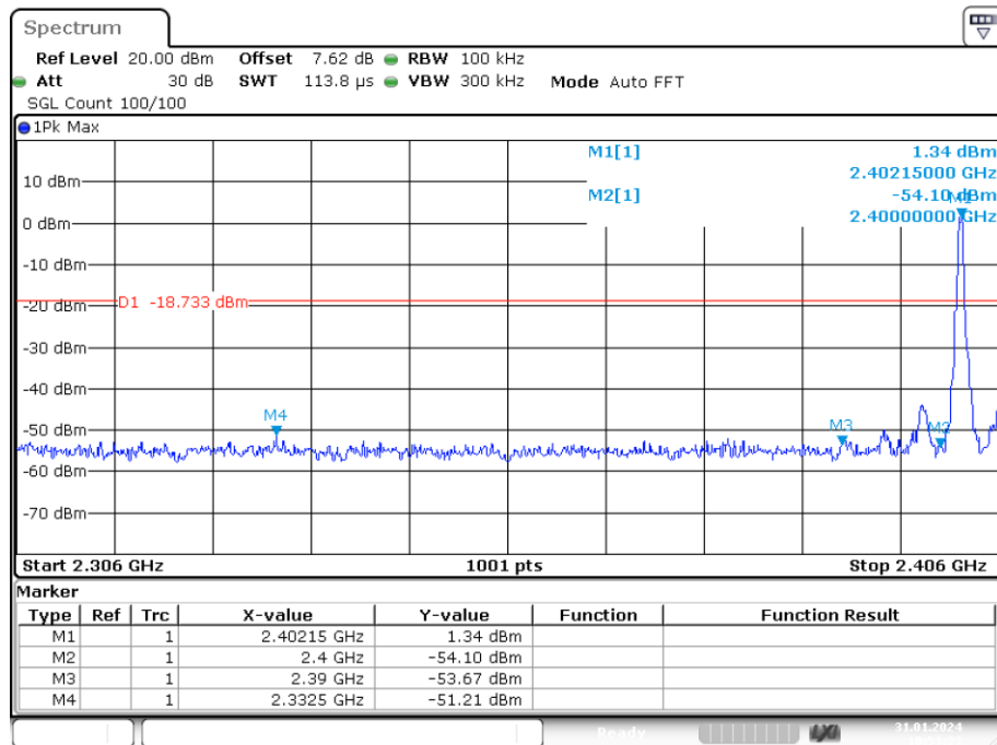
Band Edge NVNT user 2402MHz Ant1 Emission
