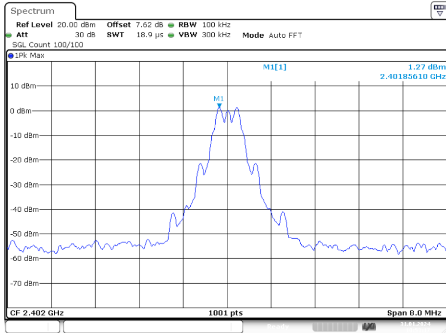
Band Edge NVNT user 2402MHz Ant1 Ref
