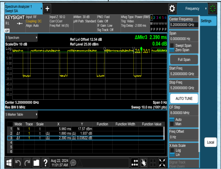
NTNV-11N20SISO-Ant1-5200
