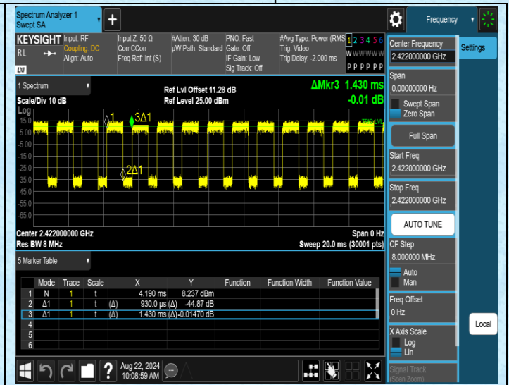
NTVN-11N40SISO-Ant1-2422
