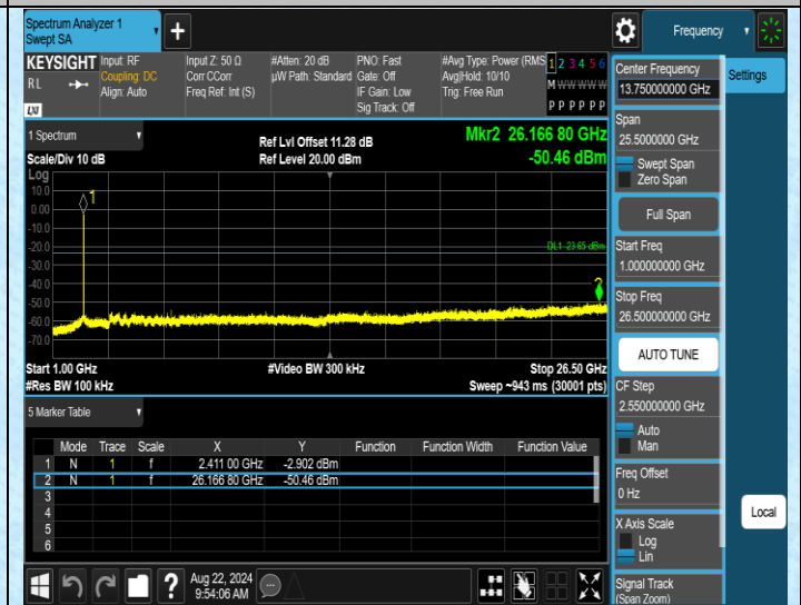
11G-Ant1-2412-1000~26500-PASS
