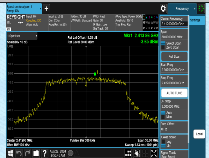
11G-Ant1-2412-0~Reference-PASS
