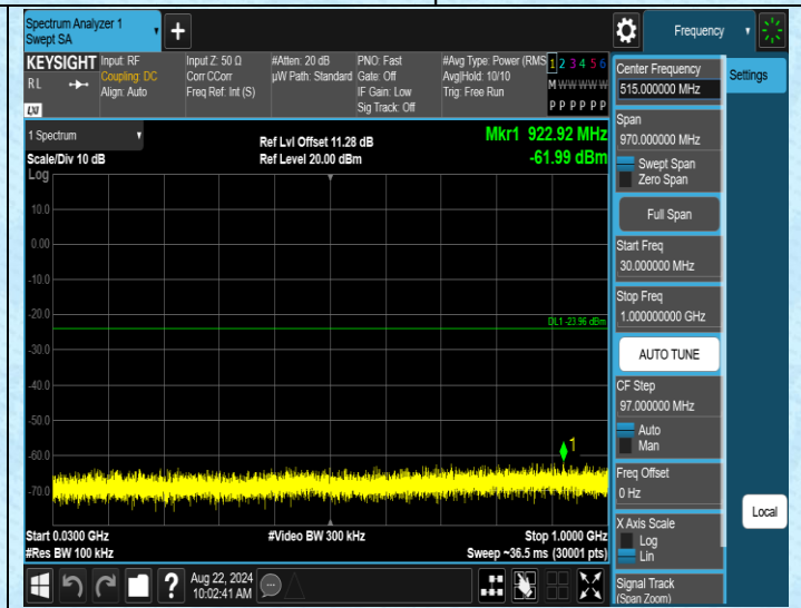
11N20SISO-Ant1-2412-30~1000-PASS
