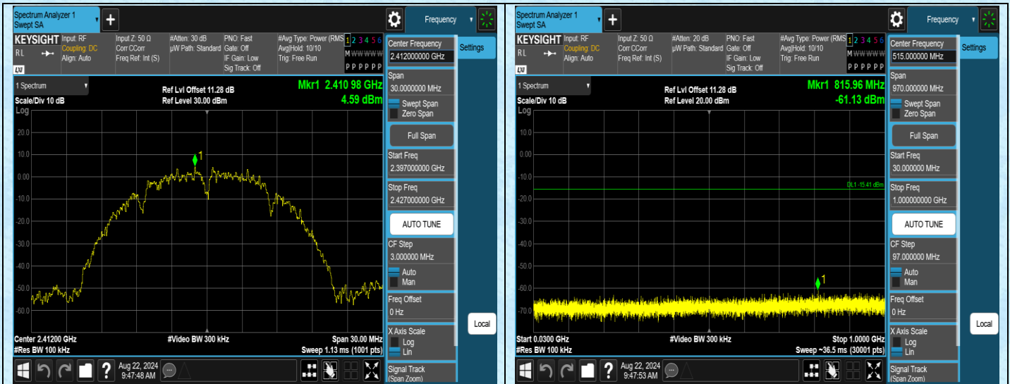
11B-Ant1-2412-0~Reference-PASS
