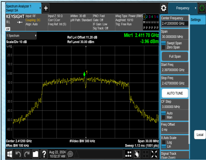
11N20SISO-Ant1-2412-0~Reference-PASS
