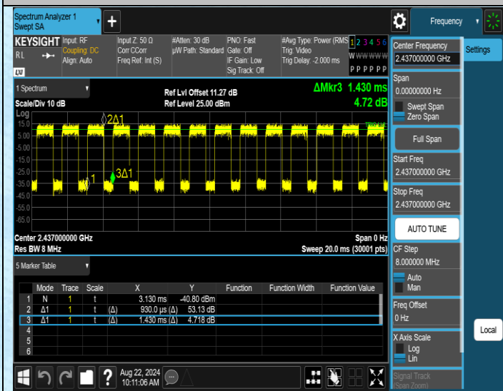
NTVN-11N40SISO-Ant1-2437
