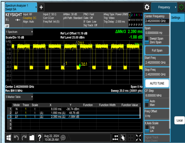
NTVN-11N20SISO-Ant1-2462
