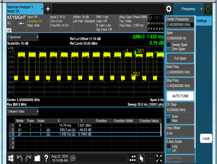
NTVN-11N40SISO-Ant1-2452
