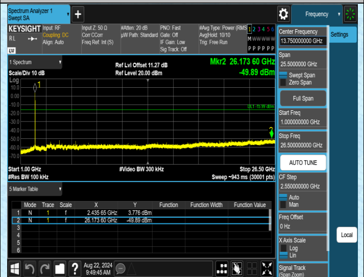
11B-Ant1-2437-1000~26500-PASS
