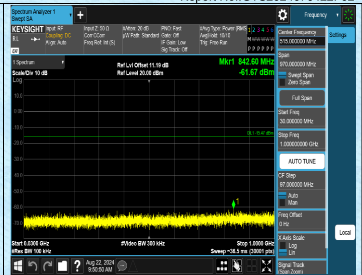
11B-Ant1-2462-30~1000-PASS
