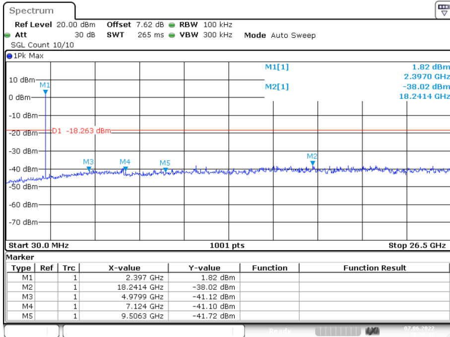
Tx. Spurious NVNT user 2402MHz Ant2 Emission
