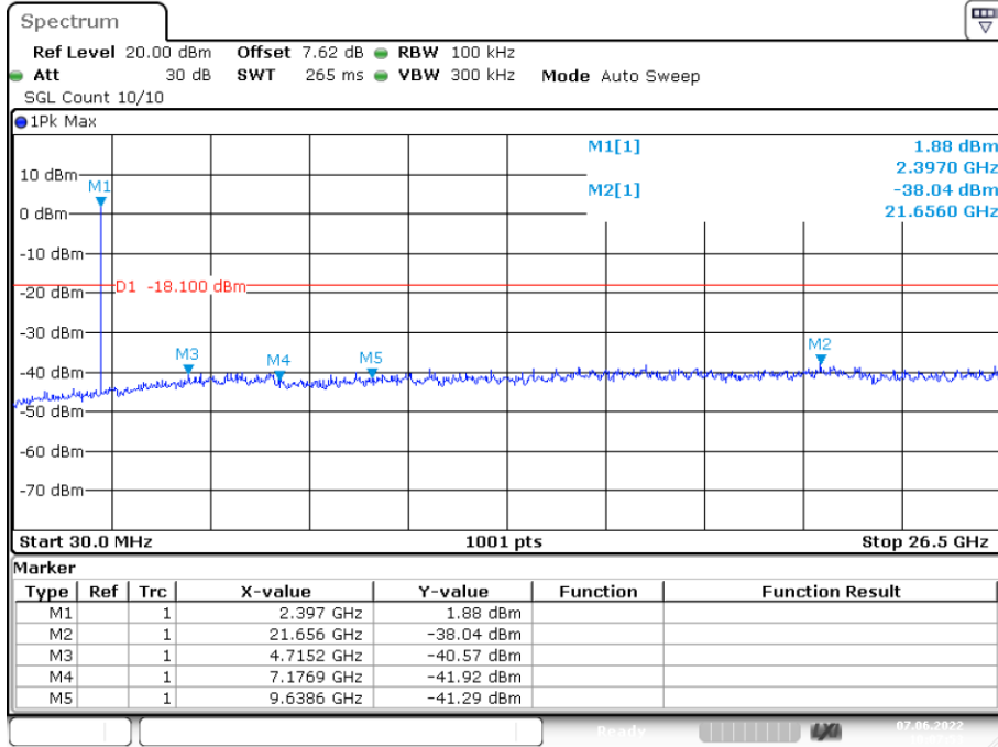
Tx. Spurious NVNT user 2402MHz Ant1 Emission
