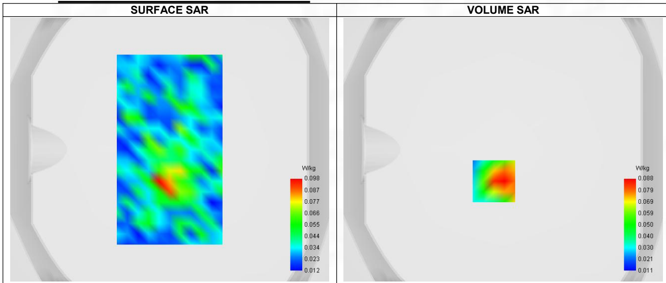
Maximum location: X=-7.00, Y=-24.00 ; SAR Peak: 0.19 W/kg
