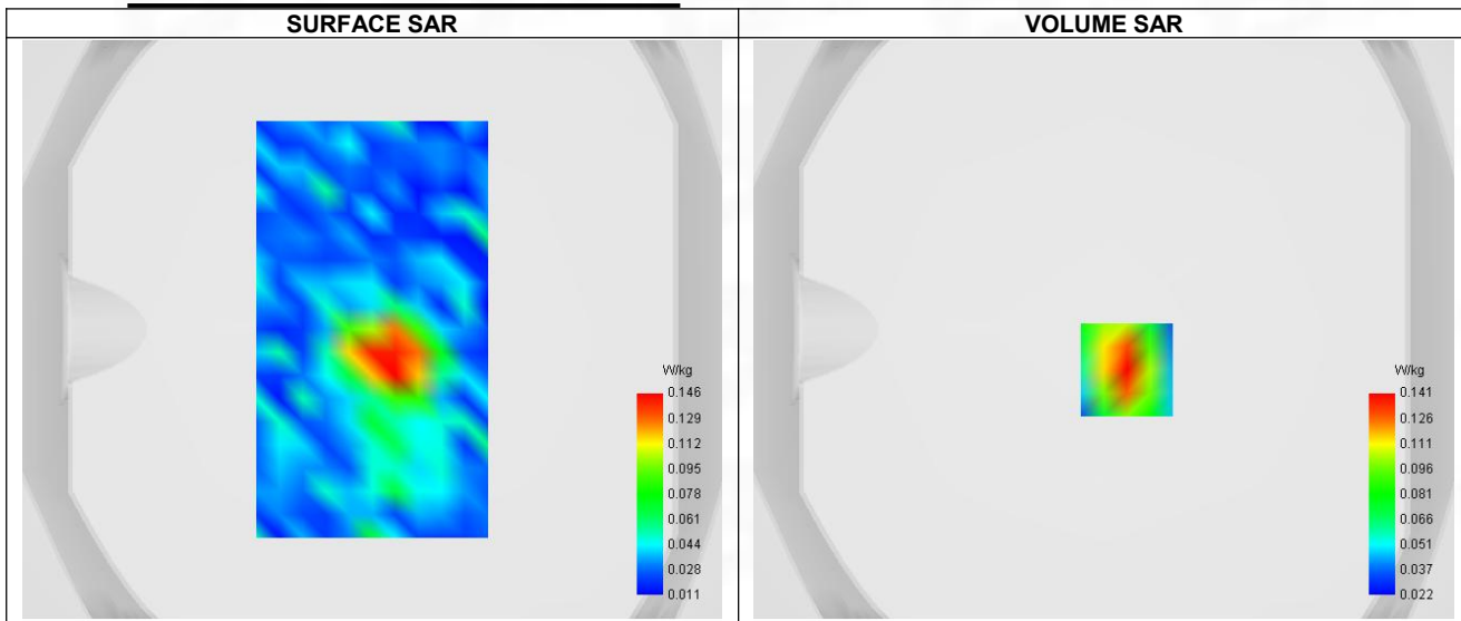
Maximum location: X=8.00, Y=-14.00 ; SAR Peak: 0.21 W/kg
