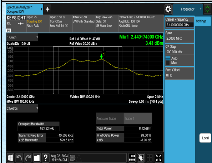
TX-Ant4-2440
