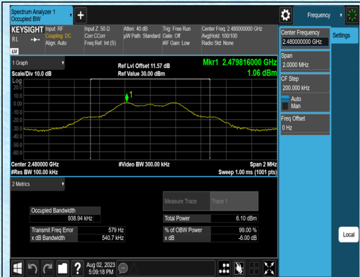
TX-Ant3-2480
