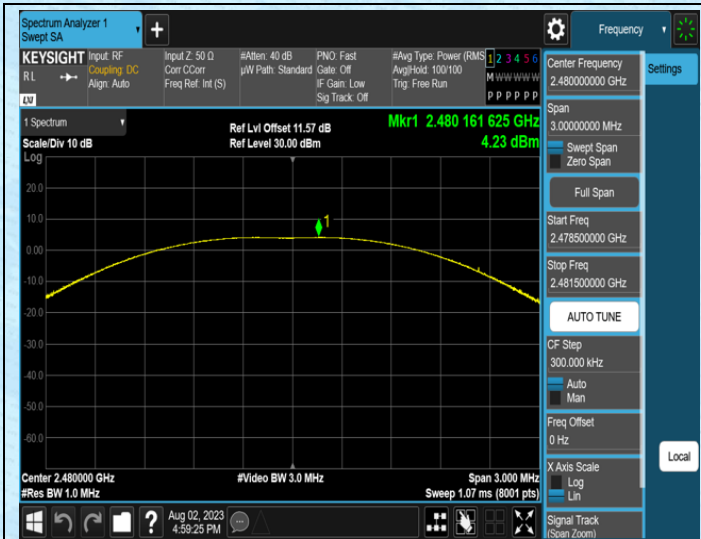
TX-Ant1-2480
