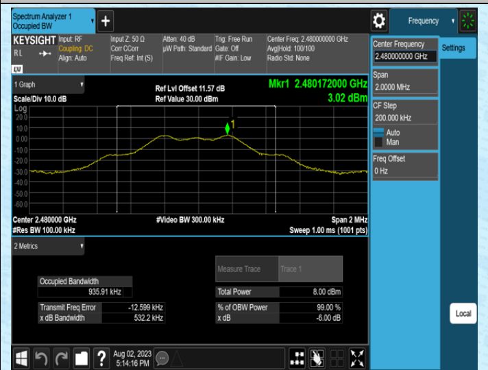
TX-Ant4-2480
