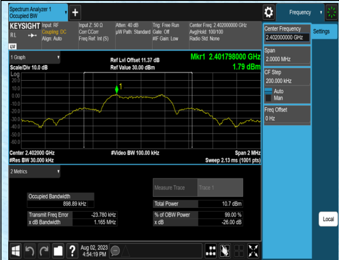
TX-Ant1-2402
