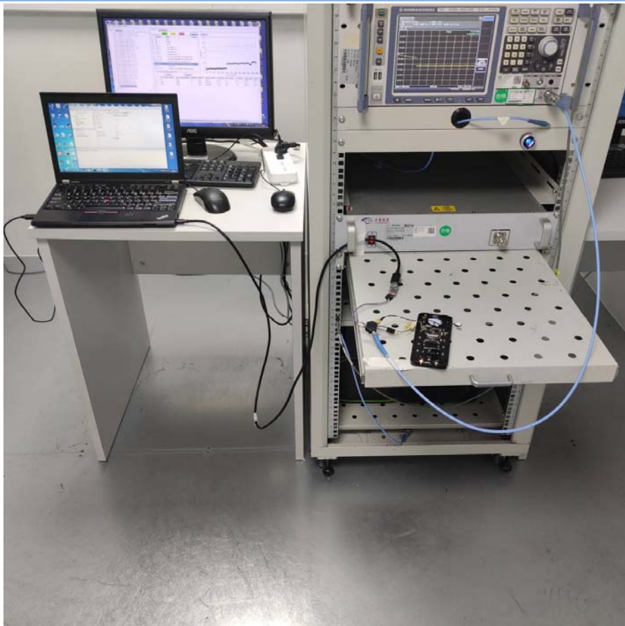
Conducted Test-BLE
