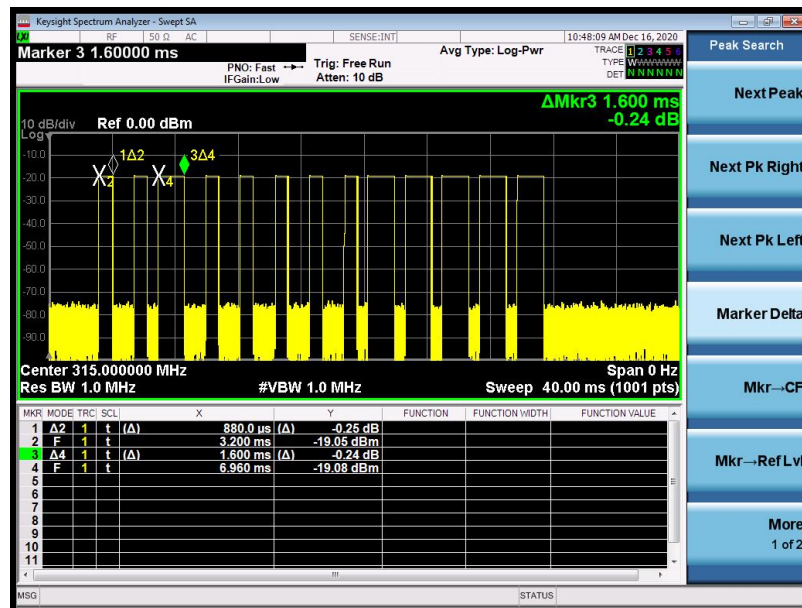
T_{on} time
