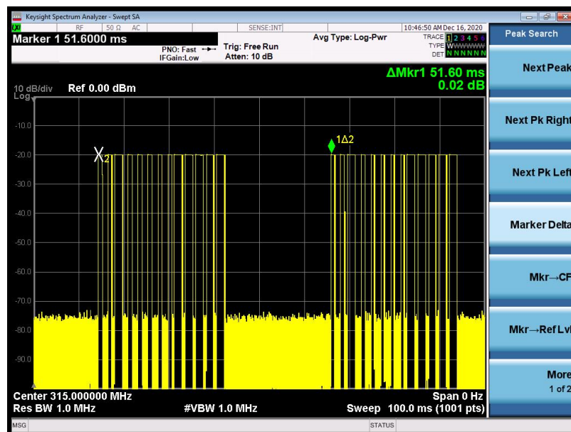
T_{period} time
