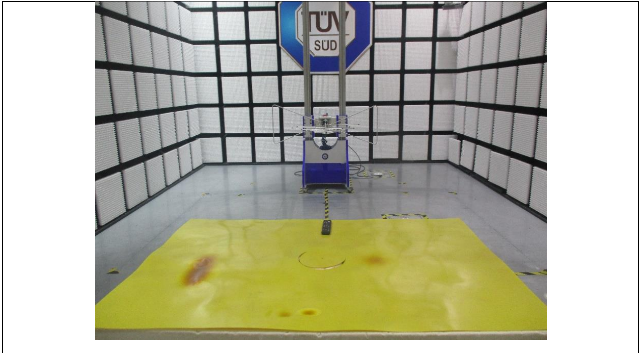
Radiated Emission test (1-18GHz)
