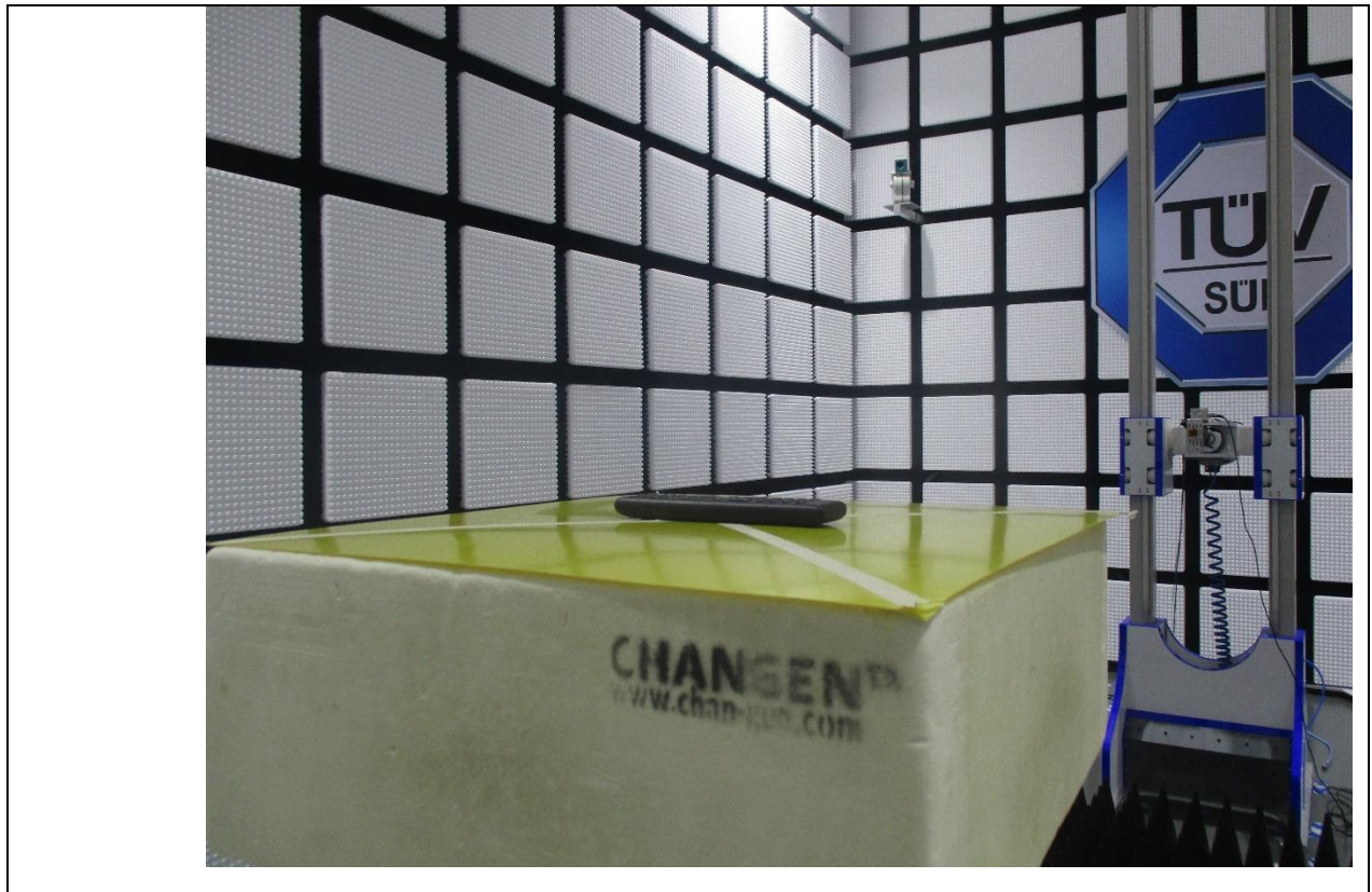
Radiated Emission test (above 18GHz)
