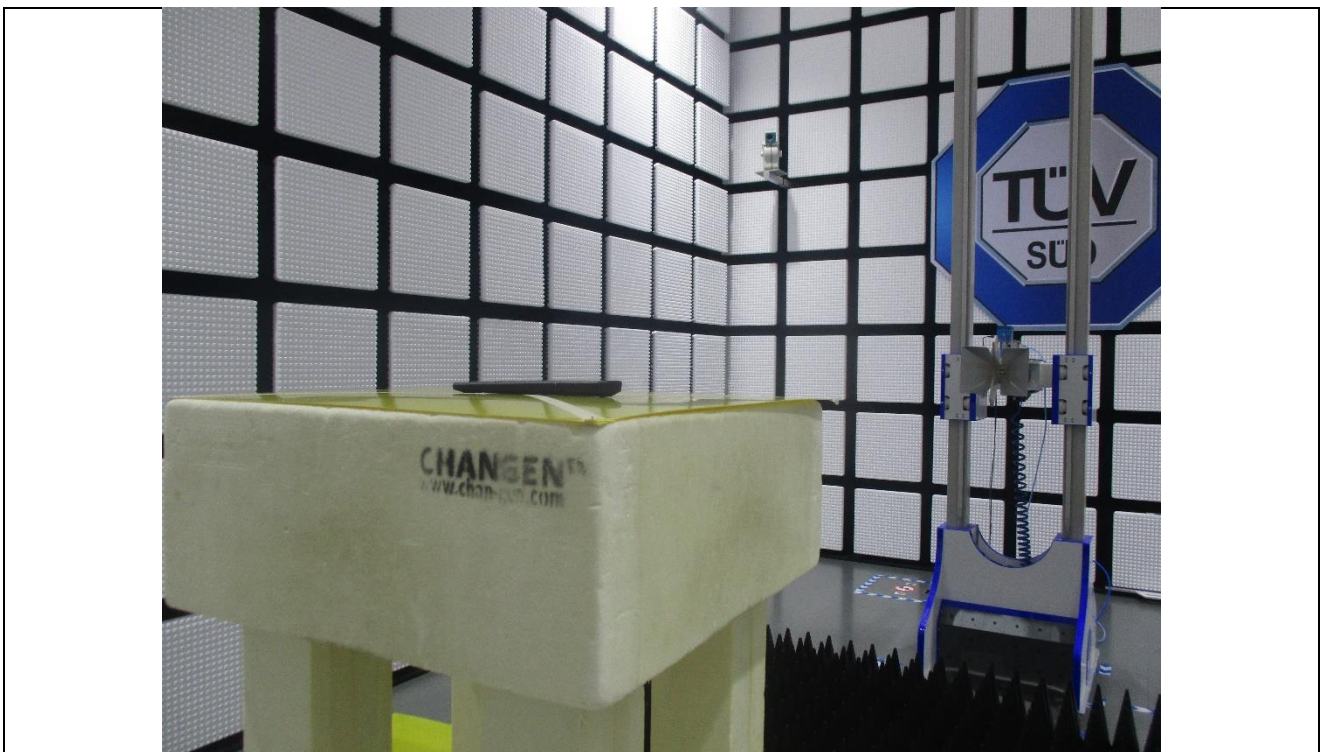
Radiated Emission test (1-18 GHz)
