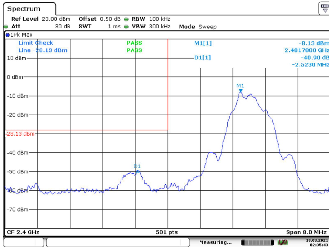
BLE, Band Edge, Left Side
