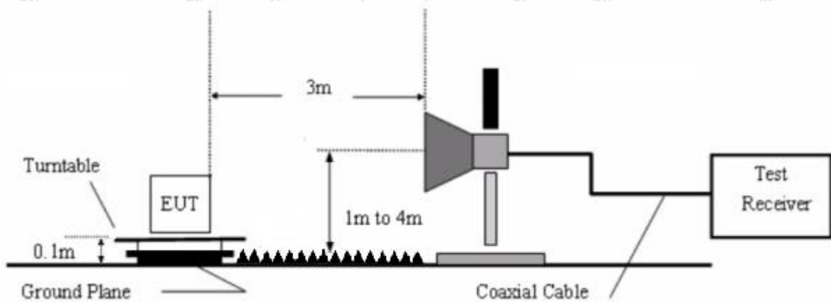
Figure 3. Above 1 GHz
