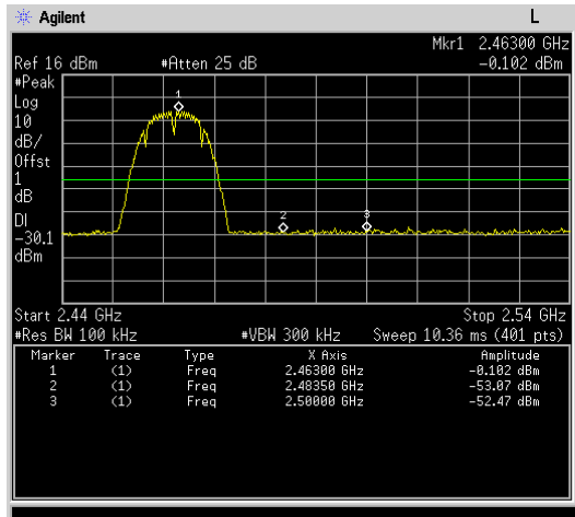
Right bandedge
