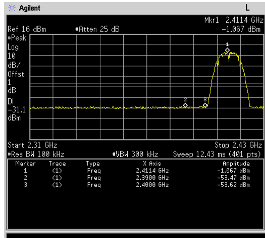
Left bandedge
