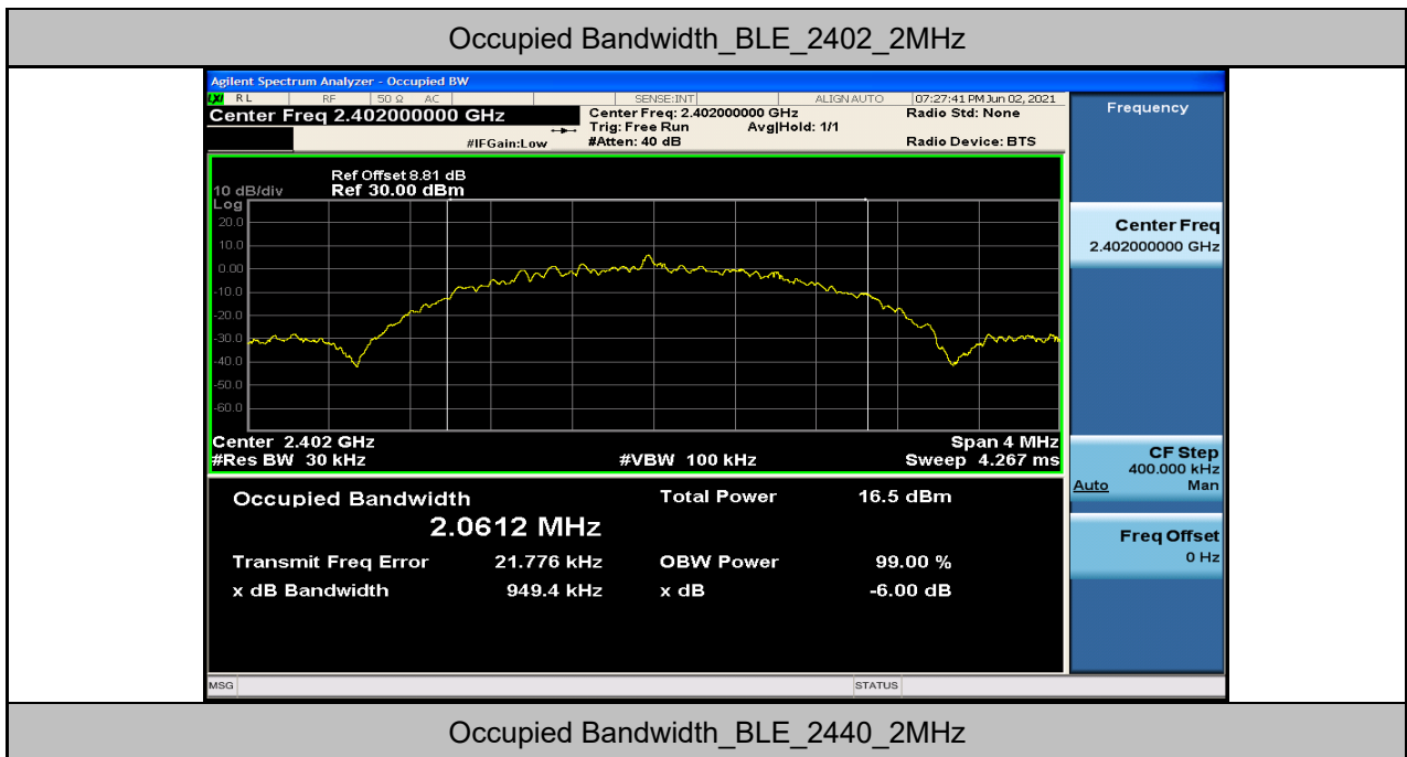
Occupied Bandwidth_BLE_2402_2MHz Occupied Bandwidth_BLE_2440_2MHz
