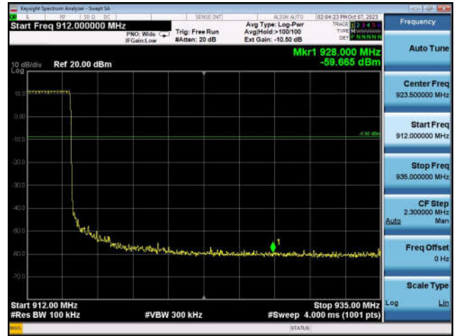
Conducted Band Edge: 914.9MHz_Hopping
