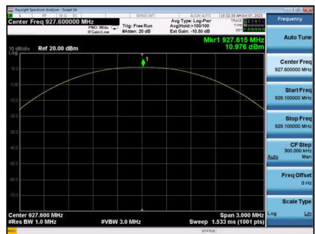
Conducted Output Power: 927.6MHz
