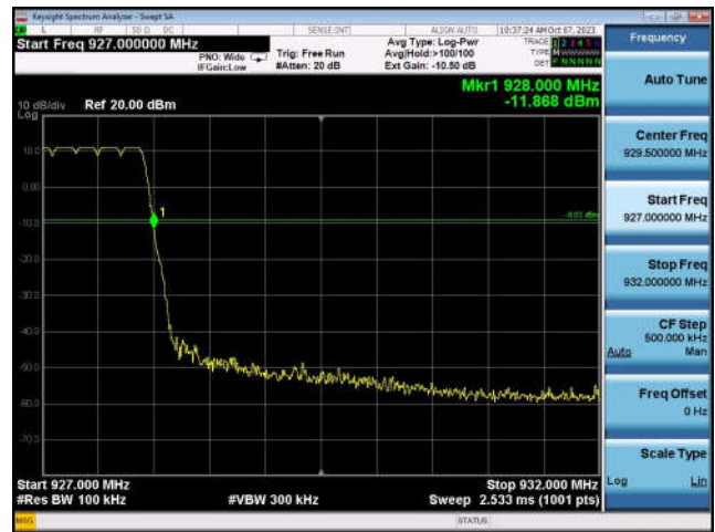
Conducted Band Edge: 927.6MHz_Hopping
