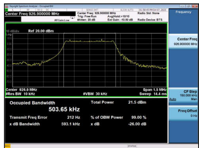
99% OBW: 926.9MHz
