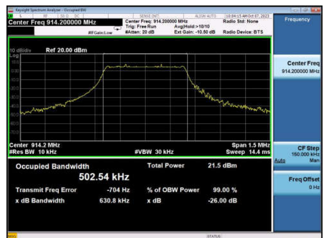
99% OBW: 914.2MHz
