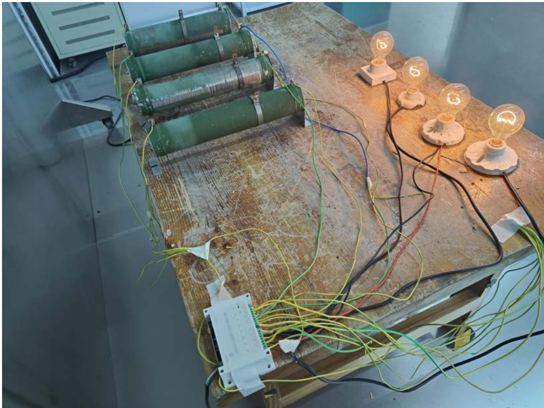
Conducted Emissions Side View- Switch Type
