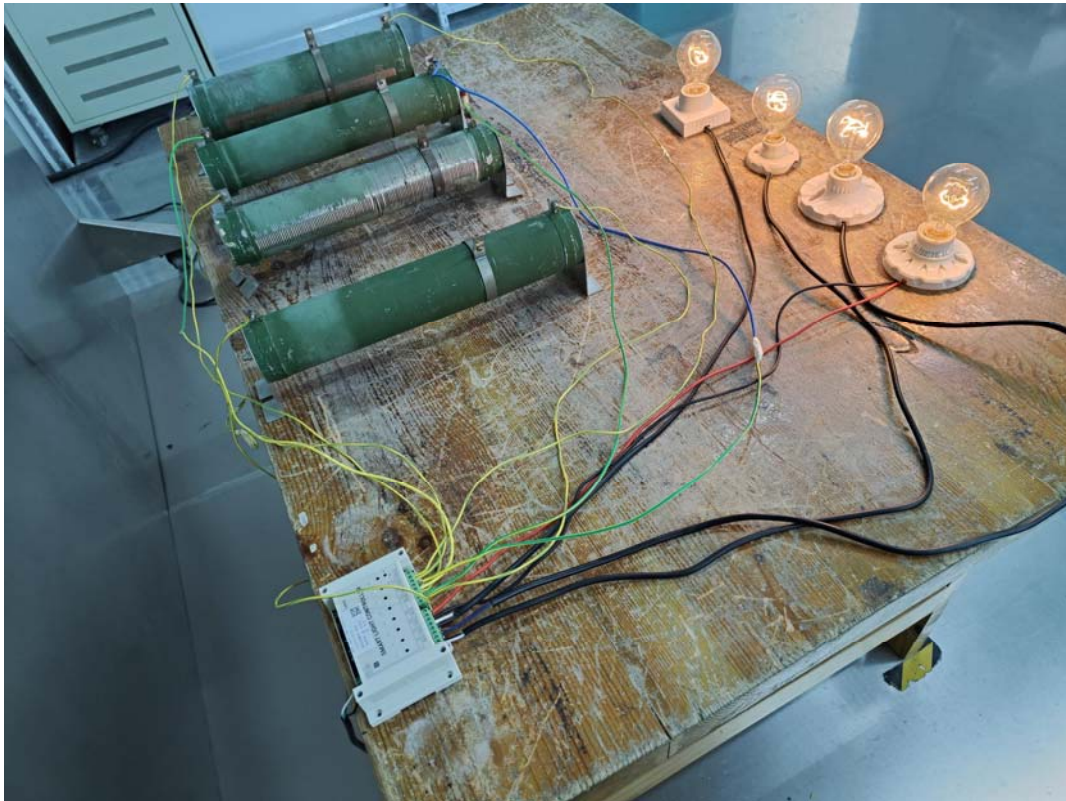
Conducted Emissions Side View- LN Type
