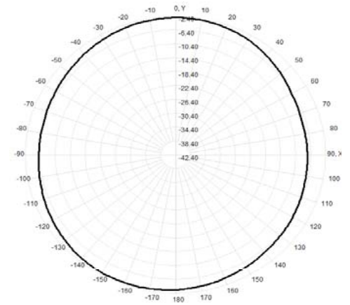
Total(H-XY), Max=-2.75dBi, CirD=4.81
