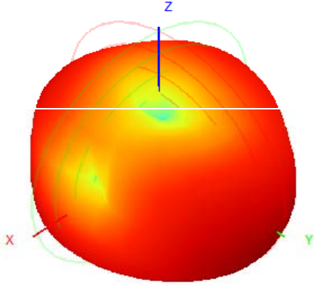
927.0MHz H+V, Eff: 17.7%
