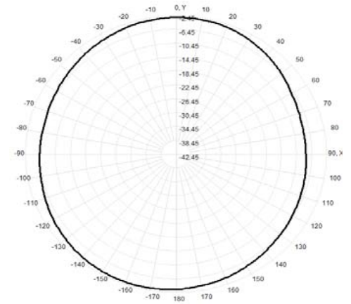
Total(H-XY), Max= -2.93dBi, CirD=5.19
