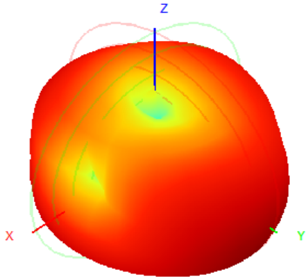
926.0MHz H+V, Eff: 18.0%
