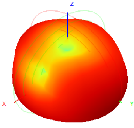
908.0MHz H+V, Eff: 24.1%
