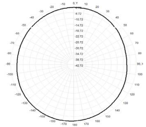
Total(H-XY), Max=-3.26dBi, CirD=5.75
