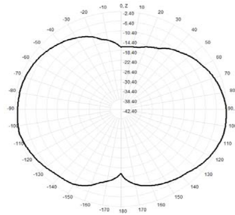
907.0MHz Total(E2-YZ), Max=-2.40dBi
