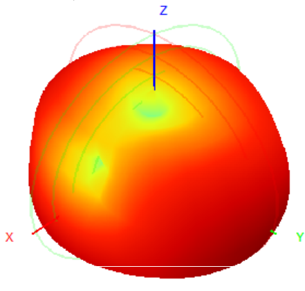
910.0MHz H+V, Eff: 23.5%
