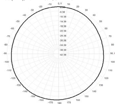
Total(H-XY), Max=-2.75dBi, CirD=4.76
