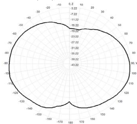
922.0MHz Total(E2-YZ), Max= -3.22dBi
