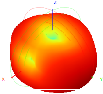
928.0MHz H+V, Eff: 17.3%
