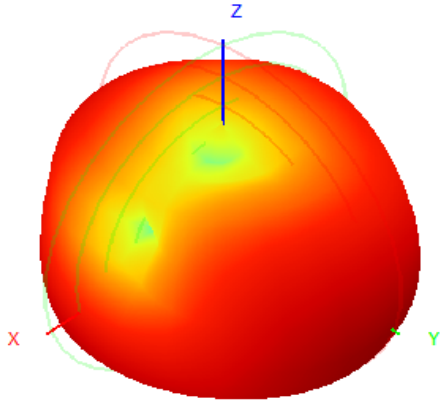
905.0MHz H+V, Eff: 24.3%
