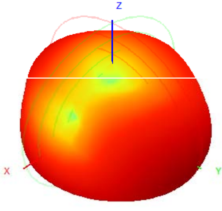
906.0MHz H+V, Eff: 24.2%
