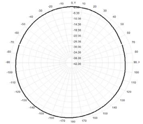
Total(H-XY), Max=-2.73dBi, CirD=4.99
