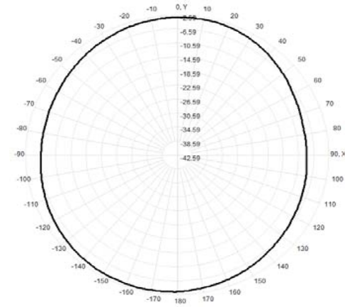
Total(H-XY), Max=-3.20dBi, CirD=5.45
