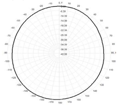
Total(H-XY), Max=-2.85dBi, CirD=5.06
