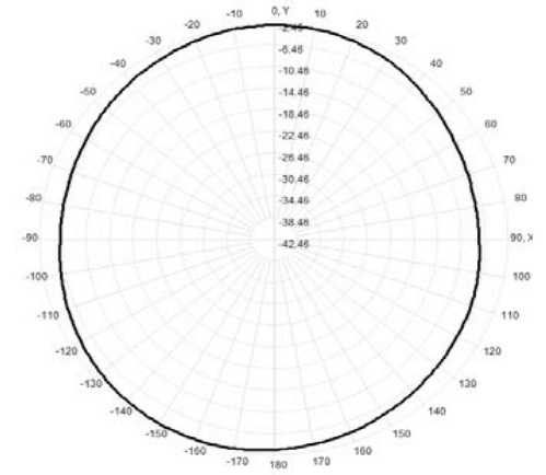
Total(H-XY), Max=-2.80dBi, CirD=4.80
