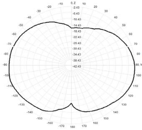
909.0MHz Total(E2-YZ), Max=-2.43dBi
