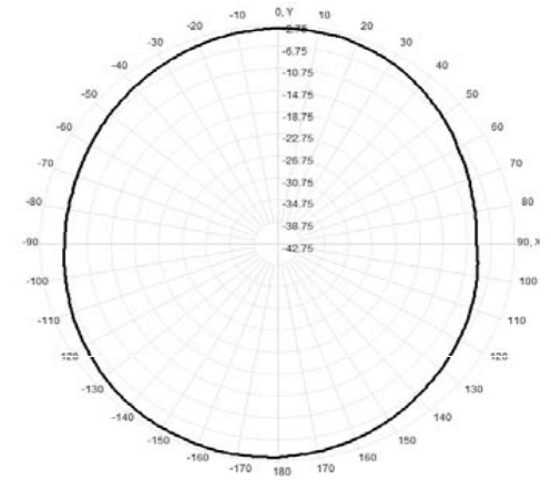
Total(H-XY), Max=-3.41dBi, CirD=5.96
