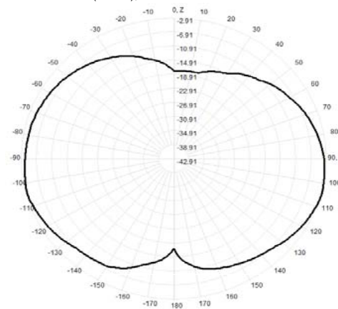
919.0MHz Total(E2-YZ), Max= -2.91dBi
