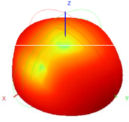
909.0MHz H+V, Eff: 23.9%
