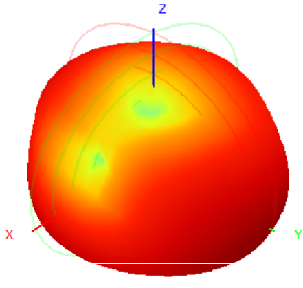
907.0MHz H+V, Eff: 24.2%
