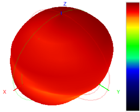
904.0MHz H+V, Eff: 18.0%
