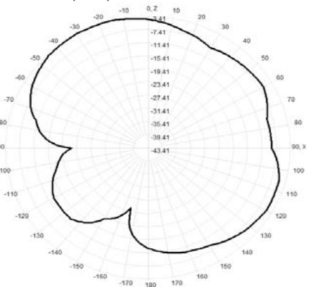
904.0MHz Total(E1-XZ), Max= -3.41dBi
