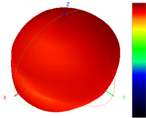
917.0MHz H+V, Eff: 22.7%
