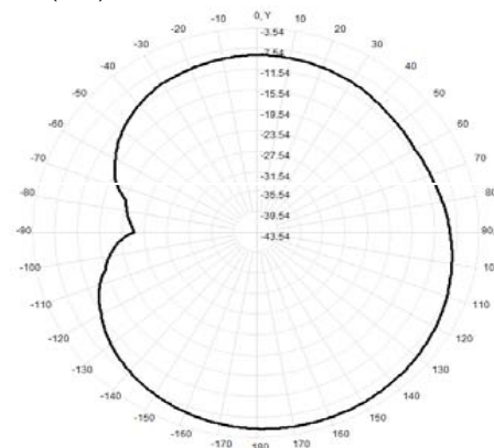
Total(H-XY), Max= -5.25dBi, CirD=16.54
