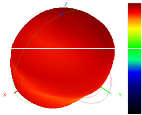
903.0MHz H+V, Eff: 17.6%
