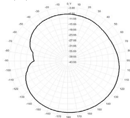
Total(H-XY), Max= -5.25dBi, CirD=15.82
