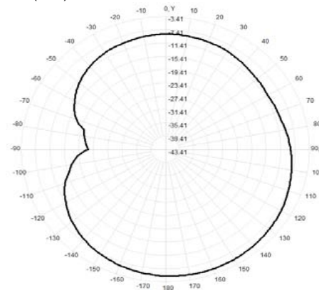
Total(H-XY), Max= -5.14dBi, CirD=16.94
