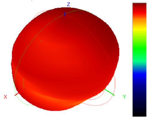
905.0MHz H+V, Eff: 18.5%
