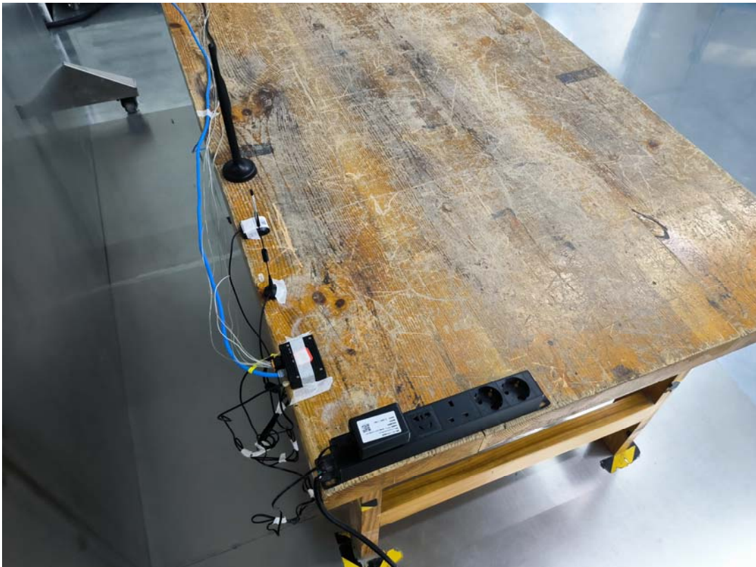
Conducted Emissions Side View-DC Adapter Mode
