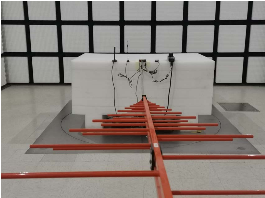
Radiated Emission Below 1GHz Rear View-DC Adapter Mode
