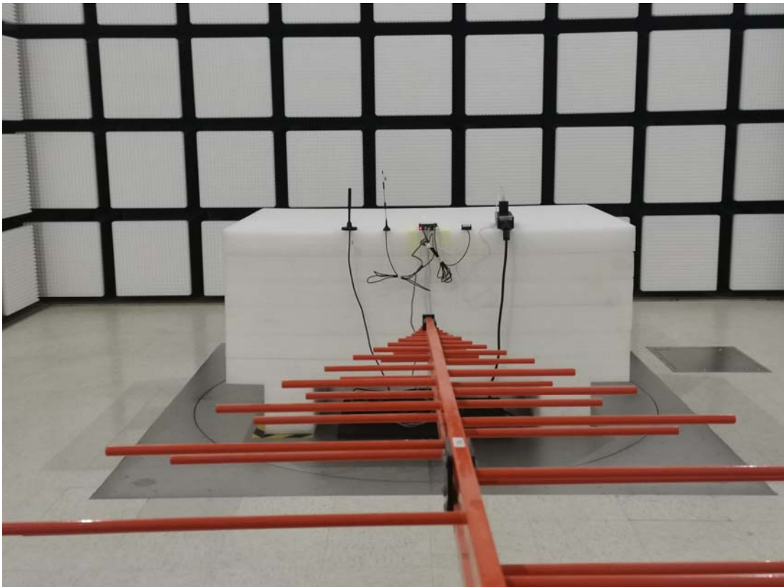
Radiated Emission Below 1GHz Rear View-USB Adapter Mode
