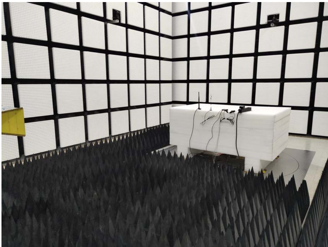
Radiated Emission Above 1GHz Rear View-DC Adapter Mode
