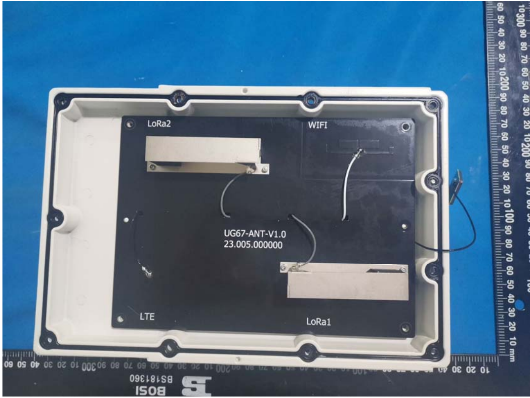
Antenna Board
