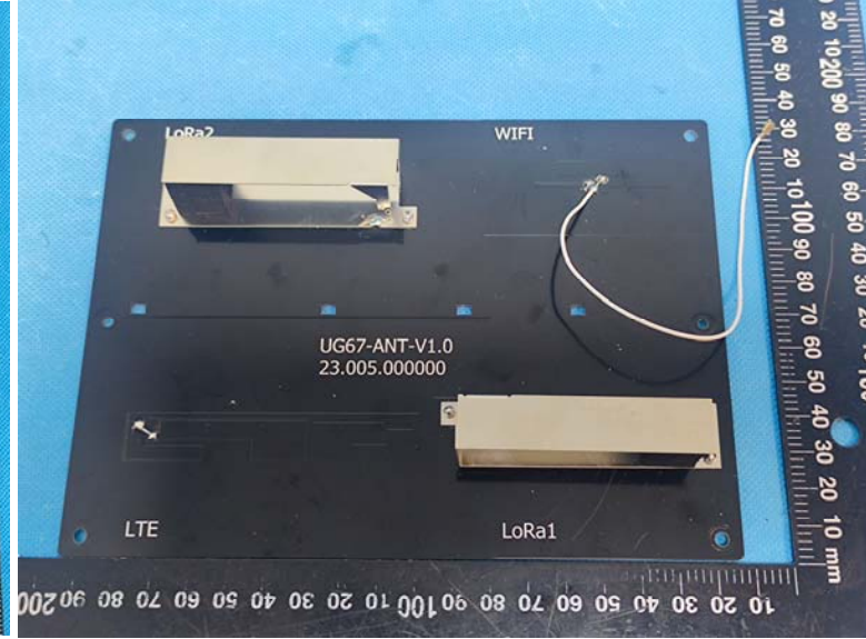
Antenna Board
