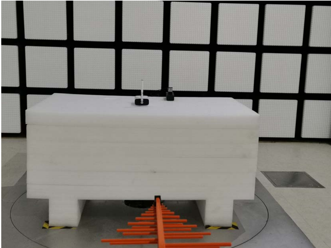
Radiated Emission Below 1GHz View-PoE mode
