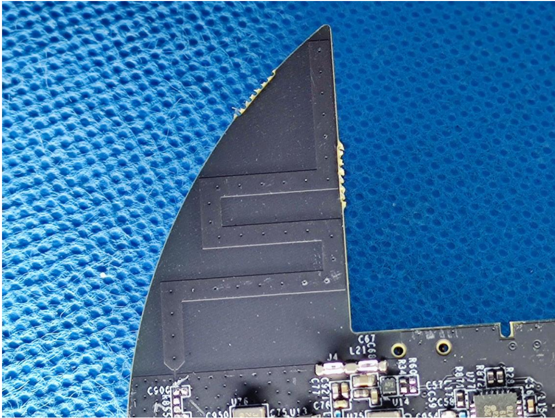
RX Antenna(Front Side)
