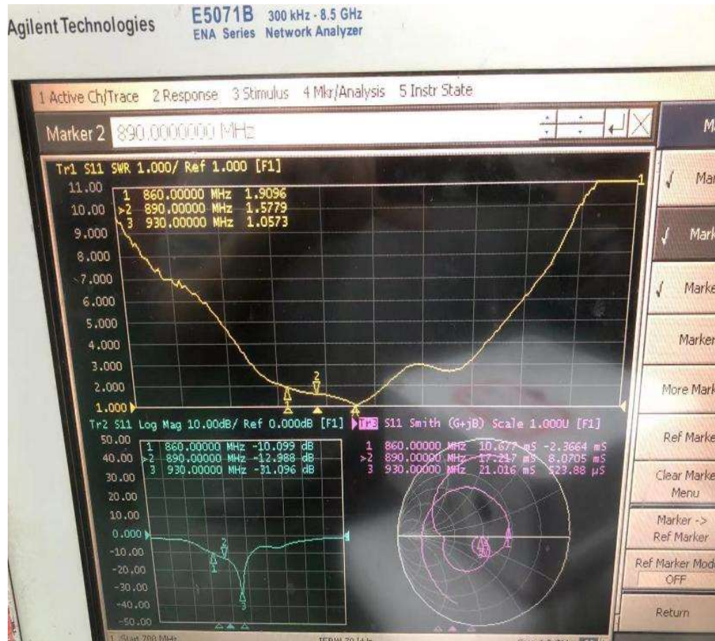
860-930MHz天线驻波图 The antenna standing wave figure
