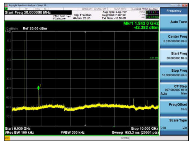
Conducted Spurious Emission: 927.8MHz
