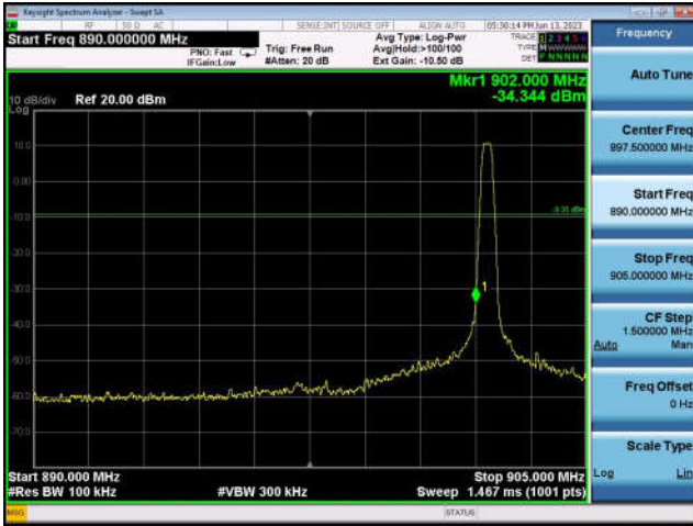
Conducted Band Edge: 902.3MHz_Hopping
