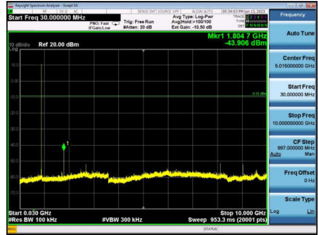
Conducted Spurious Emission: 908.7MHz
