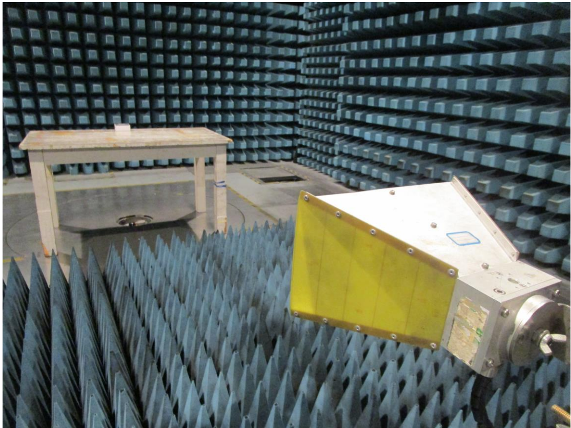
RE_Above 1GHz_Internal Ant
