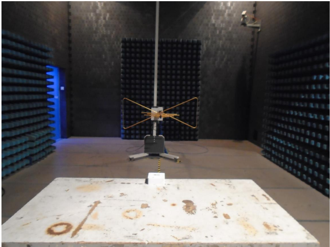
RE_Below 1GHz_Internal Ant
