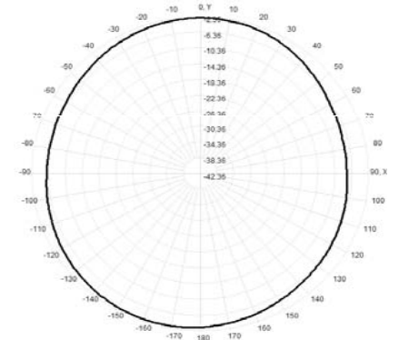
Total(H-XY), Max= -2.73dBi, CirD=4.99
