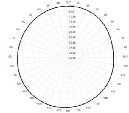
Total(H-XY), Max= -3.51dBi, CirD=6.02
