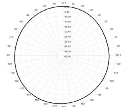
Total(H-XY), Max= -2.75dBi, CirD=4.81
