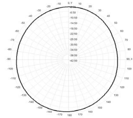
Total(H-XY), Max= -3.05dBi, CirD=5.53
