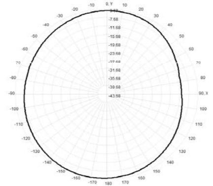
Total(H-XY), Max= -4.40dBi, CirD=6.95
