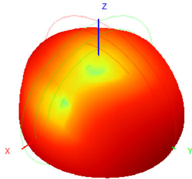
904.0MHz H+V, Eff: 24.4%
