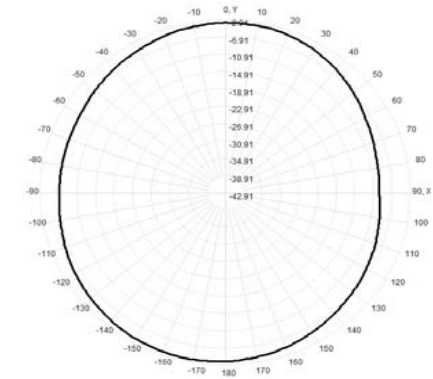
Total(H-XY), Max= -3.63dBi, CirD=6.22
