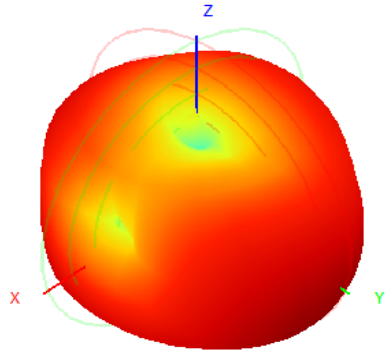
928.0MHz H+V, Eff: 17.3%
