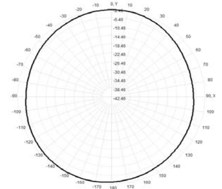
Total(H-XY), Max= -2.80dBi, CirD=4.80
