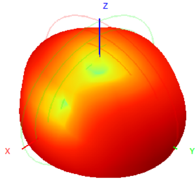
908.0MHz H+V, Eff: 24.1%
