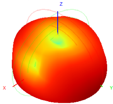
919.0MHz H+V, Eff: 20.3%
