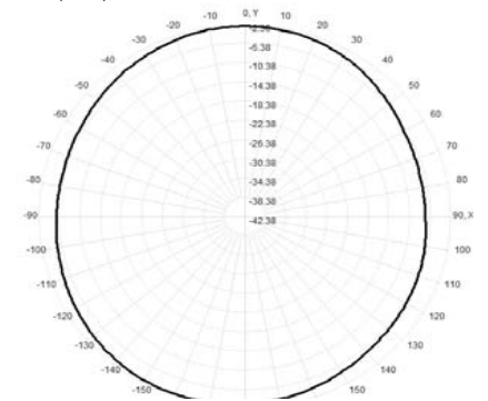
Total(H-XY), Max=-2.75dBi, CirD=4.76
