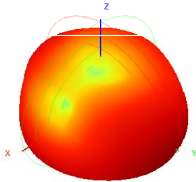
903.0MHz H+V, Eff: 24.4%
