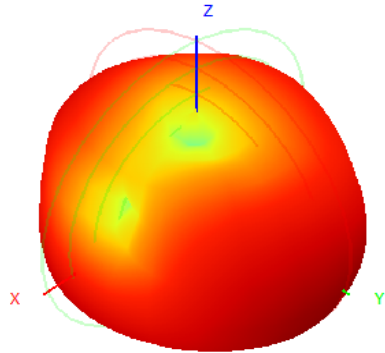
911.0MHz H+V, Eff: 23.3%
