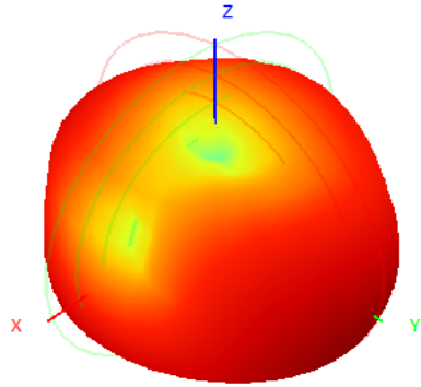
916.0MHz H+V, Eff: 21.4%
