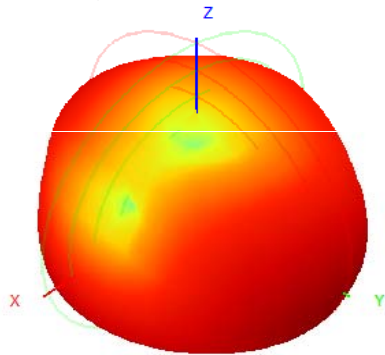
906.0MHz H+V, Eff: 24.2%
