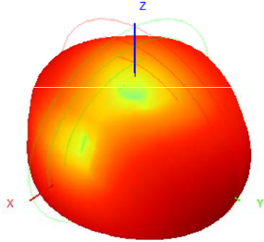
915.0MHz H+V, Eff: 21.8%
