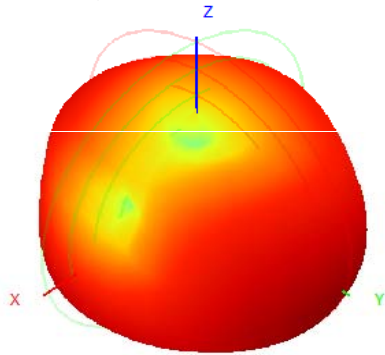
909.0MHz H+V, Eff: 23.9%
