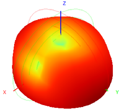
914.0MHz H+V, Eff: 22.2%
