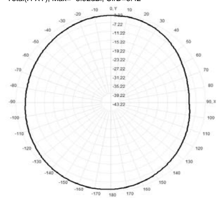
Total(H-XY), Max= -3.92dBi, CirD=6.42
