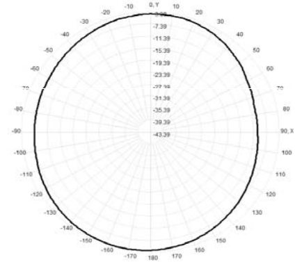
Total(H-XY), Max= -4.12dBi, CirD=6.55
