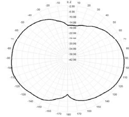
919.0MHz Total(E2-YZ), Max= -2.91dBi
