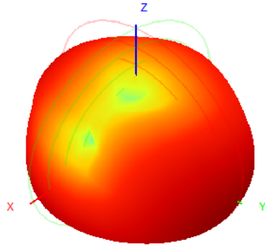
902.0MHz H+V, Eff: 24.6%
