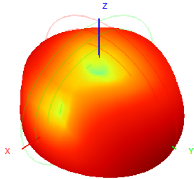
917.0MHz H+V, Eff: 20.9%
