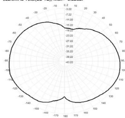
922.0MHz Total(E2-YZ), Max= -3.22dBi
