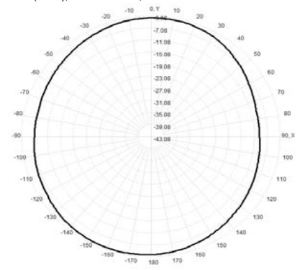
Total(H-XY), Max= -3.81dBi, CirD=6.07
