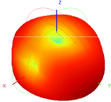
927.0MHz H+V, Eff: 17.7%
