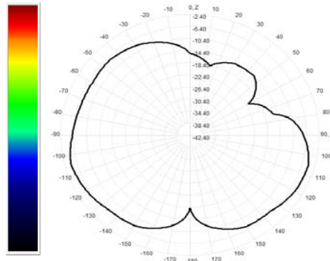
907.0MHz Total(E1-XZ), Max= -4.37dBi
