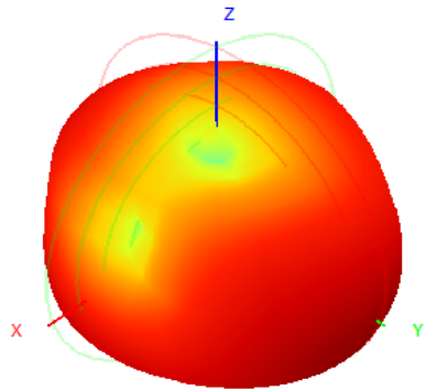
913.0MHz H+V, Eff: 22.6%
