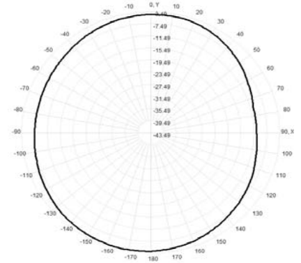
Total(H-XY), Max= -4.23dBi, CirD=6.60
