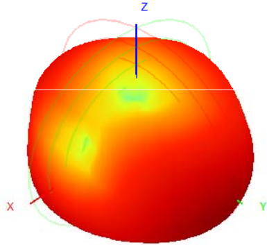
912.0MHz H+V, Eff: 23.0%
