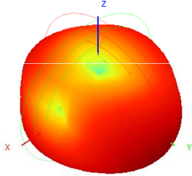
924.0MHz H+V, Eff: 18.7%
