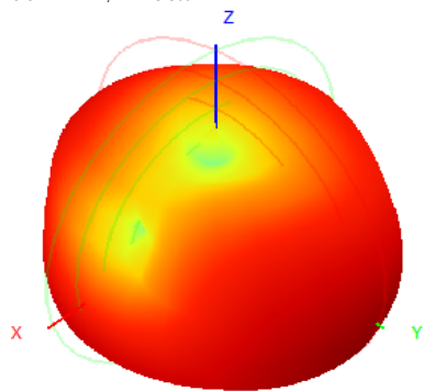
910.0MHz H+V, Eff: 23.5%
