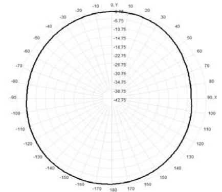
Total(H-XY), Max= -3.41dBi, CirD=5.96
