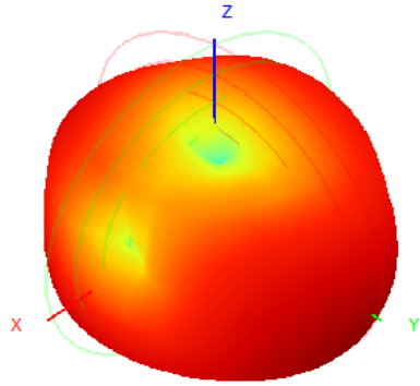
925.0MHz H+V, Eff: 18.4%
