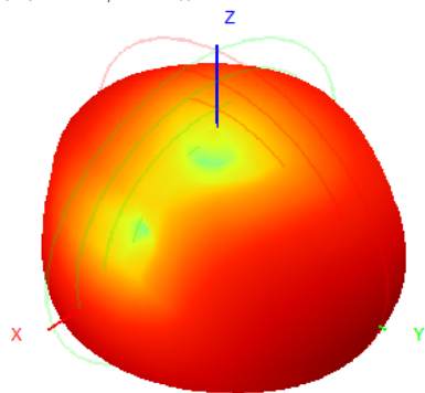
907.0MHz H+V, Eff: 24.2%
