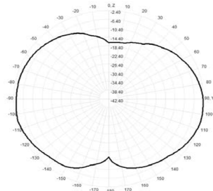
907.0MHz Total(E2-YZ), Max= -2.40dBi
