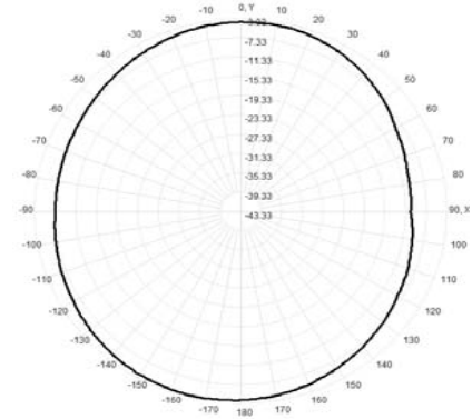
Total(H-XY), Max= -3.94dBi, CirD=6.57
