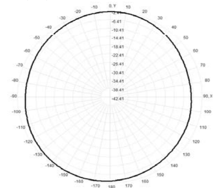
Total(H-XY), Max=-2.77dBi, CirD=4.70
