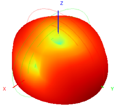
923.0MHz H+V, Eff: 19.1%
