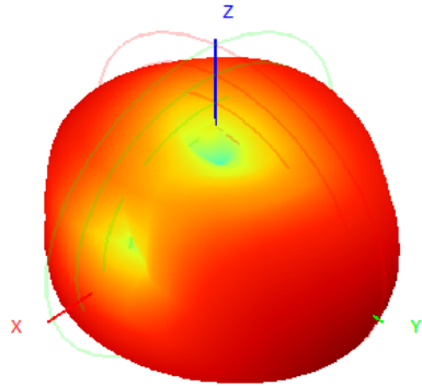
926.0MHz H+V, Eff: 18.0%
