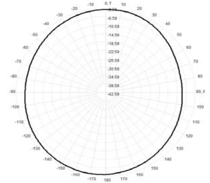
Total(H-XY), Max= -3.20dBi, CirD=5.45
