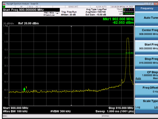
Conducted Band Edge: 915.2MHz_Hopping
