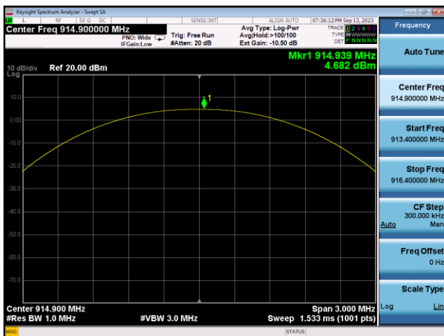
Conducted Output Power: 914.9MHz
