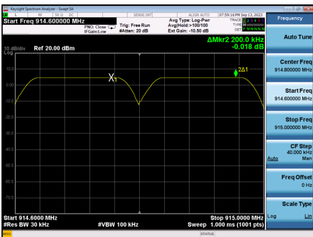
Carried Frequency Separation: 914.6~915.0MHz
