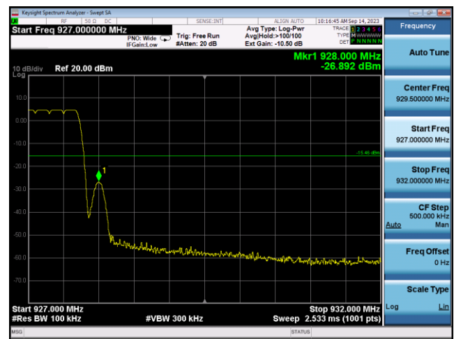
Conducted Band Edge: 927.6MHz_Hopping
