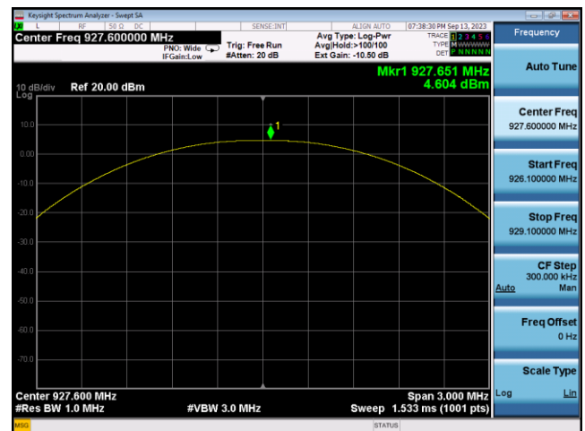
Conducted Output Power: 927.6MHz
