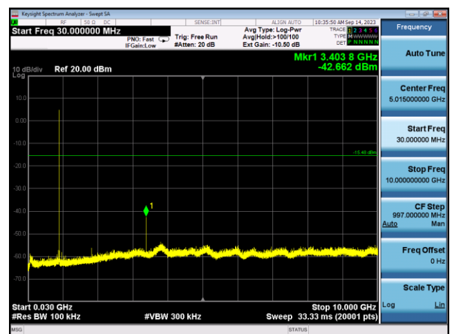
Conducted Spurious Emission: 927.6MHz
