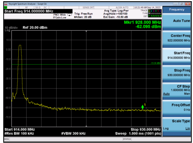
Conducted Band Edge: 914.9MHz_Hopping
