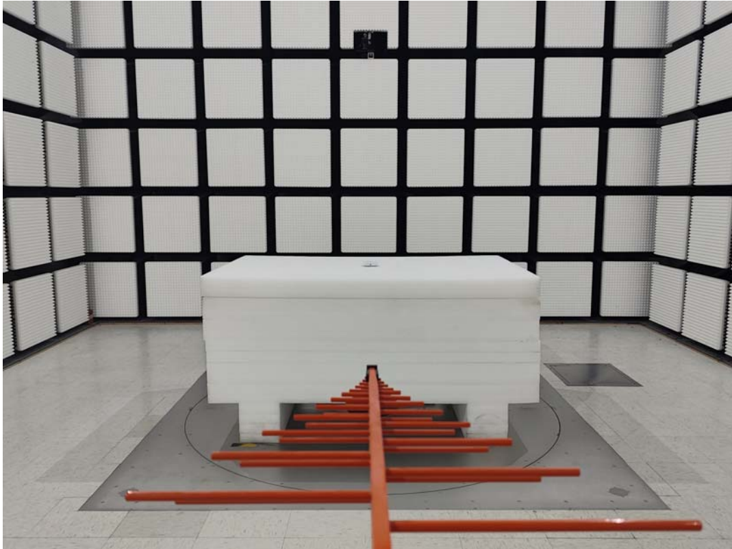
Radiated Emission Below 1GHz View- VS340-915M
