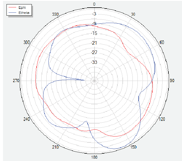
Phi=0 freq=2400MHz
