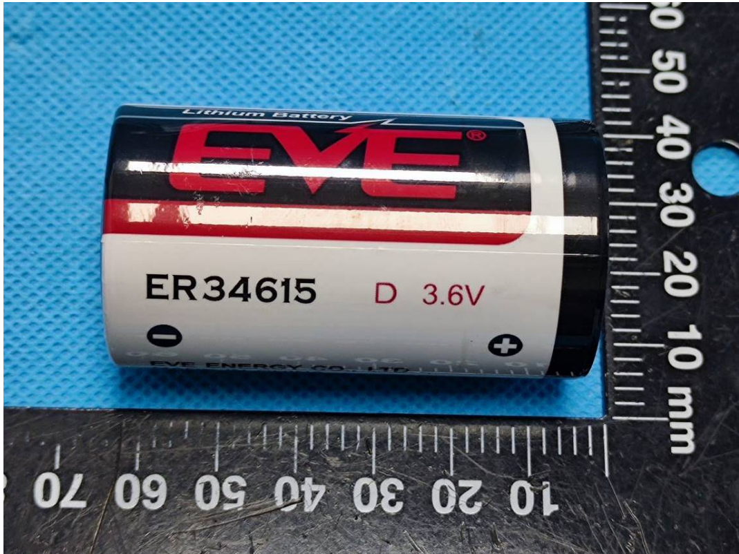
Battery 1#
