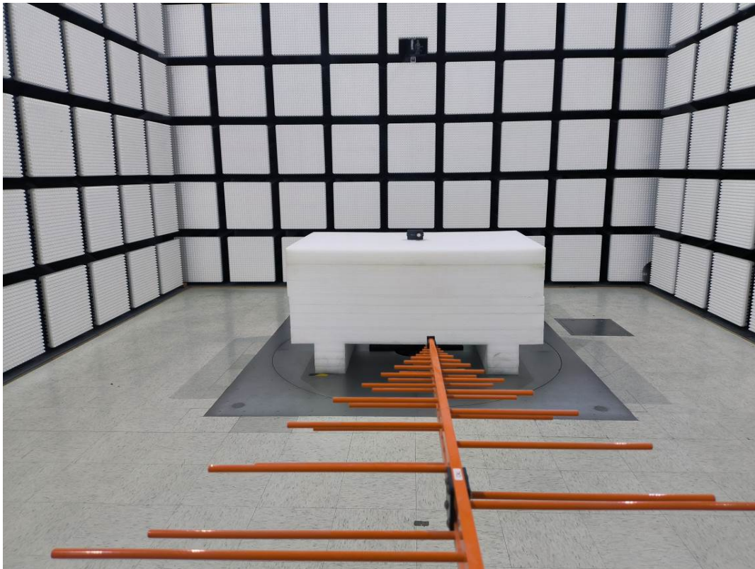
Radiated Emission Below 1GHz View EM400-UDL-915M C100
