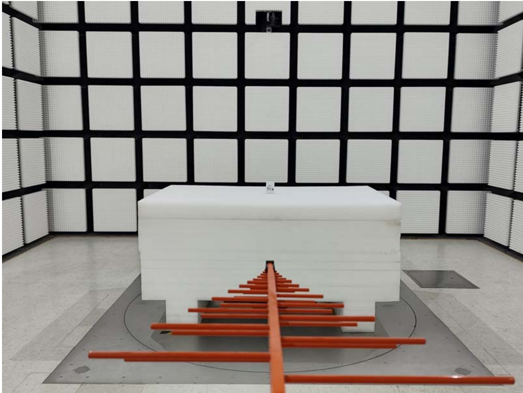
Radiated Emission Below 1GHz View EM320-TILT-915M
