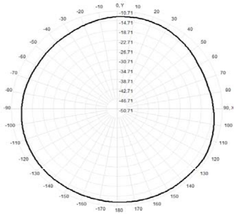
Total(H-XY), Max= -12.04dBi, CirD=3.71
