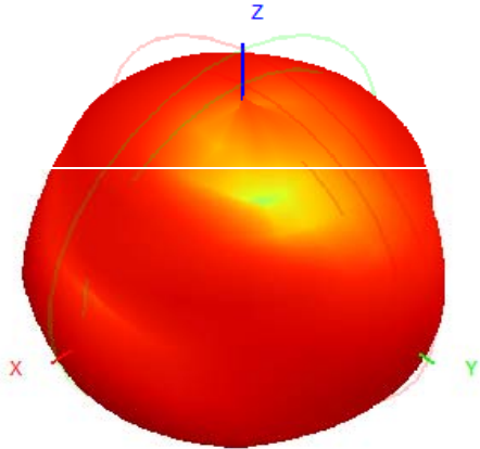
906.0MHz H+V, Eff: 2.0%
