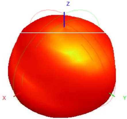
927.0MHz H+V, Eff: 3.8%
