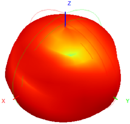
902.0MHz H+V, Eff: 1.8%
