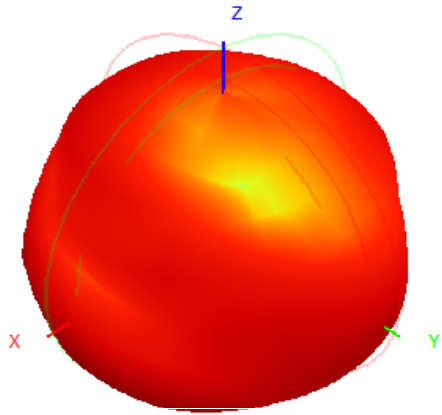
916.0MHz H+V, Eff: 2.5%
