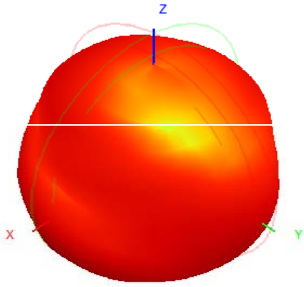
921.0MHz H+V, Eff: 3.1%
