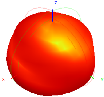
928.0MHz H+V, Eff: 3.9%
