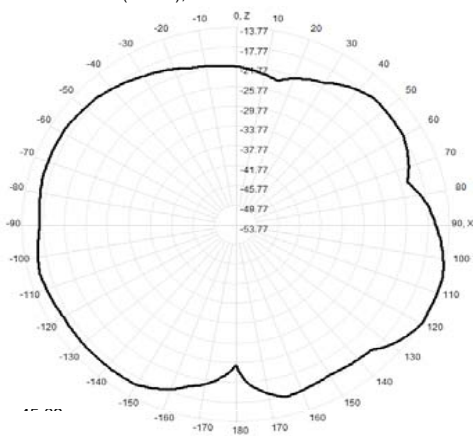
910.0MHz Total(E1-XZ), Max= -13.77dBi
