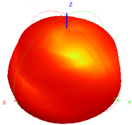
920.0MHz H+V, Eff: 3.0%
