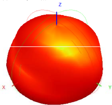
918.0MHz H+V, Eff: 2.8%
