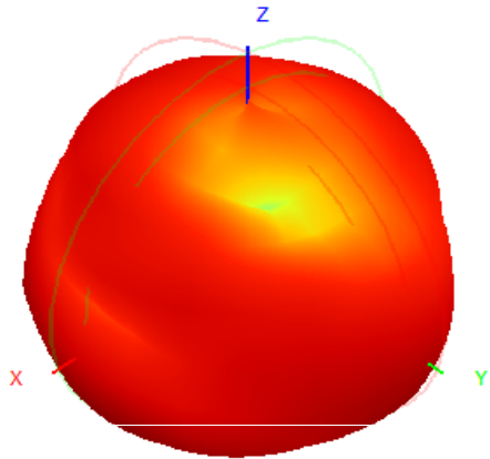
907.0MHz H+V, Eff: 2.1%
