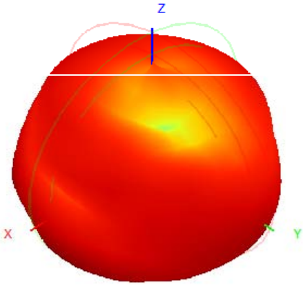
903.0MHz H+V, Eff: 1.9%
