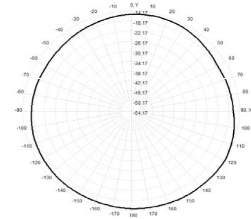
Total(H-XY), Max= -14.46dBi, CirD=3.61
