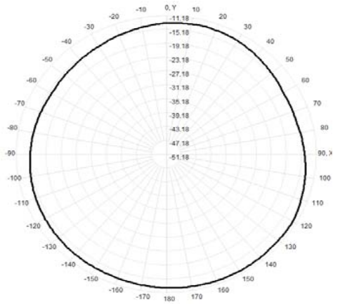
Total(H-XY), Max= -12.31dBi, CirD=3.74
