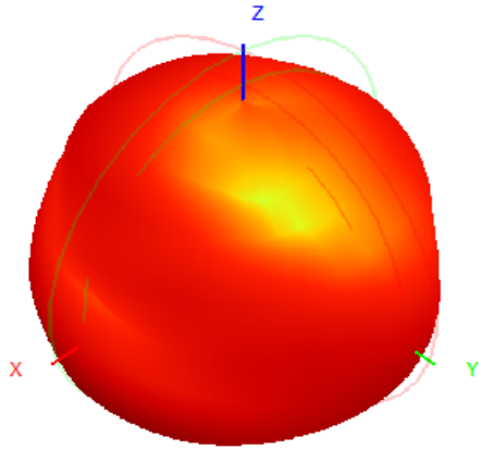
926.0MHz H+V, Eff: 3.7%
