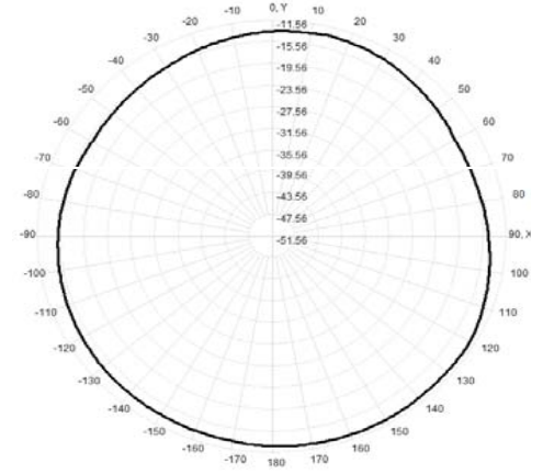
Total(H-XY), Max= -12.60dBi, CirD=3.67
