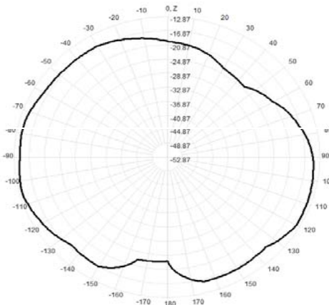
915.0MHz Total(E2-YZ), Max= -13.62dBi
