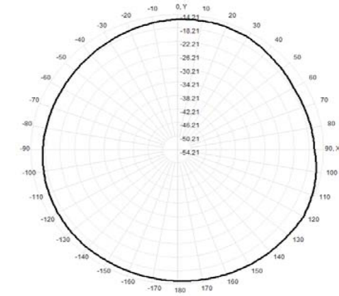
Total(H-XY), Max= -14.55dBi, CirD=3.60
