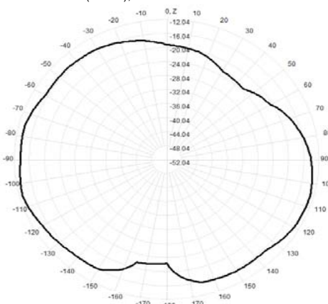
919.0MHz Total(E2-YZ), Max= -12.93dBi
