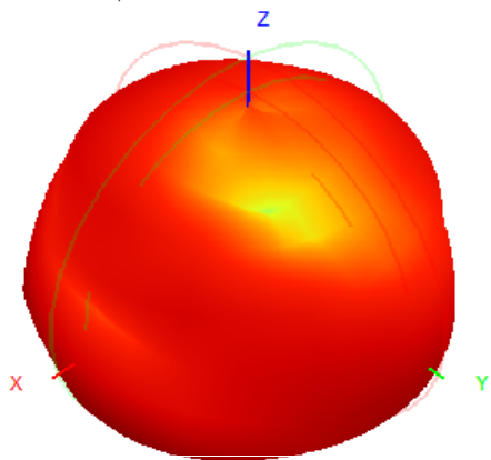
910.0MHz H+V, Eff: 2.2%
