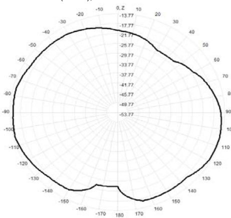
910.0MHz Total(E2-YZ), Max= -14.49dBi
