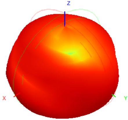
905.0MHz H+V, Eff: 2.0%
