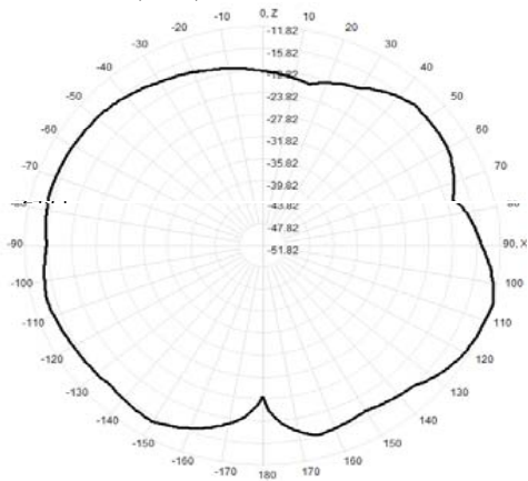
921.0MHz Total(E1-XZ), Max= -11.82dBi
