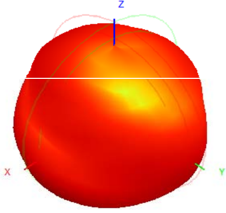
924.0MHz H+V, Eff: 3.4%
