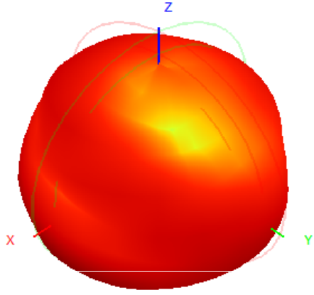
925.0MHz H+V, Eff: 3.5%
