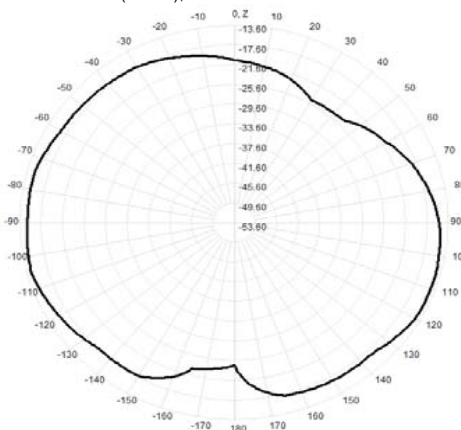
908.0MHz Total(E2-YZ), Max= -14.45dBi
