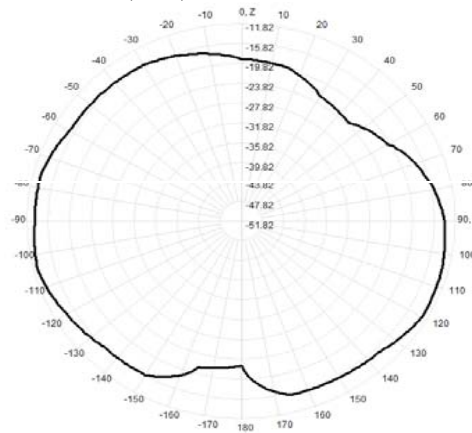
921.0MHz Total(E2-YZ), Max= -12.61dBi
