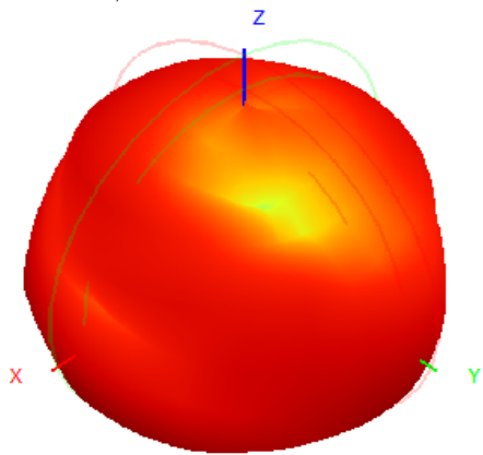
911.0MHz H+V, Eff: 2.2%
