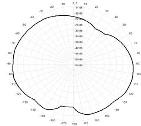
904.0MHz Total(E2-YZ), Max=-14.70dBi
