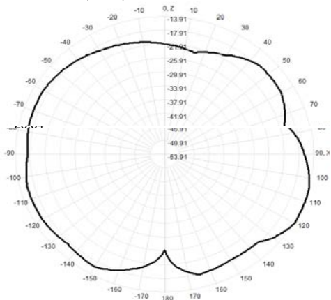
909.0MHz Total(E1-XZ), Max= -13.91dBi
