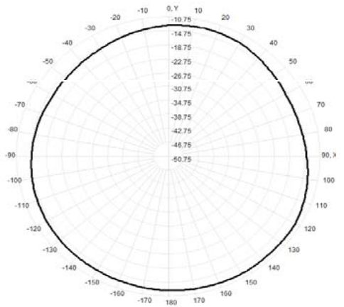
Total(H-XY), Max= -12.16dBi, CirD=3.71
