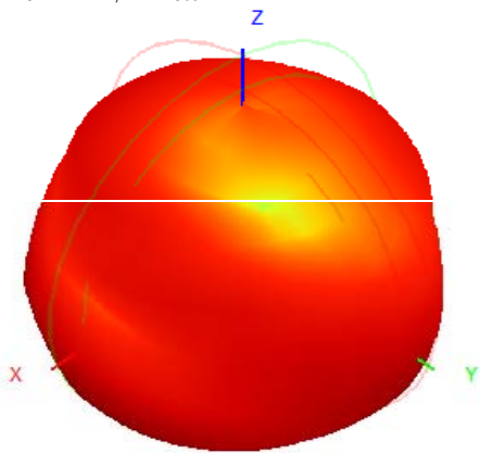
912.0MHz H+V, Eff: 2.3%
