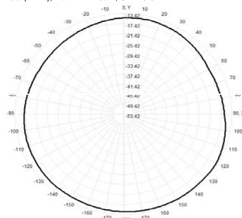
Total(H-XY), Max= -14.16dBi, CirD=3.60
