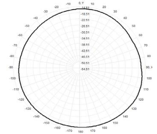
Total(H-XY), Max=-14.90dBi, CirD=3.52
