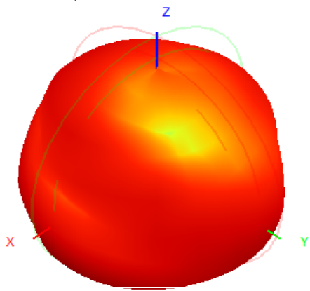
919.0MHz H+V, Eff: 2.9%
