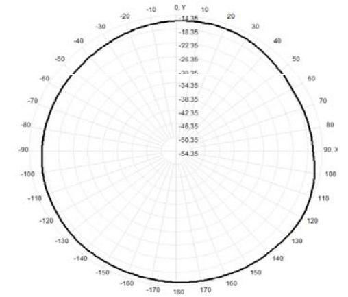
Total(H-XY), Max=-14.74dBi, CirD=3.55
