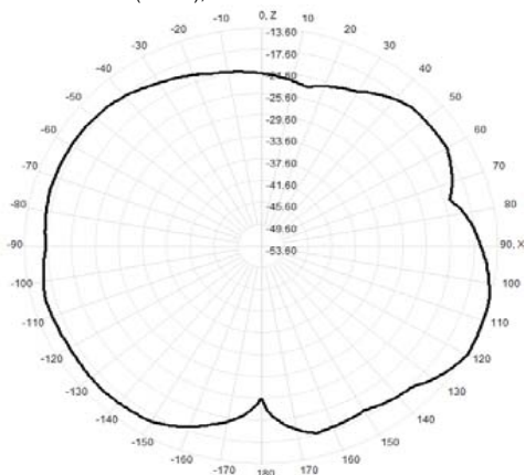
908.0MHz Total(E1-XZ), Max= -13.60dBi
