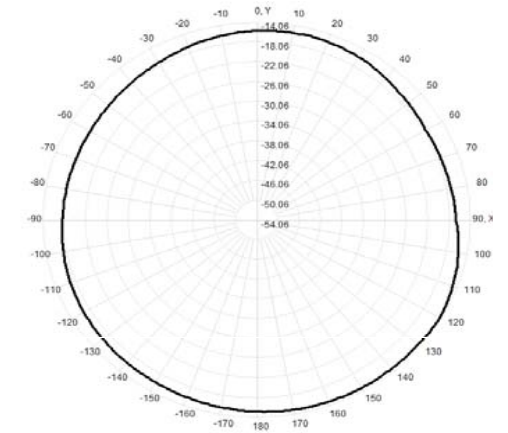
Total(H-XY), Max=-14.64dBi, CirD=3.52
