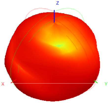
904.0MHz H+V, Eff: 1.9%
