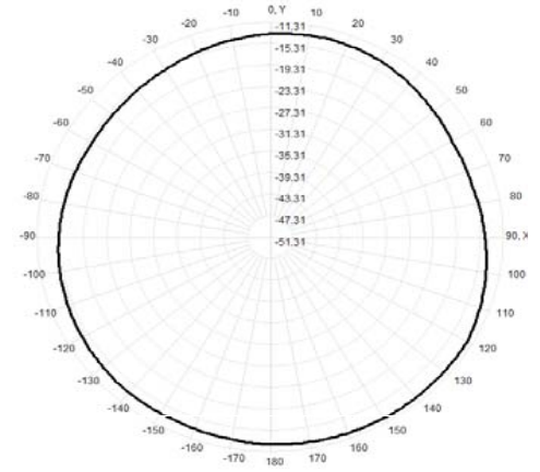
Total(H-XY), Max= -12.46dBi, CirD=3.65
