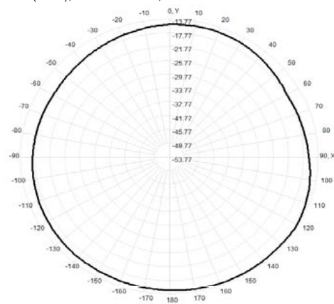
Total(H-XY), Max= -14.32dBi, CirD=3.61
