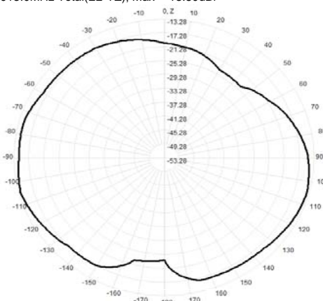
913.0MHz Total(E2-YZ), Max= -13.80dBi
