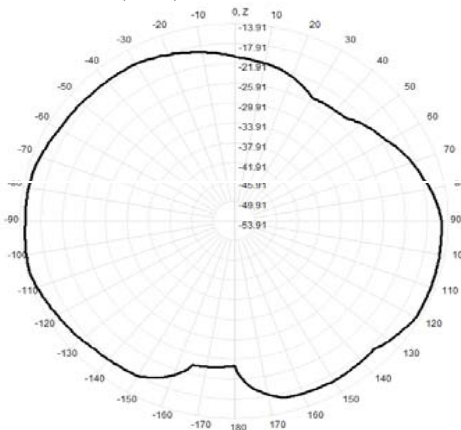
909.0MHz Total(E2-YZ), Max= -14.35dBi
