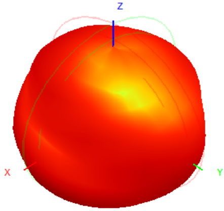
923.0MHz H+V, Eff: 3.3%
