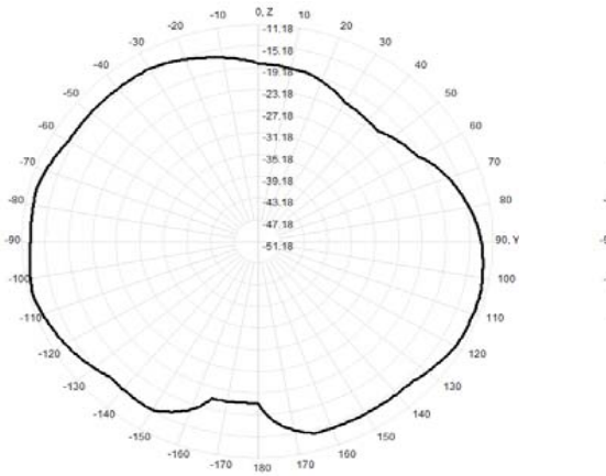
926.0MHz Total(E2-YZ), Max= -11.82dBi
