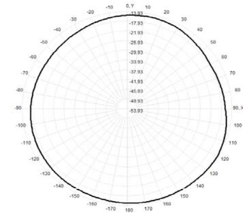
Total(H-XY), Max= -14.43dBi, CirD=3.49
