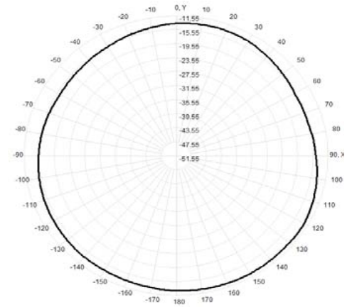
Total(H-XY), Max= -12.74dBi, CirD=3.64
