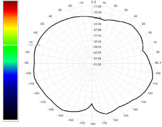
924.0MHz Total(E1-XZ), Max= -11.56dBi
