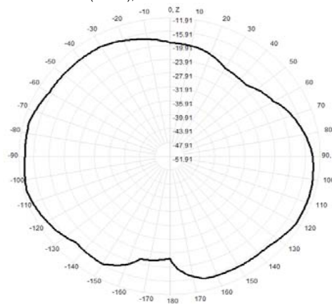
920.0MHz Total(E2-YZ), Max= -12.77dBi
