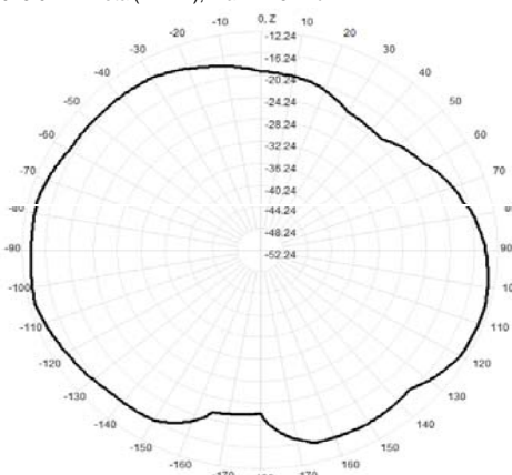
918.0MHz Total(E2-YZ), Max= -13.17dBi
