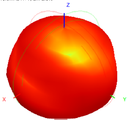
913.0MHz H+V, Eff: 2.3%
