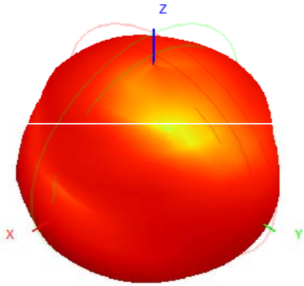
915.0MHz H+V, Eff: 2.5%
