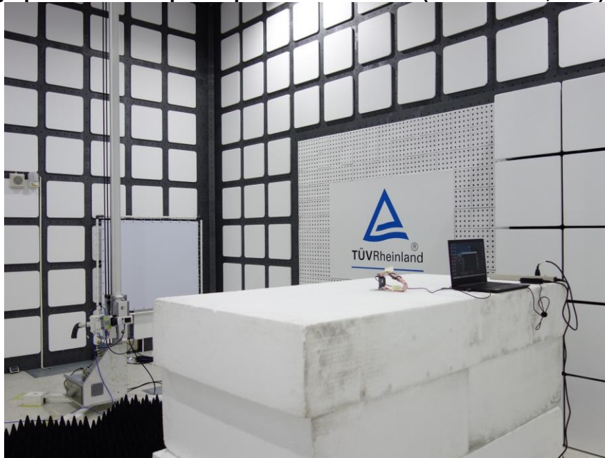
Photograph 5: Test Setup for Spurious Emissions (Back View 3, RSE)
