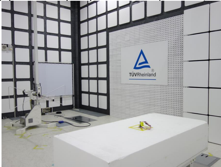
Photograph 10: Test Setup for Spurious Emissions (Back View 3, ERP/EIRP)
