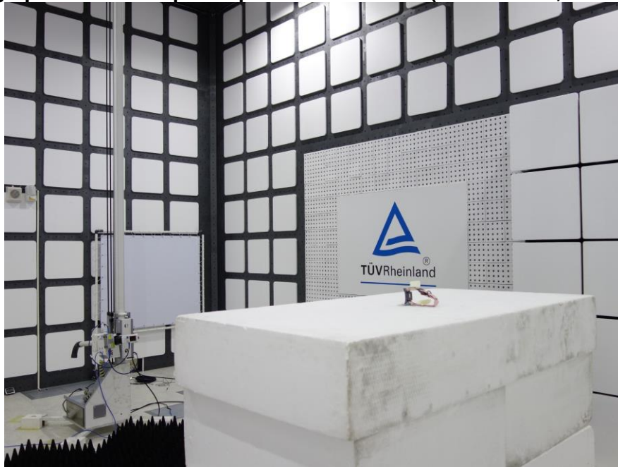
Photograph 9: Test Setup for Spurious Emissions (Back View 2, ERP/EIRP)
