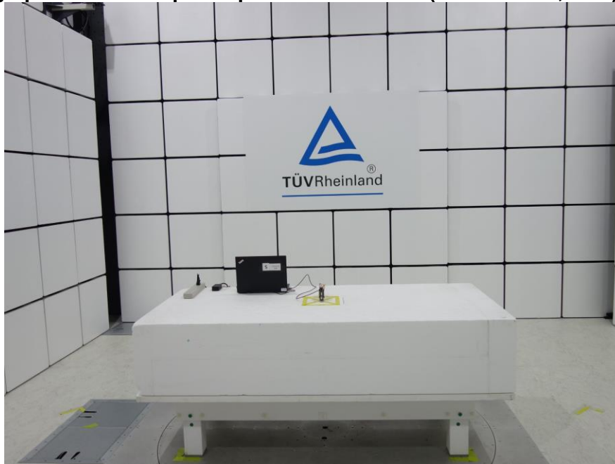
Photograph 2: Test Setup for Spurious Emissions (Front View 2, RSE)
