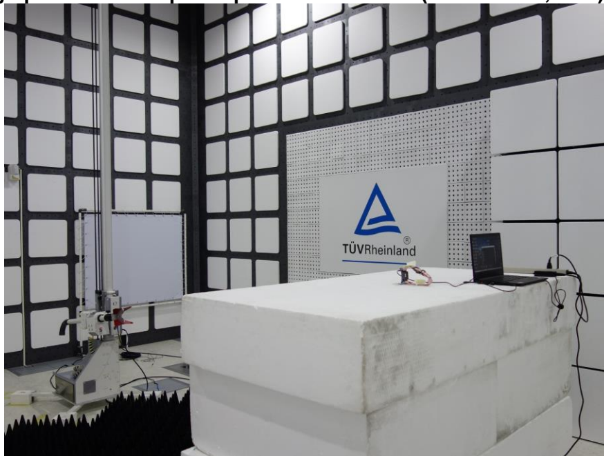
Photograph 4: Test Setup for Spurious Emissions (Back View 2, RSE)
