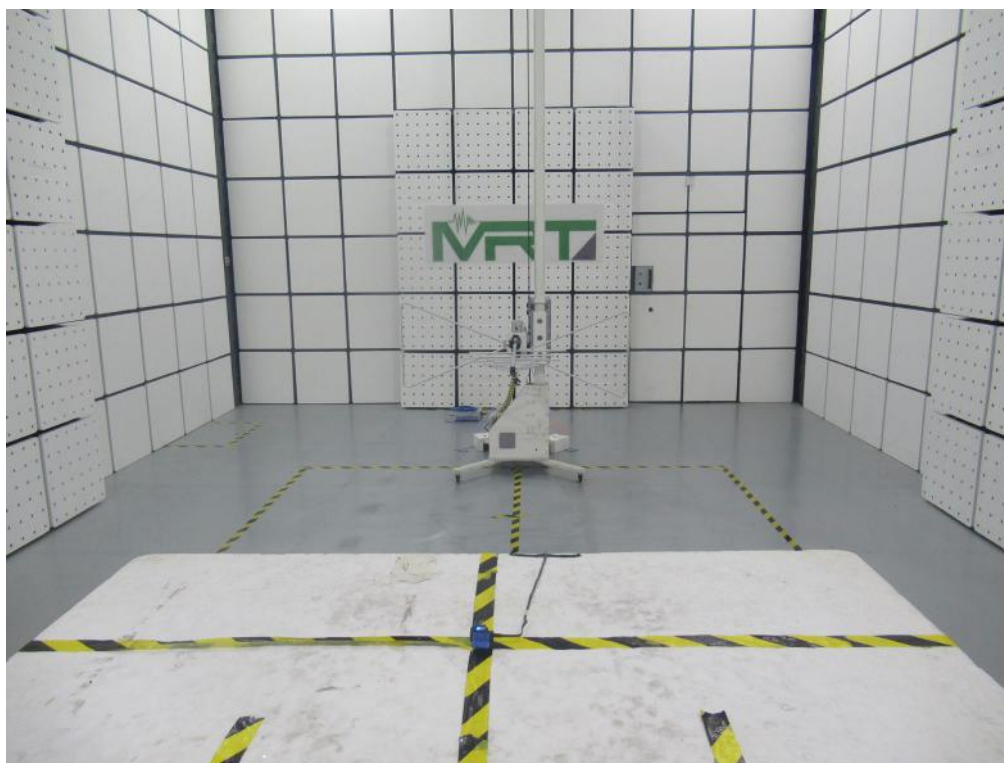
Description: Radiated Spurious Emission Test Setup for Above 1GHz
