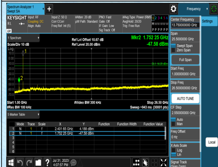
2.4G_TX-Ant1-2402-1000~26500
