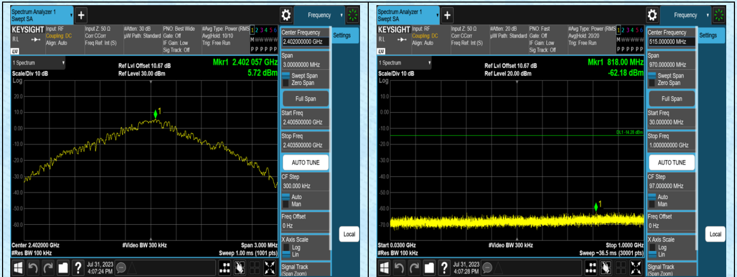
2.4G_TX-Ant1-2402-0~Reference
