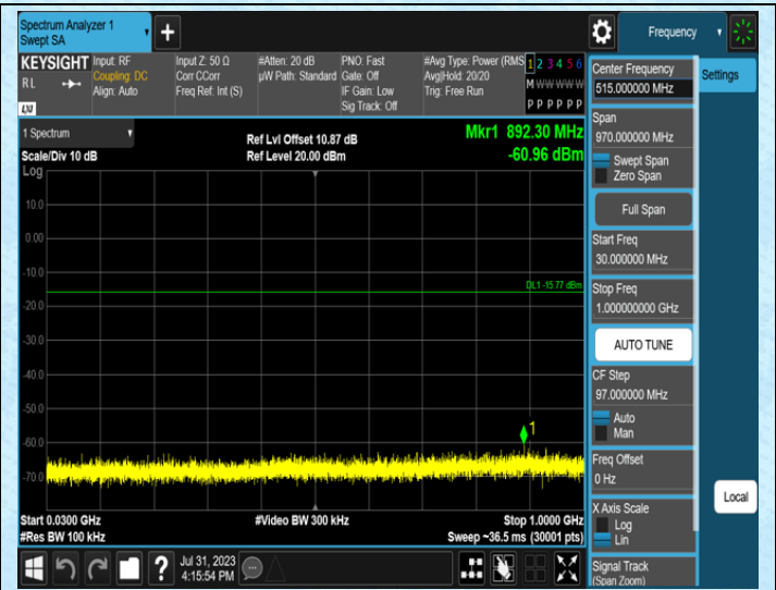
2.4G_TX-Ant1-2480-30~1000
