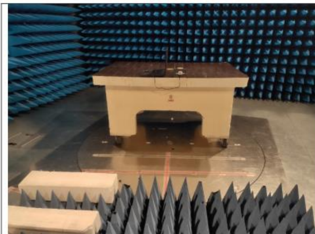
Test setup in Operating mode 1
