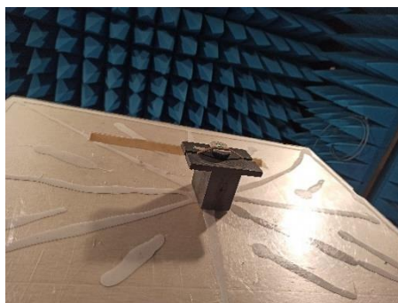
Setup in Anechoic room (XY axes)
