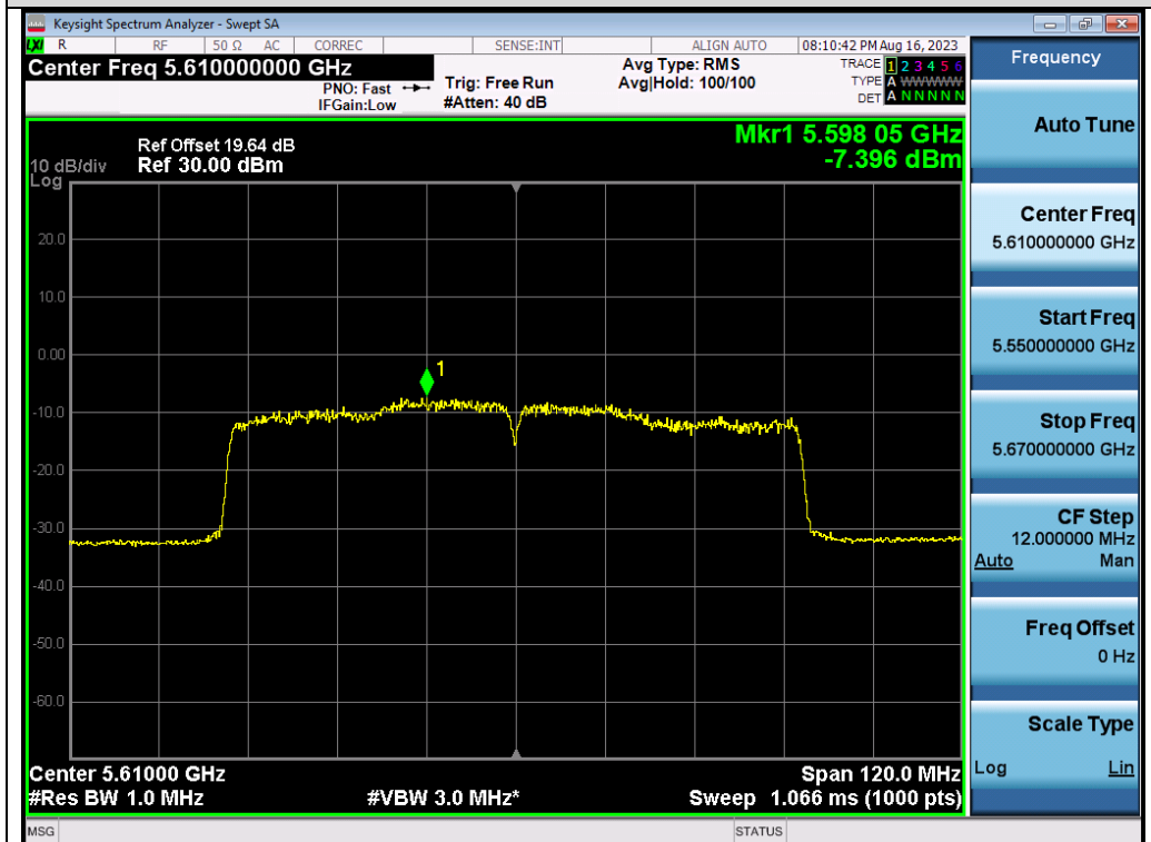
Test_Graph_802.11ac80_ANT2_5610_MCS9_PSD
