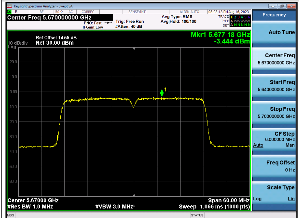
Test_Graph_802.11ac40_ANT2_5670_MCS9_PSD
