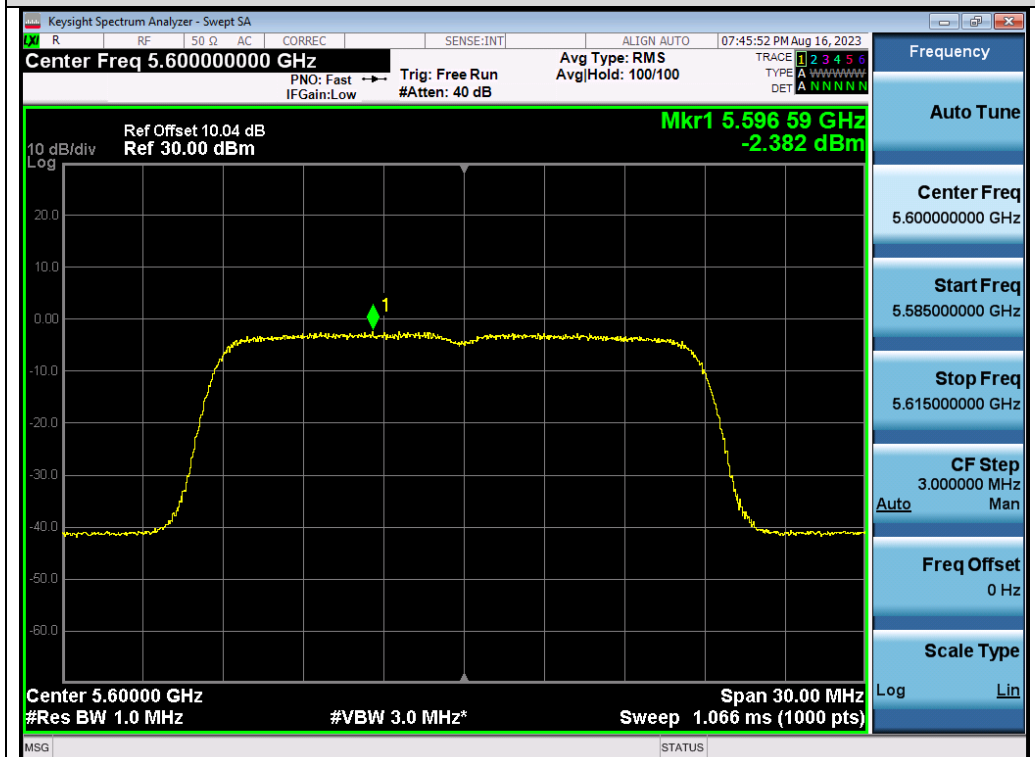
Test_Graph_802.11n20_ANT2_5600_MCS0_PSD
