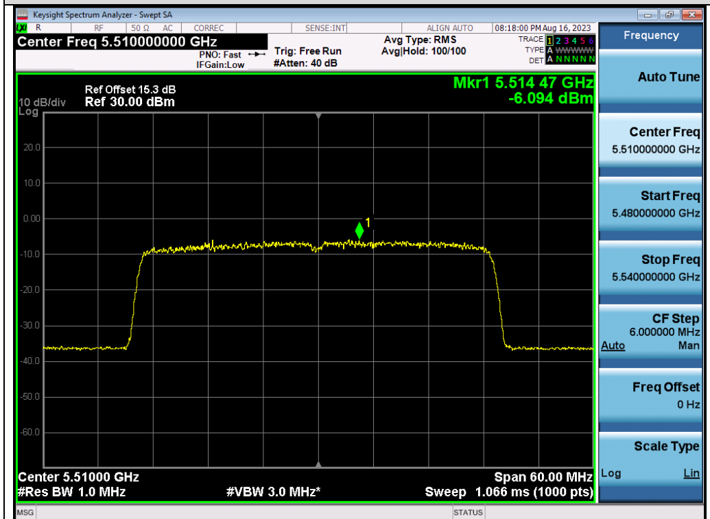
Test_Graph_802.11ax40_ANT2_5510_MCS9_PSD
