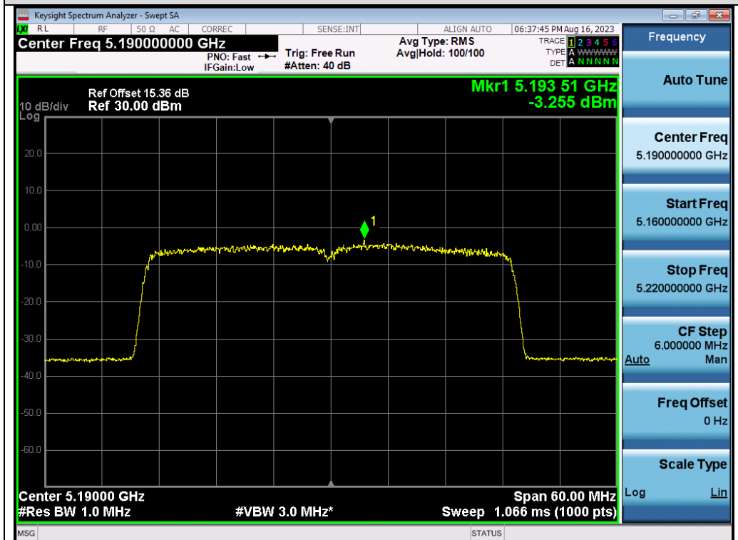
Test_Graph_802.11ax40_ANT2_5190_MCS9_PSD
