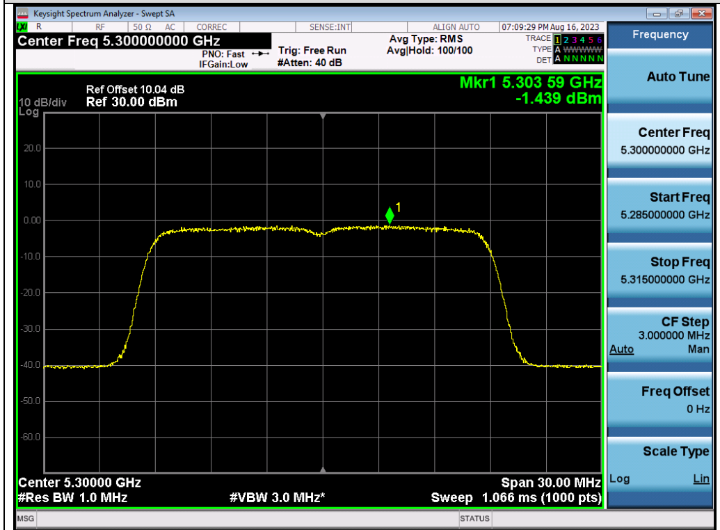
Test_Graph_802.11ac20_ANT2_5300_MCS0_PSD
