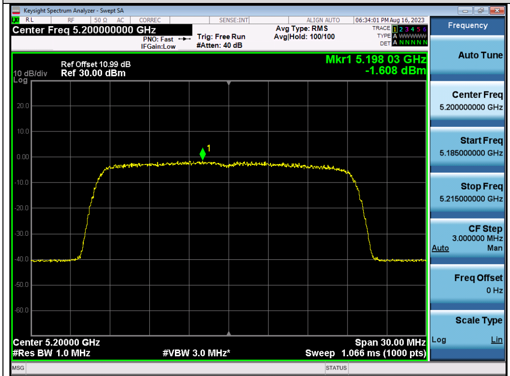
Test_Graph_802.11ax20_ANT2_5200_MCS0_PSD
