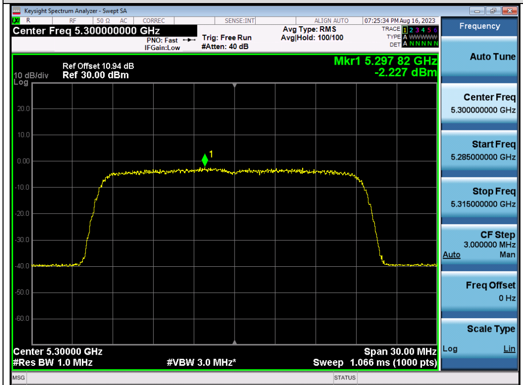
Test_Graph_802.11ax20_ANT2_5300_MCS0_PSD
