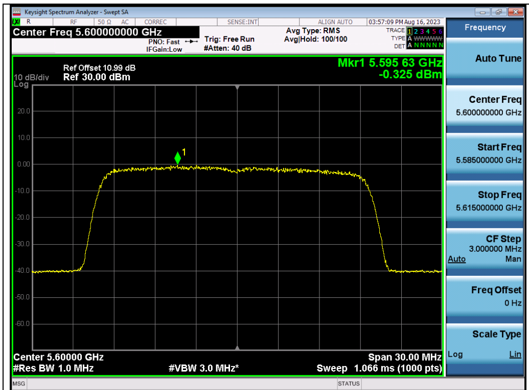
Test_Graph_802.11ax20_ANT1_5600_MCS0_PSD
