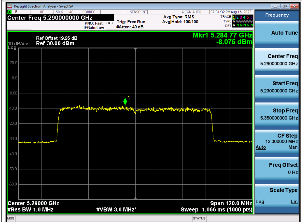
Test_Graph_802.11ax80_ANT2_5290_MCS0_PSD
