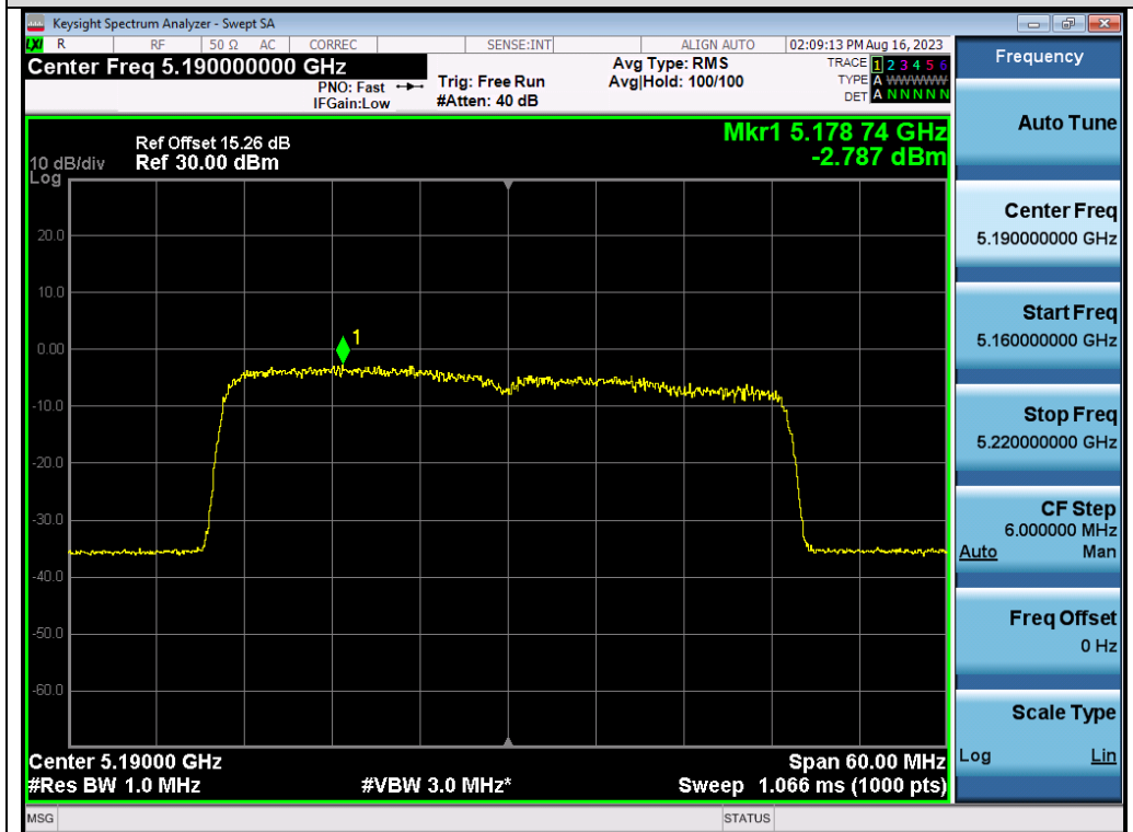
Test_Graph_802.11ax40_ANT1_5190_MCS9_PSD
