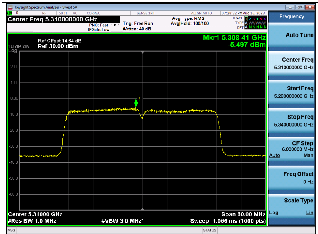
Test_Graph_802.11ax40_ANT2_5310_MCS0_PSD
