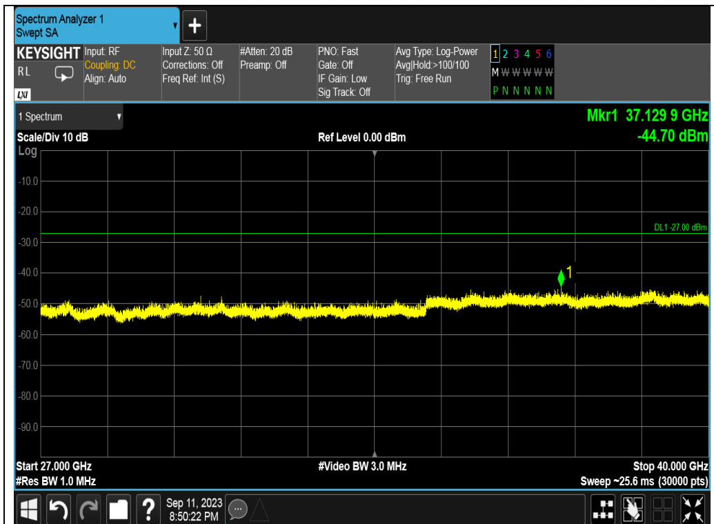
Test_Graph_802.11ax80_ANT1_5610_MCS9_Frequency Band 5
