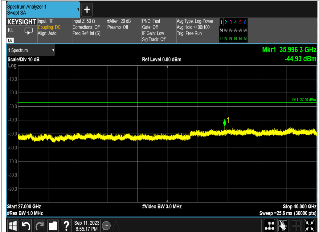
Test_Graph_802.11ac80_ANT2_5610_MCS9_Frequency Band 5
