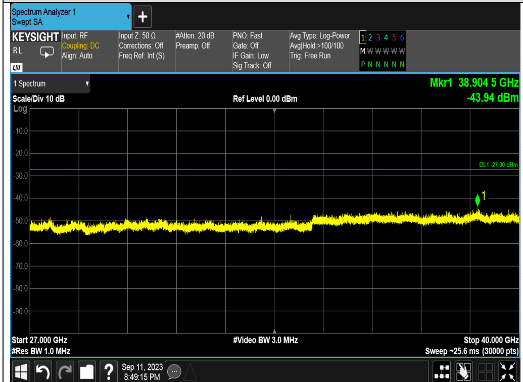
Test_Graph_802.11ax80_ANT1_5530_MCS9_Frequency Band 5
