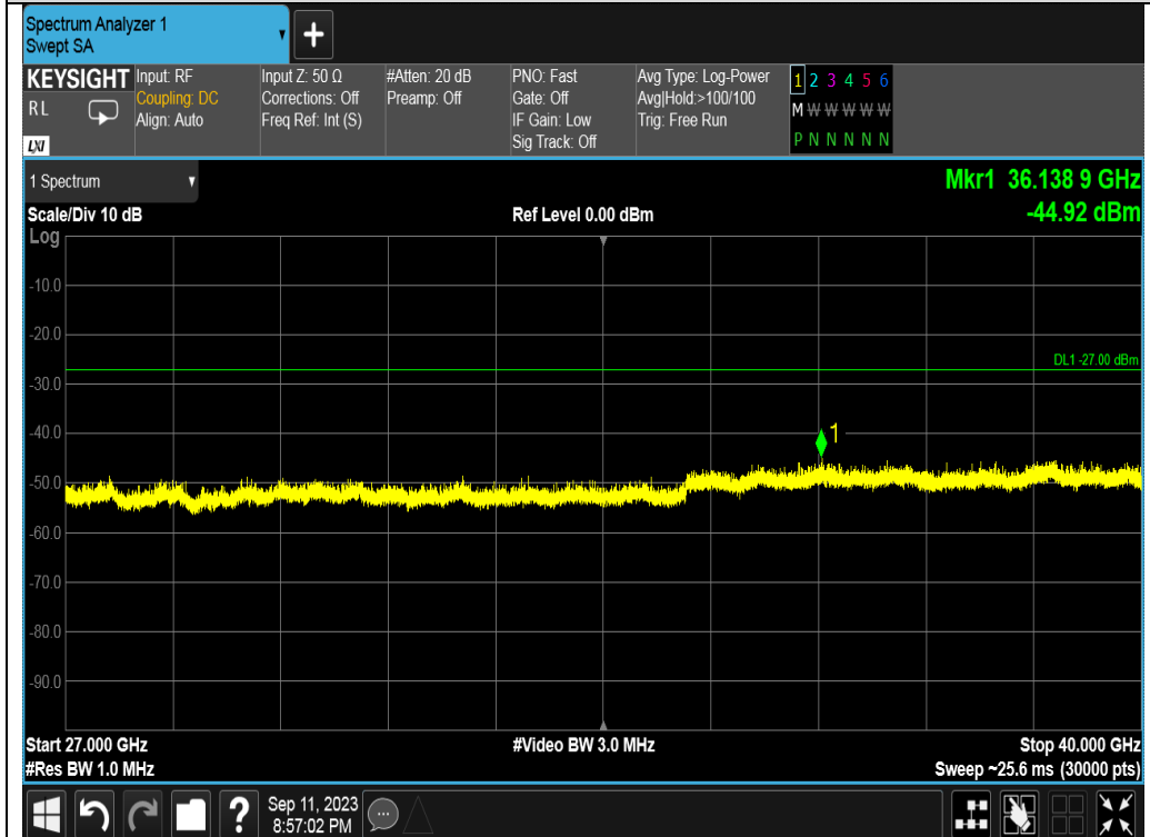
Test_Graph_802.11ax80_ANT2_5610_MCS9_Frequency Band 5
