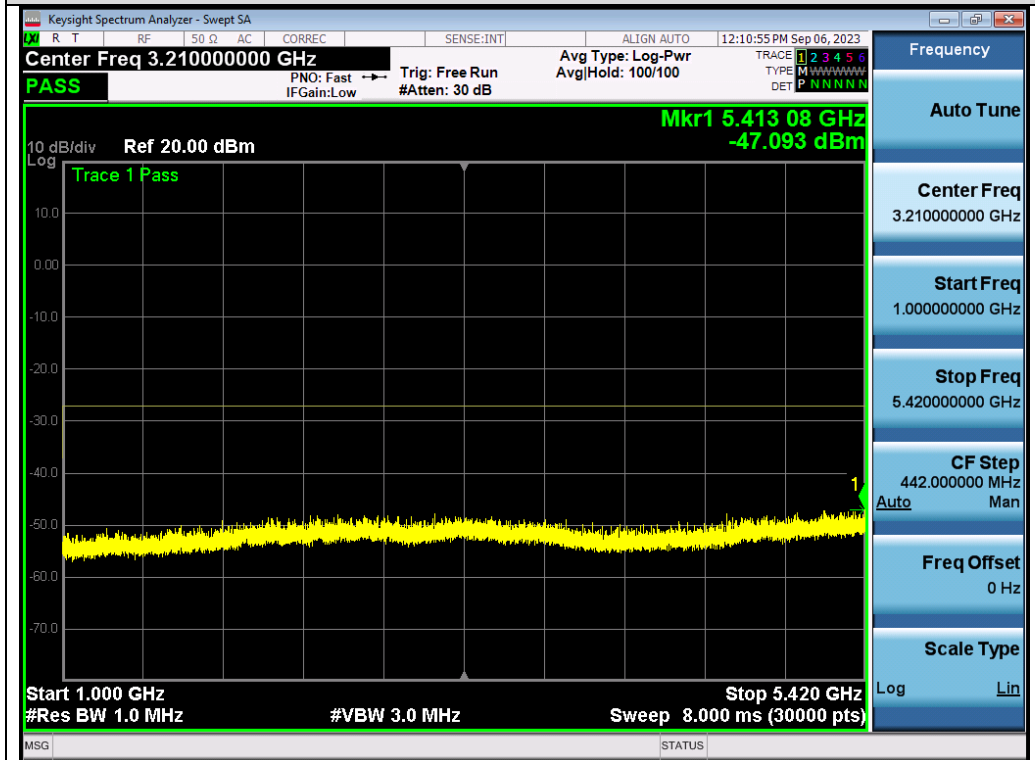
Test_Graph_802.11ax80_ANT1_5610_MCS9_Frequency Band 2
