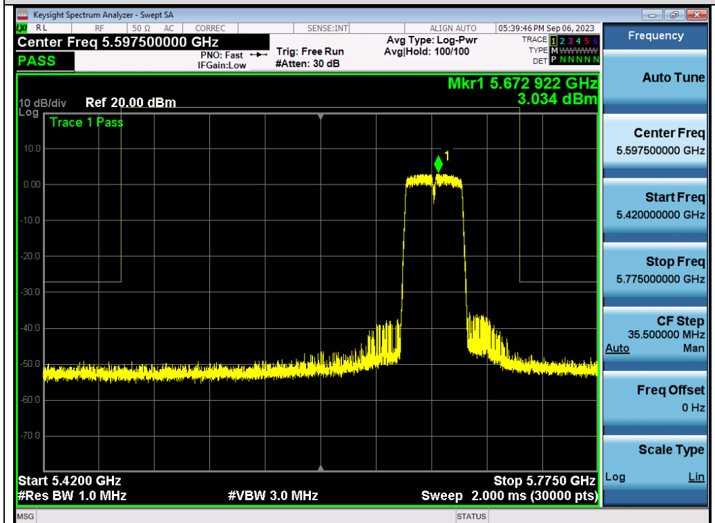
Test_Graph_802.11n40_ANT2_5670_MCS0_Frequency Band 3
