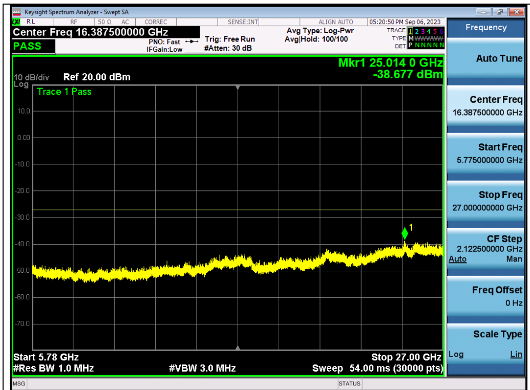
Test_Graph_802.11a_ANT2_5500_6Mbps_Frequency Band 4
