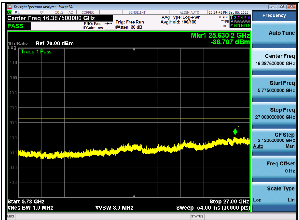
Test_Graph_802.11n40_ANT2_5510_MCS0_Frequency Band 4
