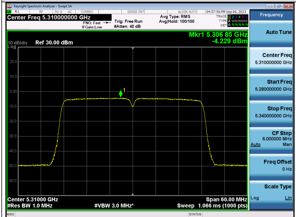
Test_Graph_802.11n40_ANT2_5310_MCS0_PSD
