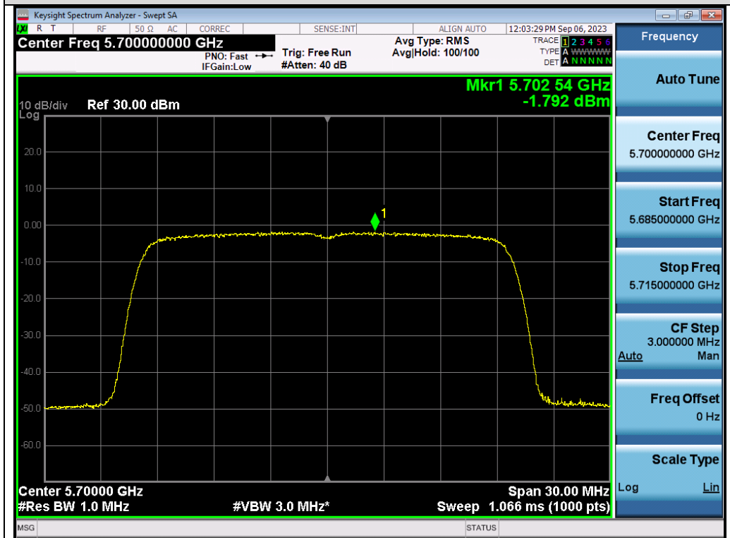
Test_Graph_802.11ax20_ANT1_5700_MCS9_OBW
