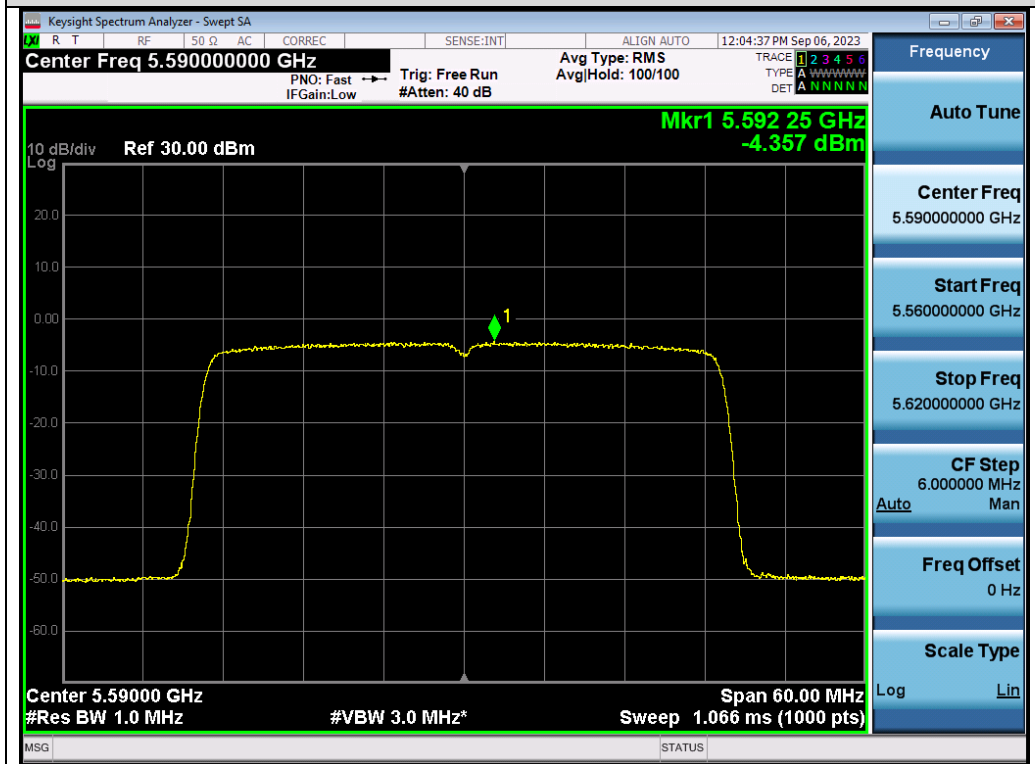
Test_Graph_802.11ax40_ANT1_5590_MCS9_OBW
