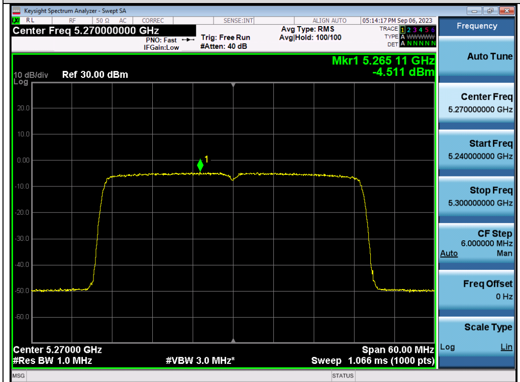
Test_Graph_802.11ax40_ANT2_5270_MCS0_PSD
