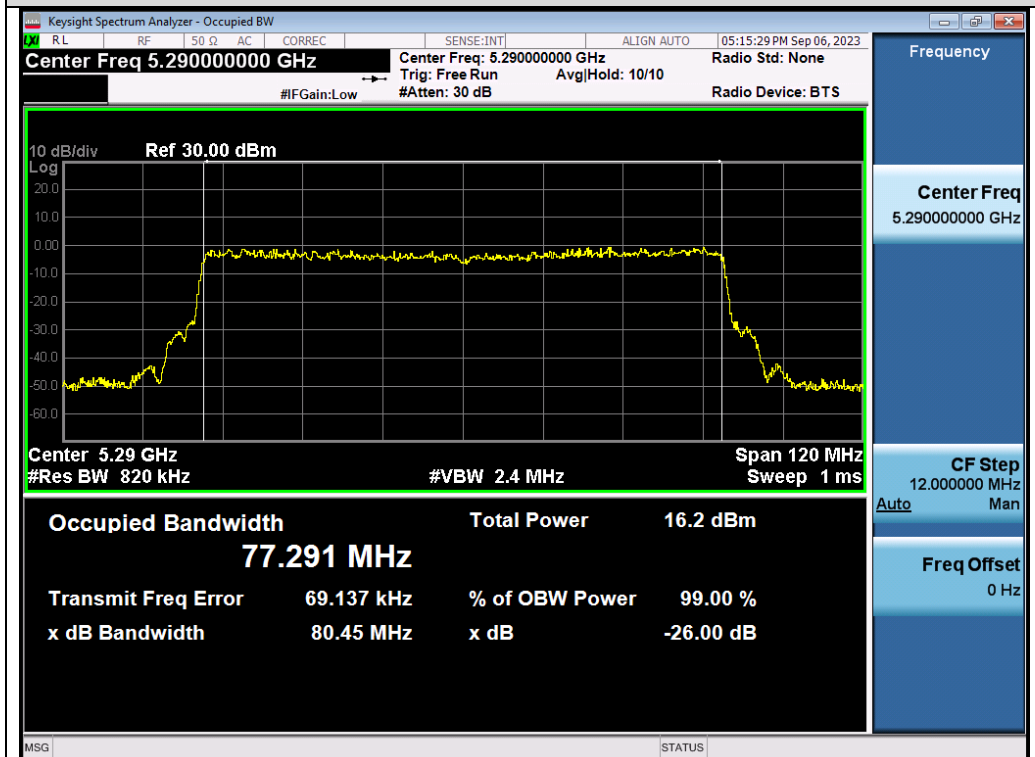
Test_Graph_802.11ax80_ANT2_5290_MCS0_OBW
