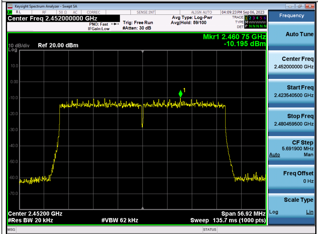
Test_Graph_802.11ax40_ANT2_2452_MCS0_PSD
