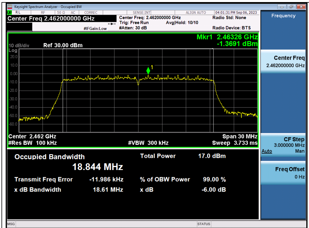
Test_Graph_802.11ax20_ANT2_2462_MCS0_DTSBW
