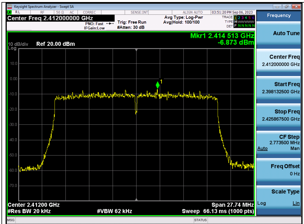
Test_Graph_802.11ax20_ANT2_2412_MCS0_PSD
