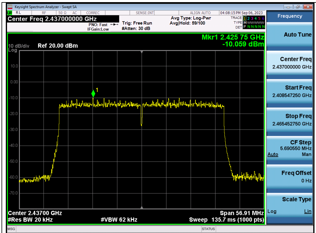
Test_Graph_802.11ax40_ANT2_2437_MCS0_PSD
