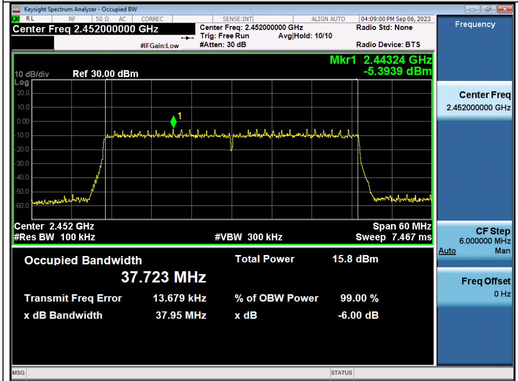
Test_Graph_802.11ax40_ANT2_2452_MCS0_DTSBW
