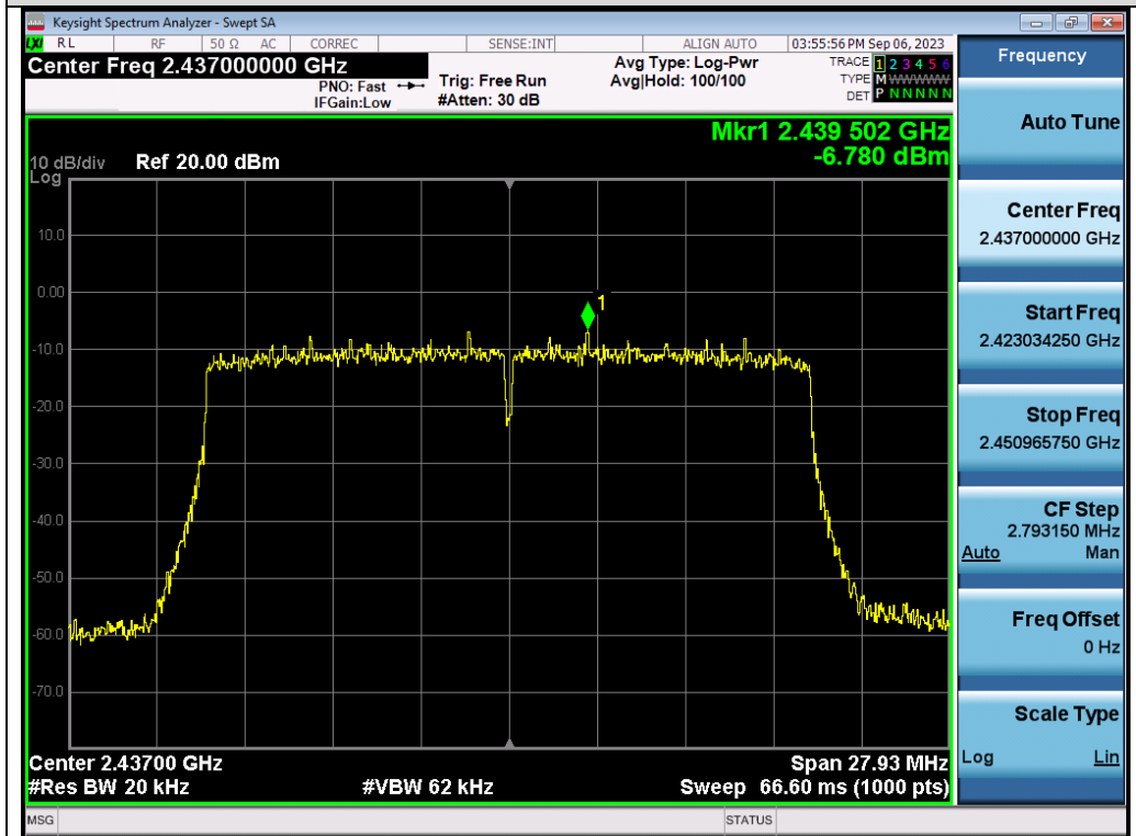
Test_Graph_802.11ax20_ANT2_2437_MCS0_PSD
