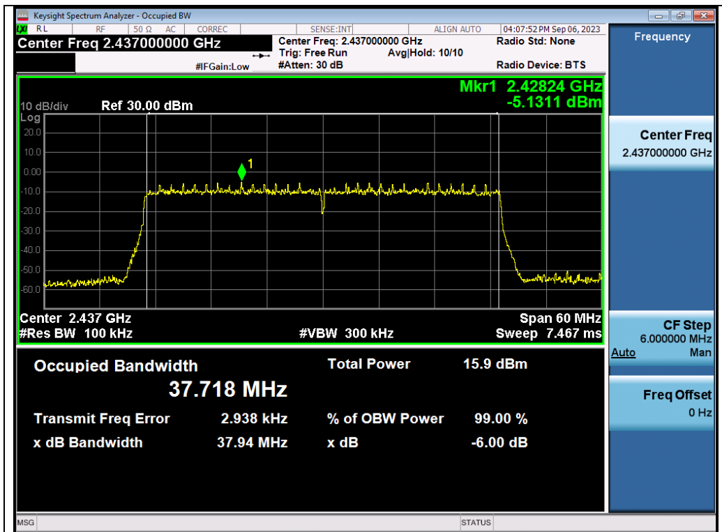
Test_Graph_802.11ax40_ANT2_2437_MCS0_DTSBW
