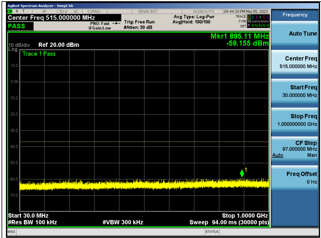
Test_Graph_802.11a_ANT1_5260_6Mbps_Frequency Band 1
