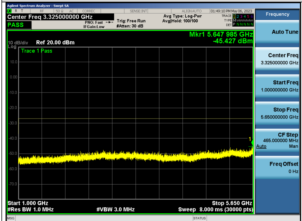
Test_Graph_802.11ac80_ANT1_5775_MCS9_Frequency Band2
