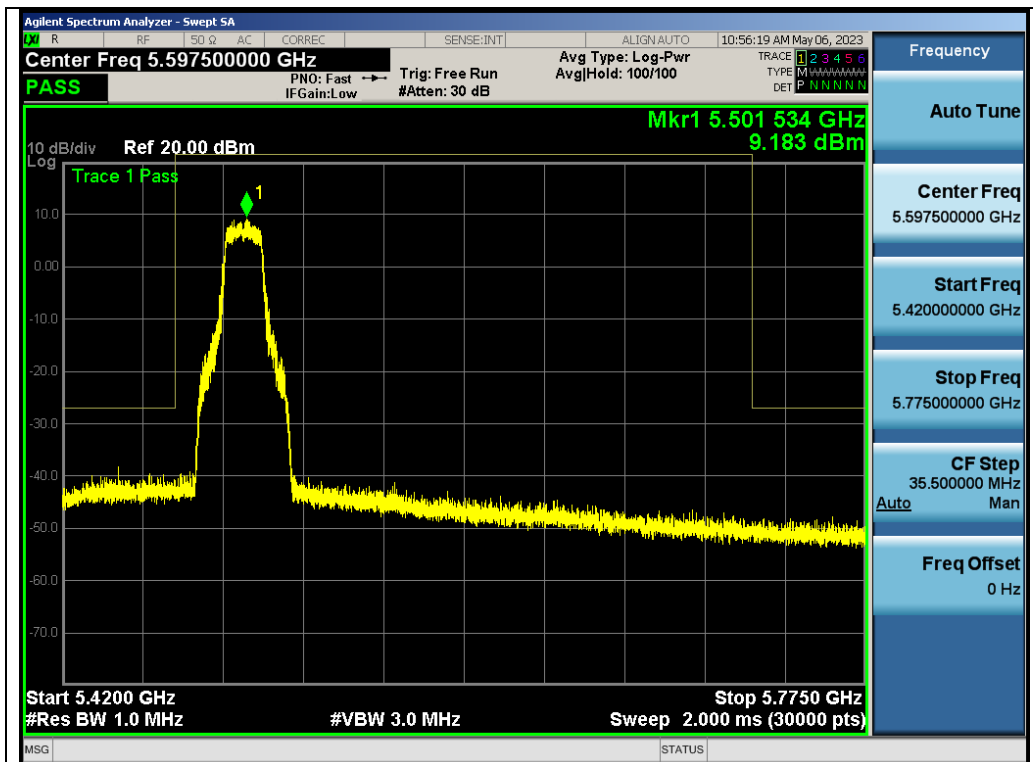
Test_Graph_802.11a_ANT2_5500_6Mbps_Frequency Band 3
