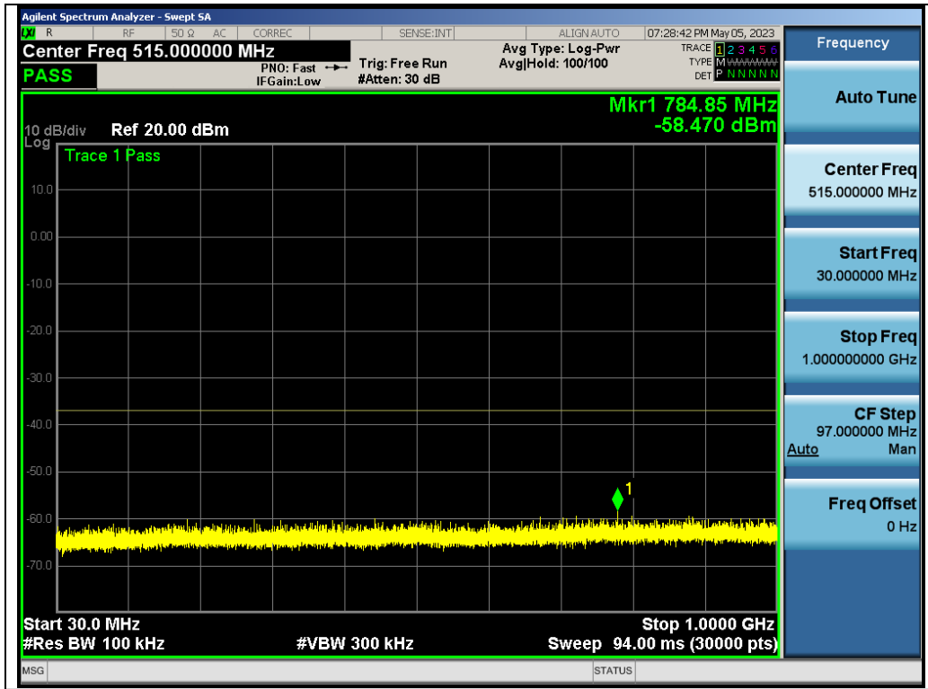
Test_Graph_802.11a_ANT2_5260_6Mbps_Frequency Band 1
