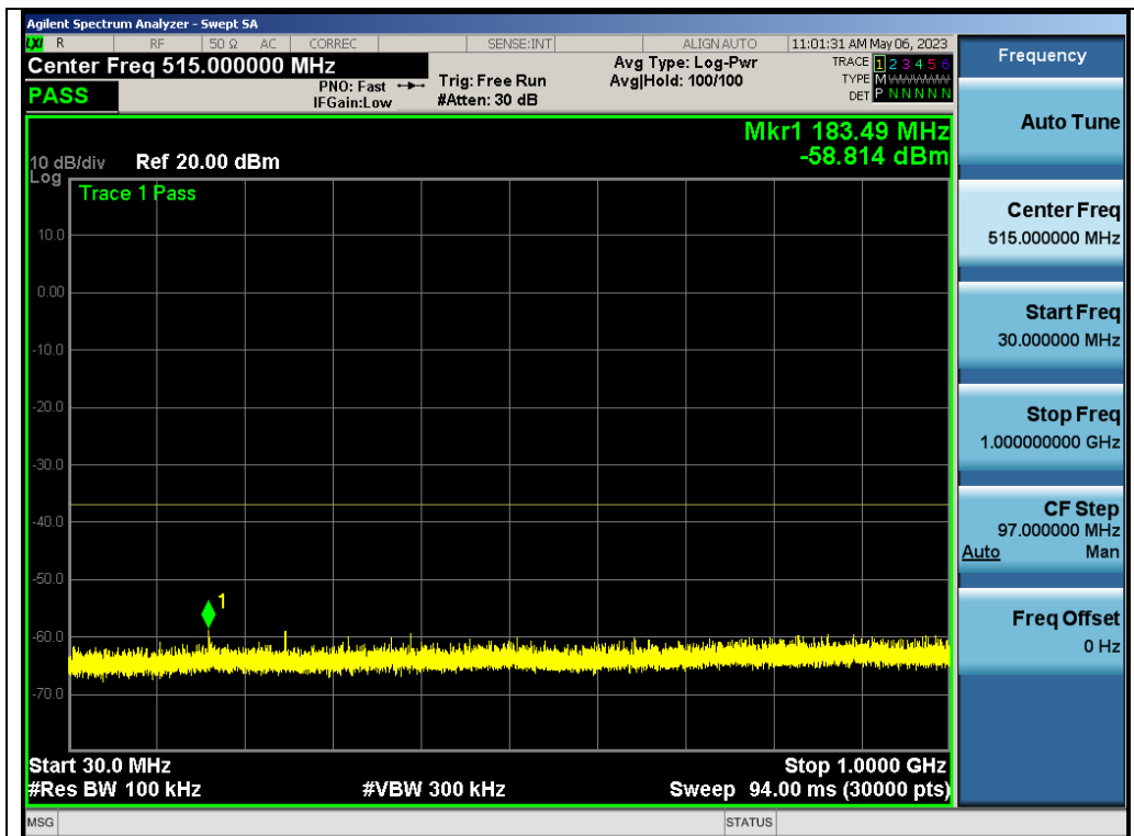
Test_Graph_802.11a_ANT2_5700_6Mbps_Frequency Band 1
