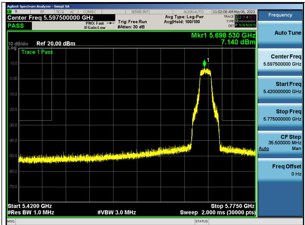
Test_Graph_802.11a_ANT2_5700_6Mbps_Frequency Band 3
