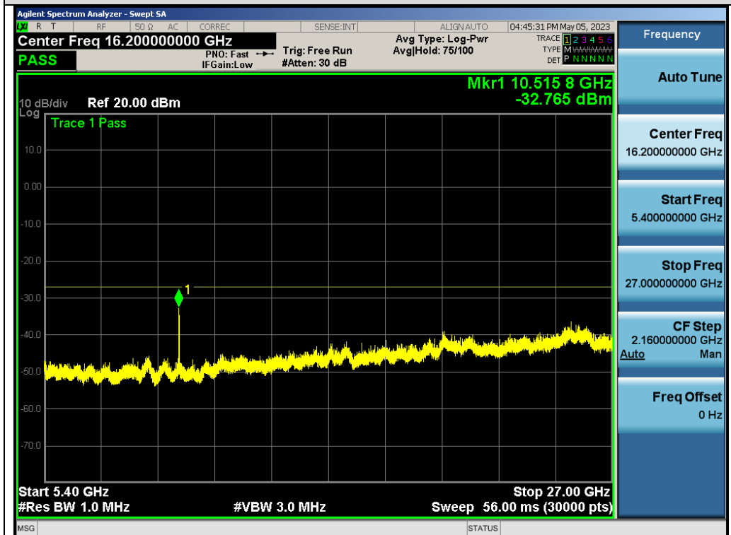
Test_Graph_802.11a_ANT1_5260_6Mbps_Frequency Band 4
