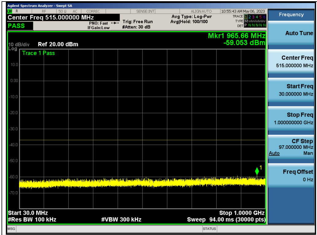
Test_Graph_802.11a_ANT2_5500_6Mbps_Frequency Band 1
