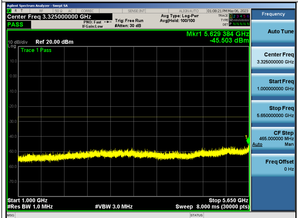
Test_Graph_802.11a_ANT1_5825_6Mbps_Frequency Band2
