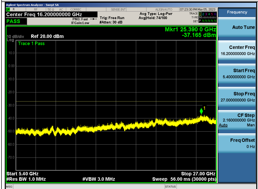
Test_Graph_802.11ac80_ANT2_5210_MCS0_Frequency Band 4
