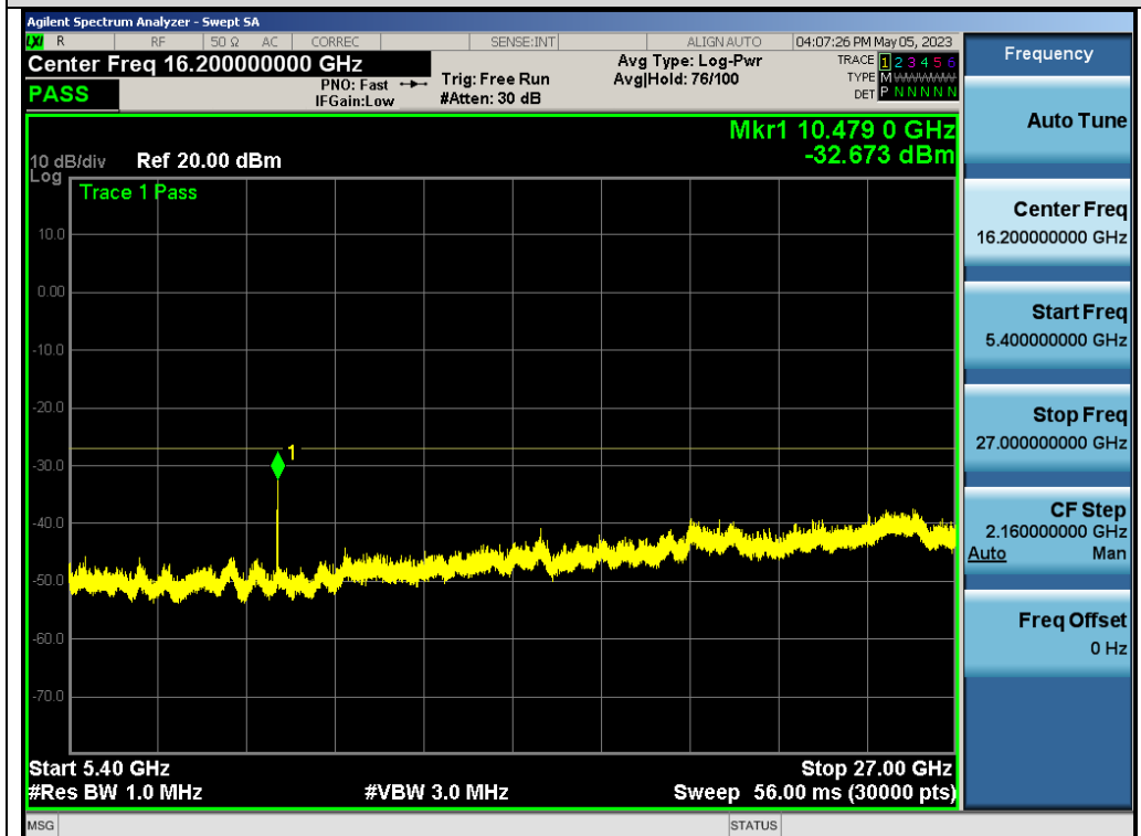
Test_Graph_802.11a_ANT1_5240_6Mbps_Frequency Band 4
