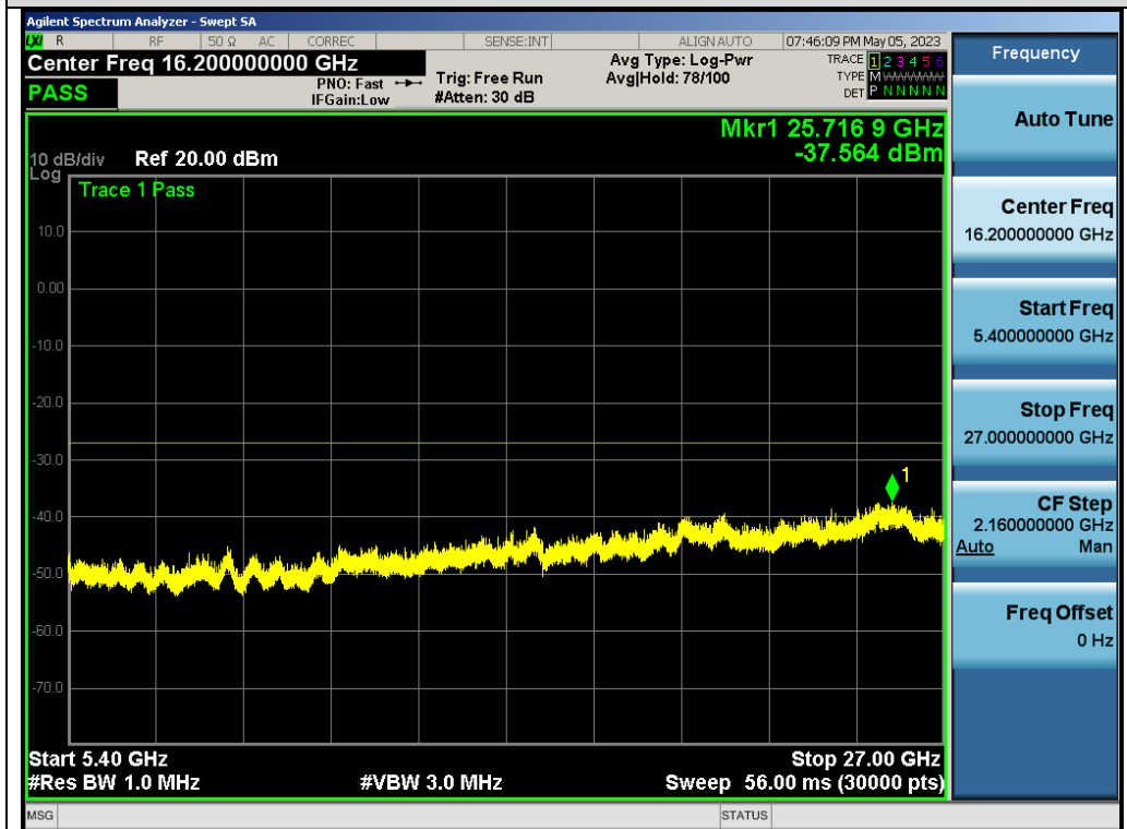
Test_Graph_802.11n40_ANT2_5310_MCS0_Frequency Band 4
