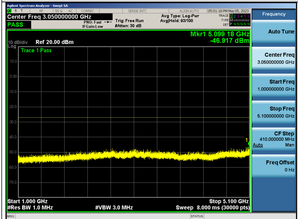
Test_Graph_802.11n40_ANT1_5310_MCS0_Frequency Band 2
