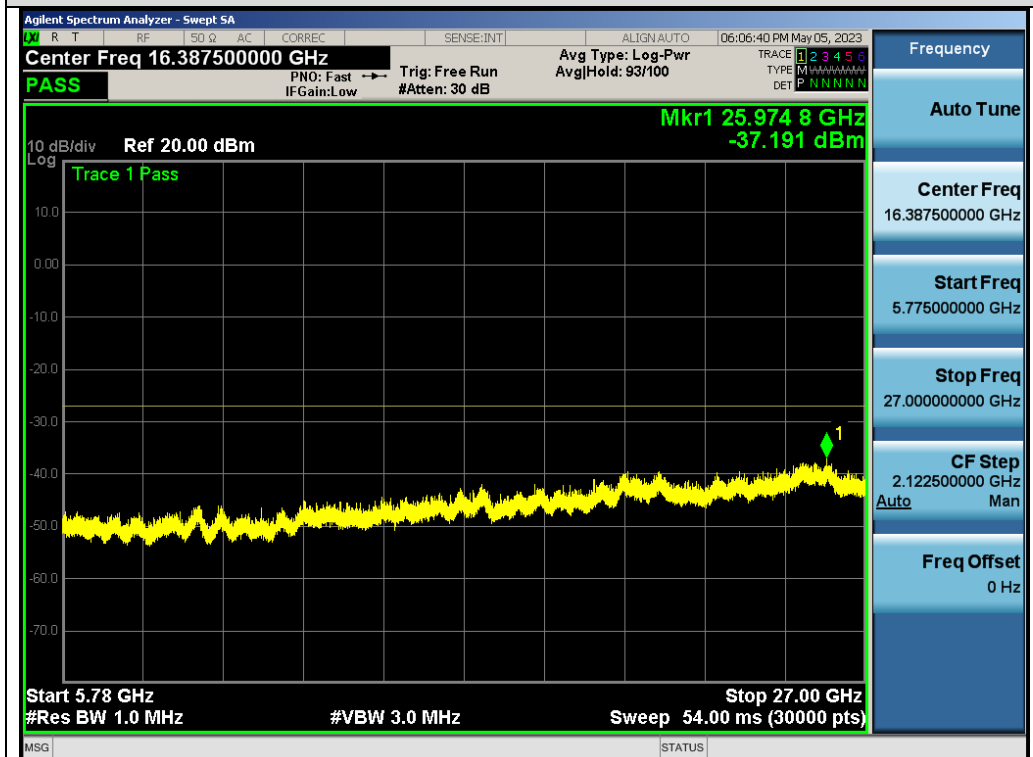
Test_Graph_802.11ac80_ANT1_5530_MCS0_Frequency Band 4
