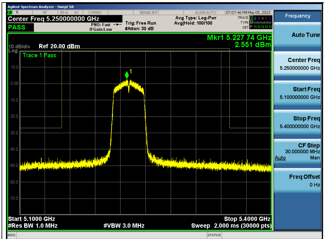
Test_Graph_802.11n40_ANT2_5230_MCS0_Frequency Band 3
