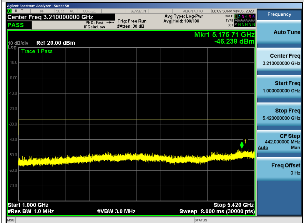
Test_Graph_802.11ac80_ANT1_5610_MCS0_Frequency Band 2
