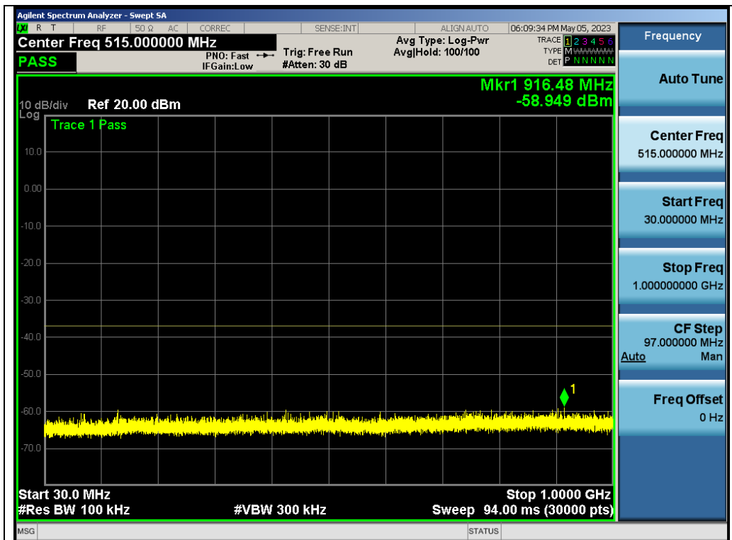
Test_Graph_802.11ac80_ANT1_5610_MCS0_Frequency Band 1
