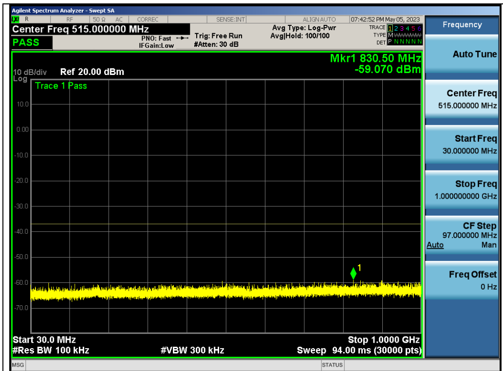
Test_Graph_802.11n40_ANT2_5270_MCS0_Frequency Band 1
