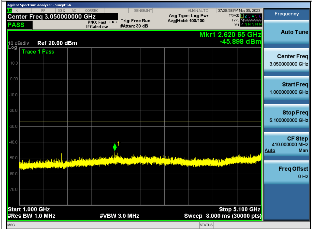
Test_Graph_802.11a_ANT2_5260_6Mbps_Frequency Band 2
