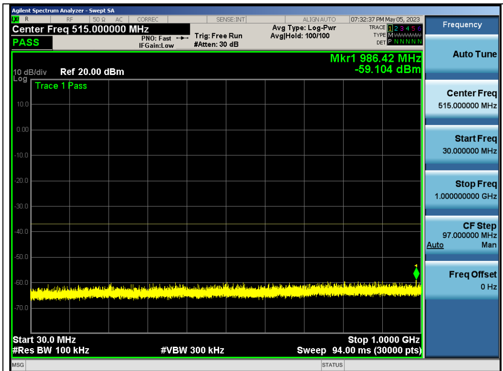
Test_Graph_802.11a_ANT2_5320_6Mbps_Frequency Band 1
