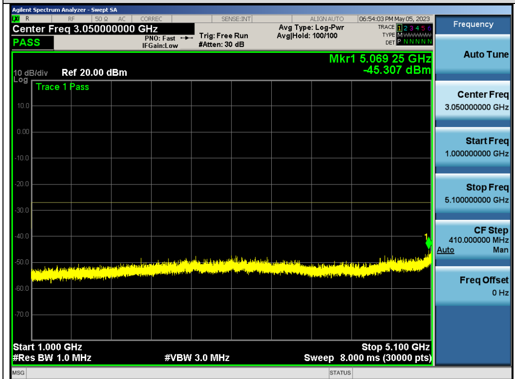
Test_Graph_802.11a_ANT2_5240_6Mbps_Frequency Band 2
