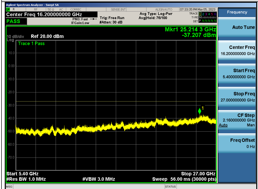
Test_Graph_802.11a_ANT2_5320_6Mbps_Frequency Band 4
