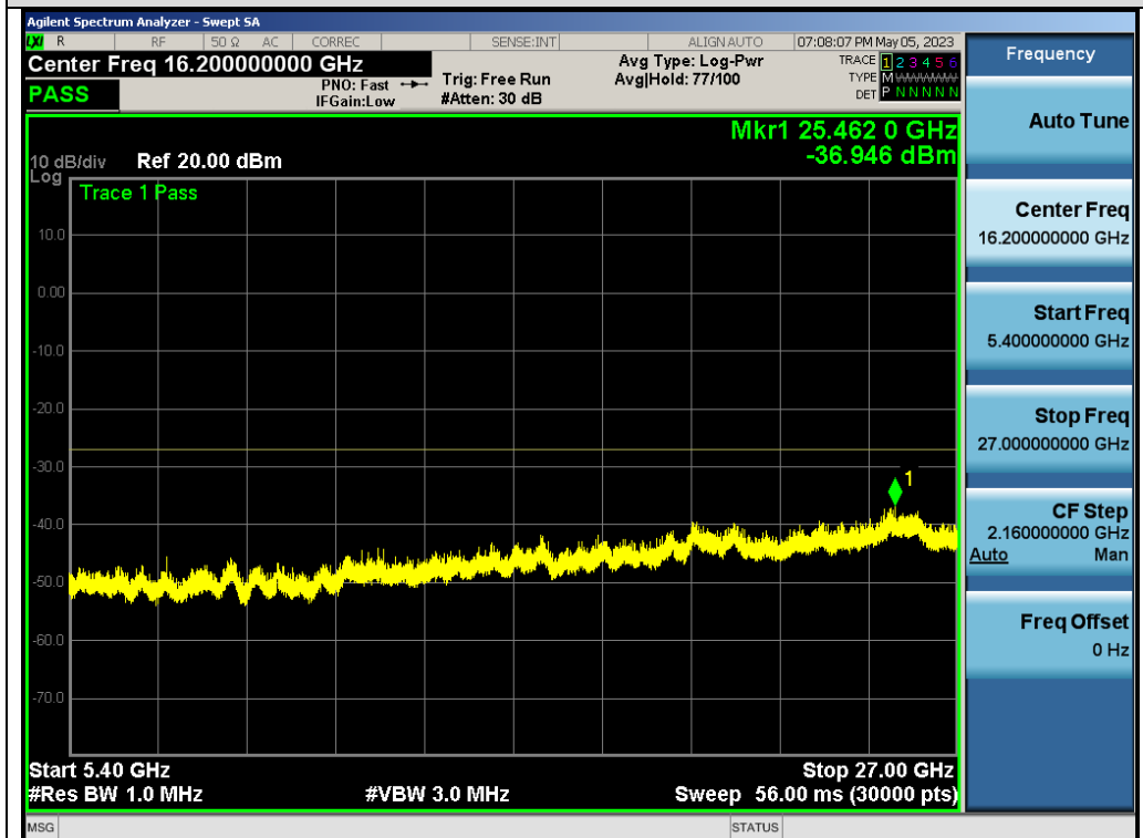
Test_Graph_802.11n40_ANT2_5230_MCS0_Frequency Band 4
