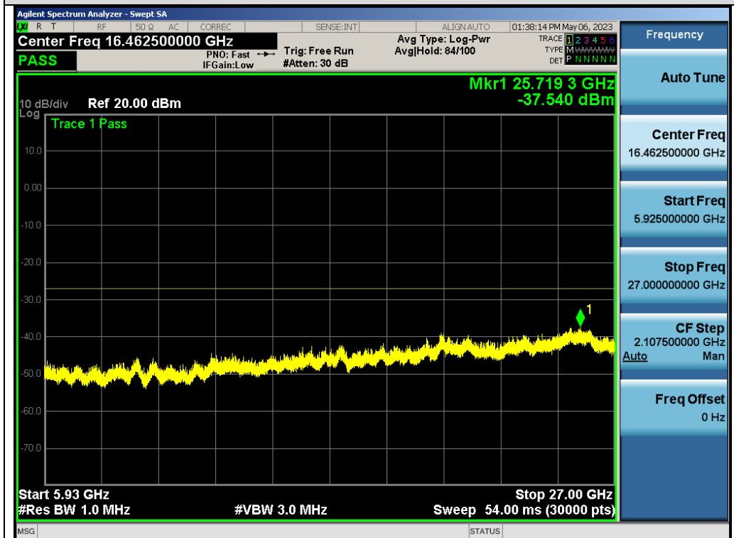
Test_Graph_802.11n40_ANT1_5795_MCS0_Frequency Band4
