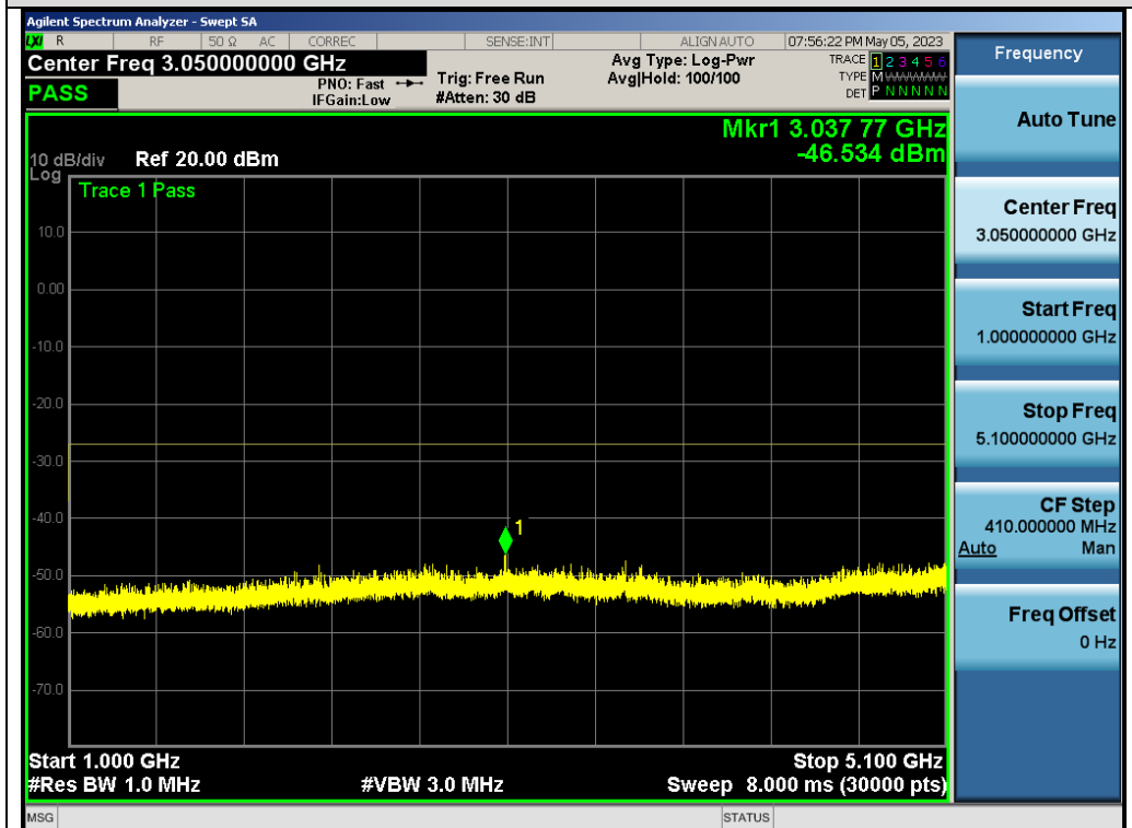
Test_Graph_802.11ac80_ANT2_5290_MCS0_Frequency Band 2
