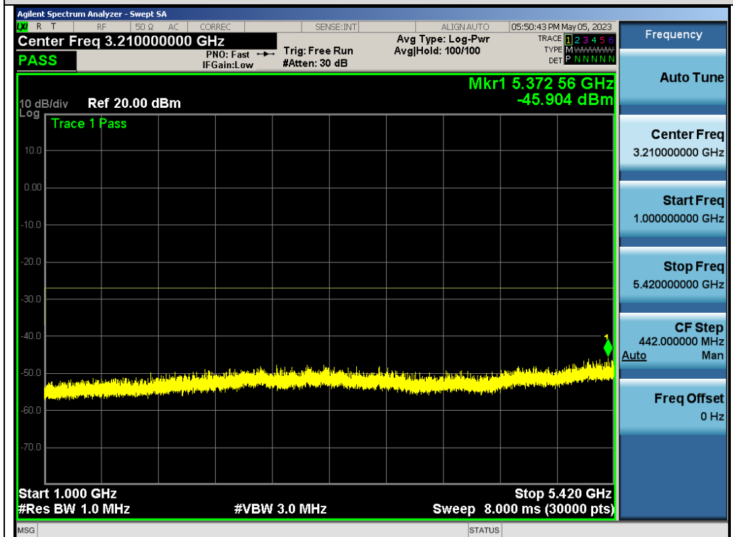
Test_Graph_802.11n40_ANT1_5590_MCS0_Frequency Band 2
