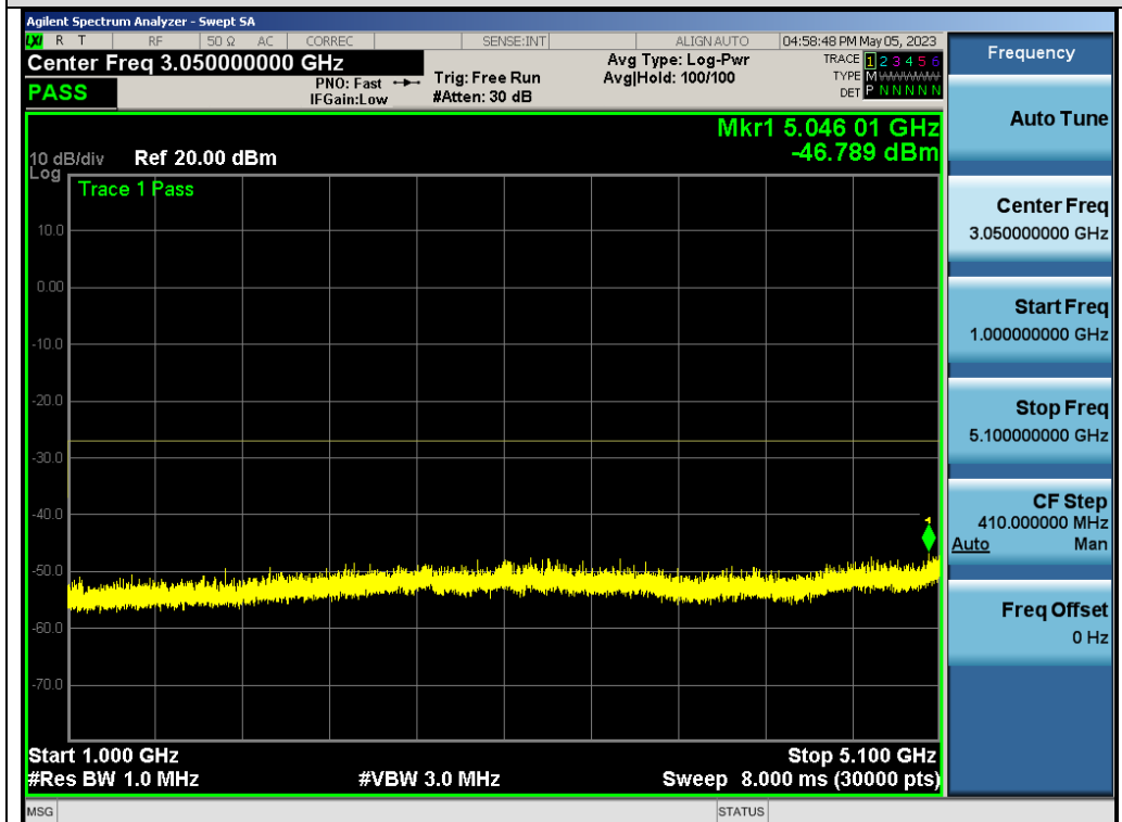
Test_Graph_802.11n40_ANT1_5270_MCS0_Frequency Band 2
