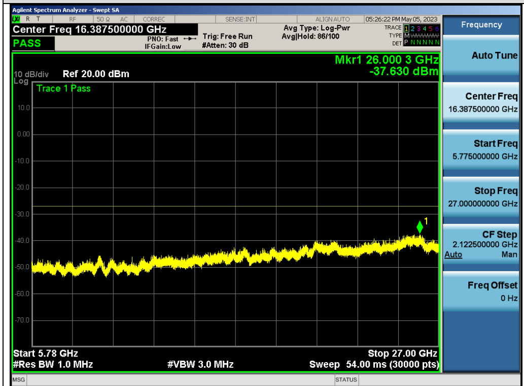
Test_Graph_802.11a_ANT1_5500_6Mbps_Frequency Band 4
