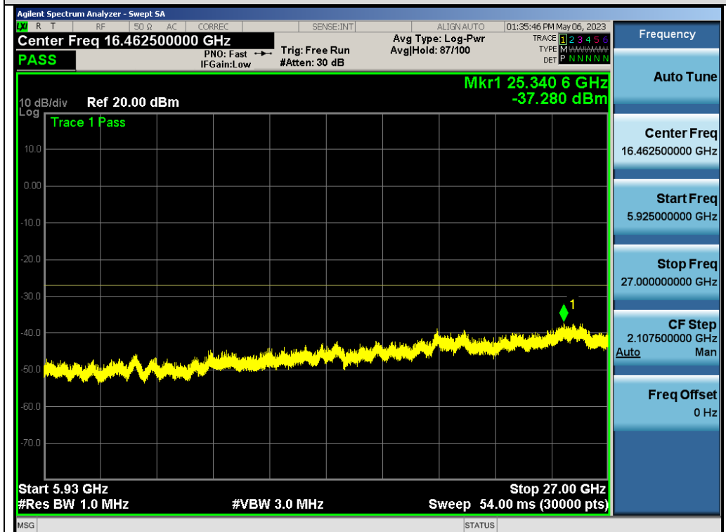
Test_Graph_802.11n40_ANT1_5755_MCS0_Frequency Band4
