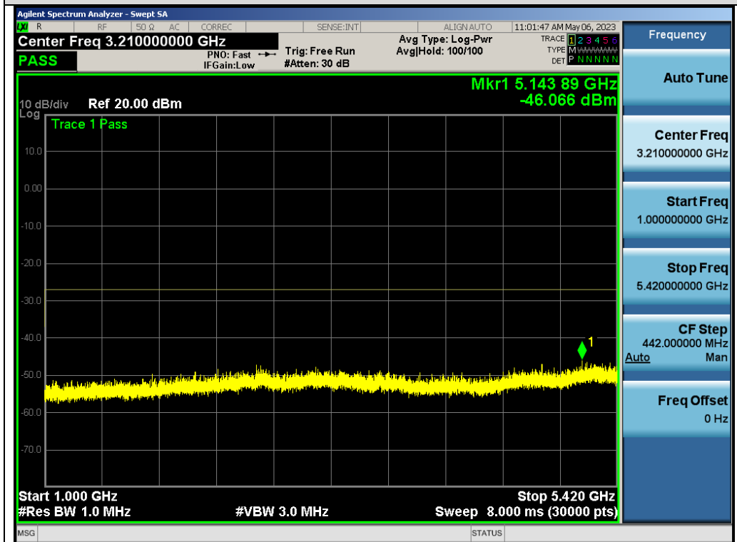
Test_Graph_802.11a_ANT2_5700_6Mbps_Frequency Band 2
