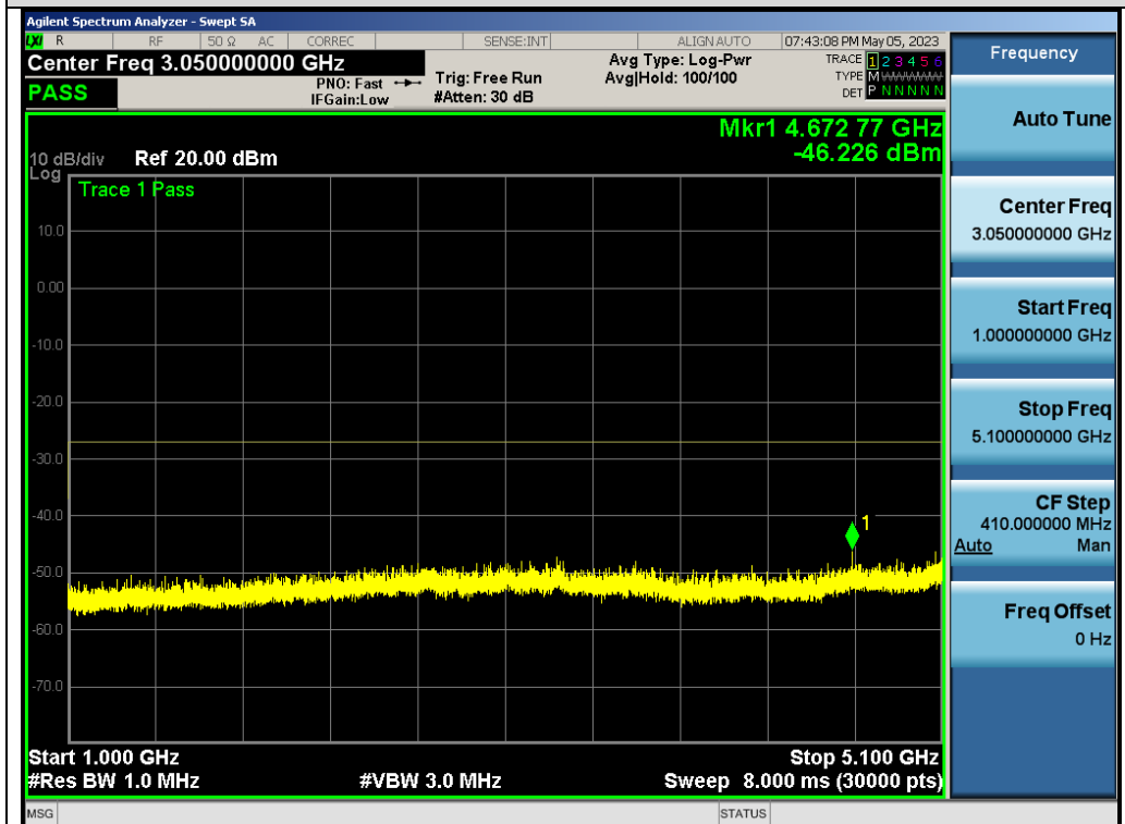
Test_Graph_802.11n40_ANT2_5270_MCS0_Frequency Band 2
