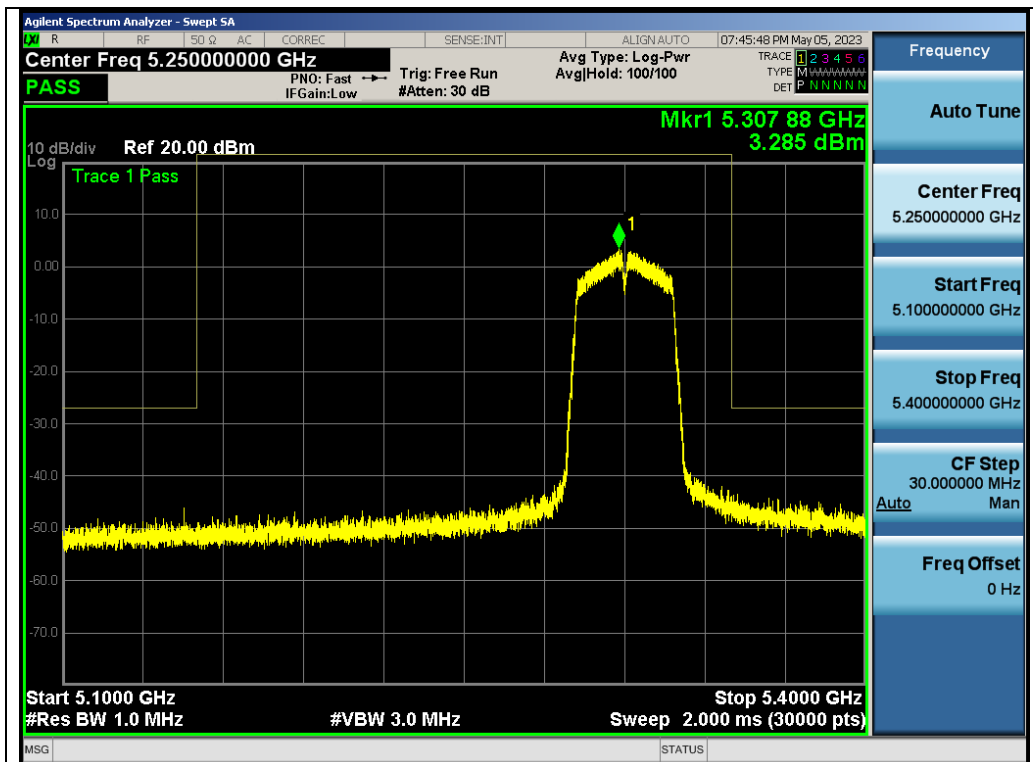
Test_Graph_802.11n40_ANT2_5310_MCS0_Frequency Band 3
