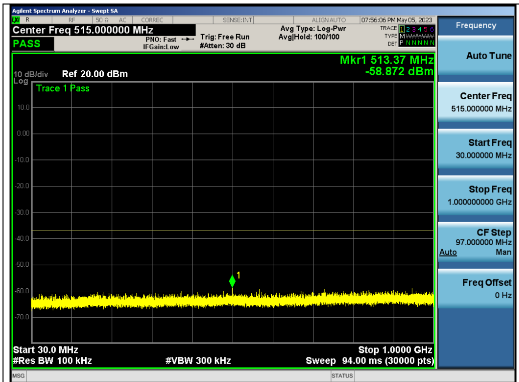
Test_Graph_802.11ac80_ANT2_5290_MCS0_Frequency Band 1
