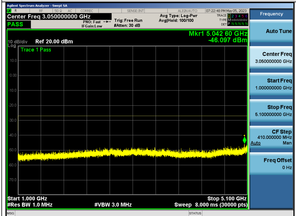
Test_Graph_802.11ac80_ANT2_5210_MCS0_Frequency Band 2
