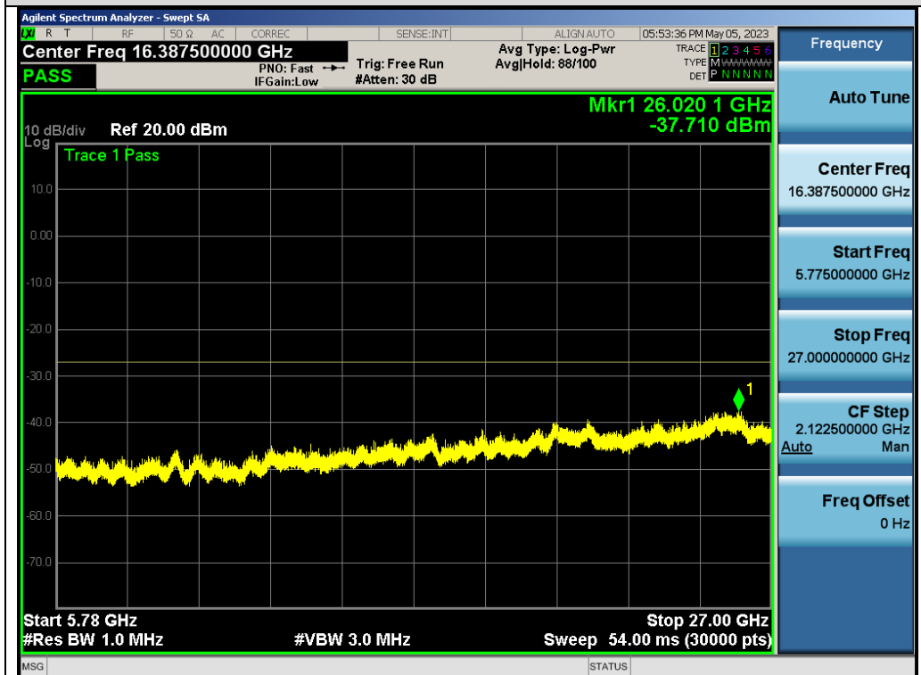
Test_Graph_802.11n40_ANT1_5670_MCS0_Frequency Band 4
