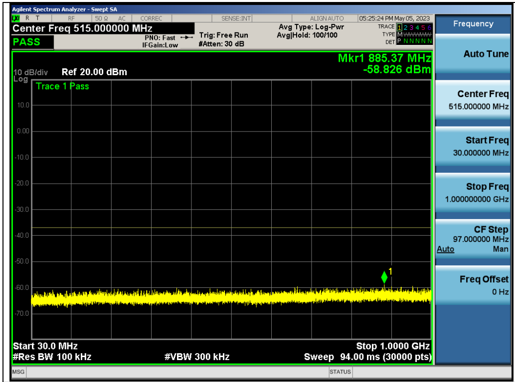
Test_Graph_802.11a_ANT1_5500_6Mbps_Frequency Band 1
