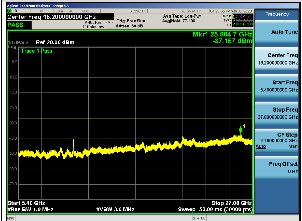
Test_Graph_802.11n40_ANT1_5230_MCS0_Frequency Band 4
