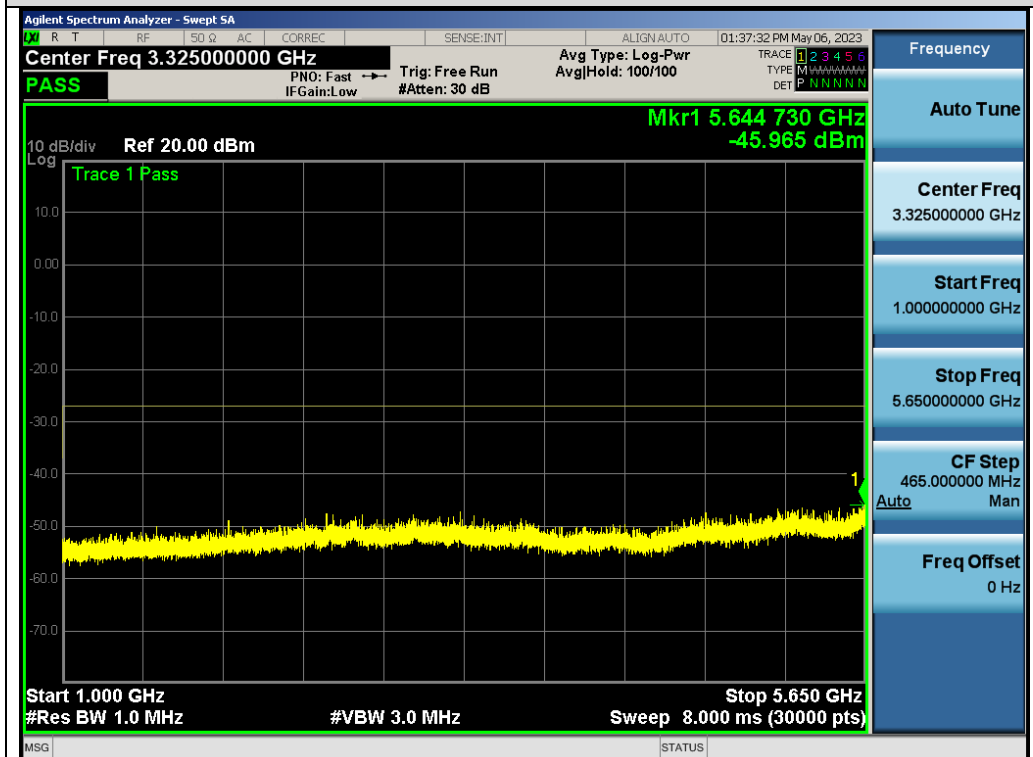
Test_Graph_802.11n40_ANT1_5795_MCS0_Frequency Band2
