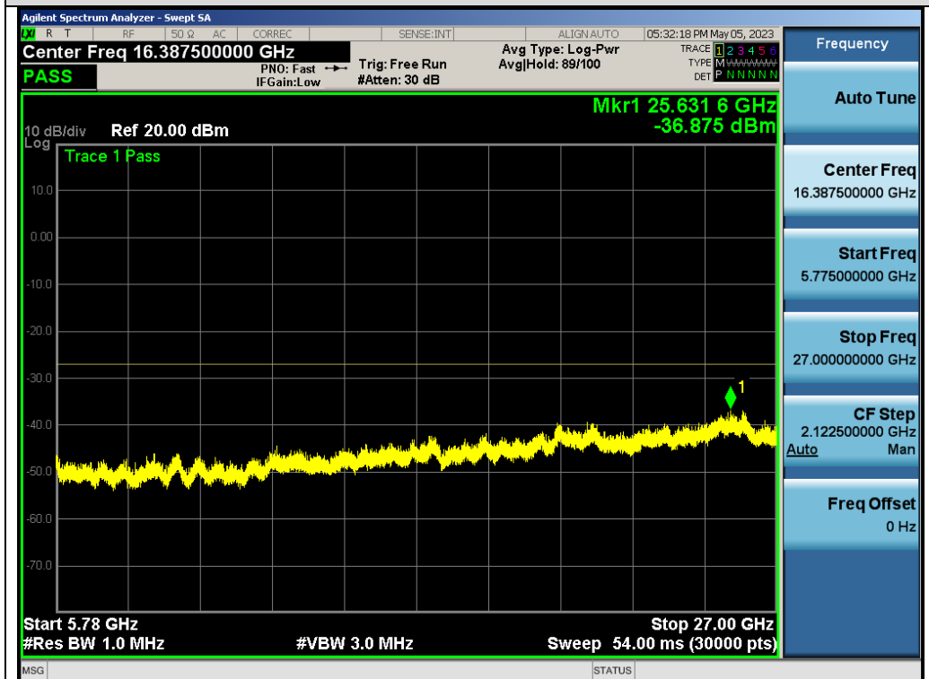
Test_Graph_802.11a_ANT1_5700_6Mbps_Frequency Band 4
