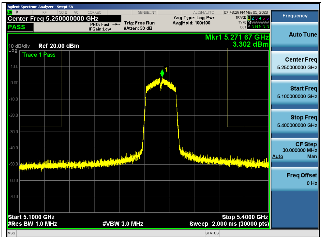
Test_Graph_802.11n40_ANT2_5270_MCS0_Frequency Band 3
