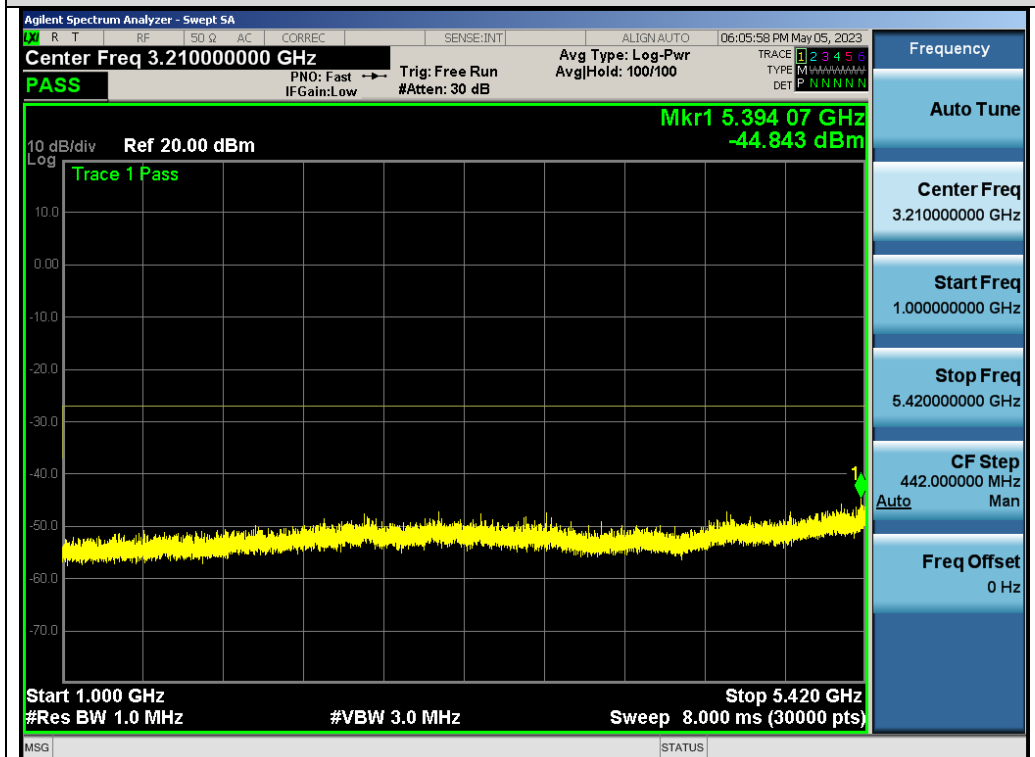
Test_Graph_802.11ac80_ANT1_5530_MCS0_Frequency Band 2
