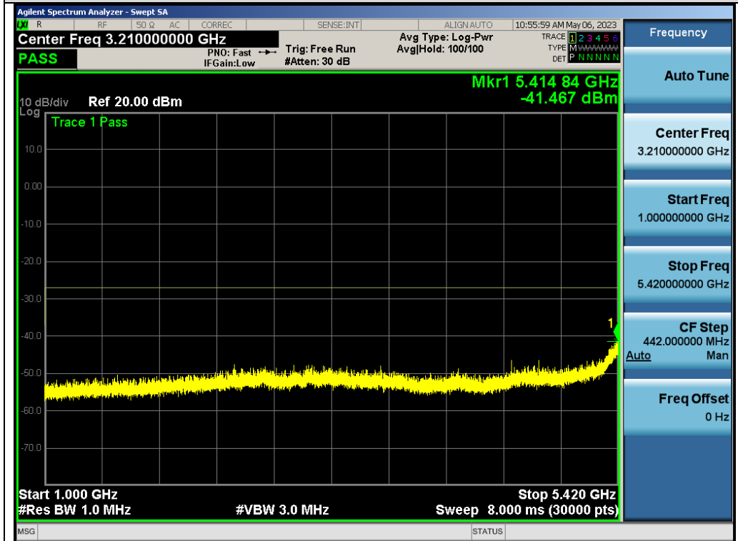
Test_Graph_802.11a_ANT2_5500_6Mbps_Frequency Band 2
