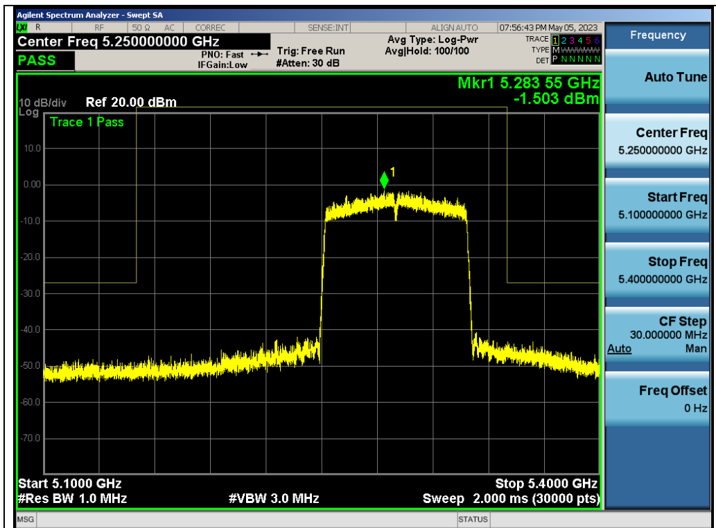
Test_Graph_802.11ac80_ANT2_5290_MCS0_Frequency Band 3
