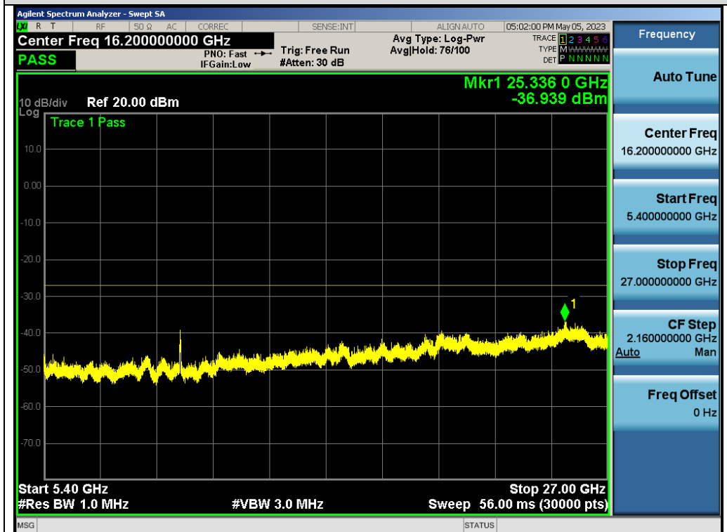
Test_Graph_802.11n40_ANT1_5310_MCS0_Frequency Band 4
