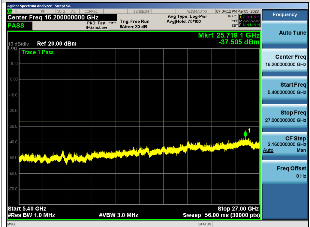
Test_Graph_802.11n40_ANT2_5190_MCS0_Frequency Band 4
