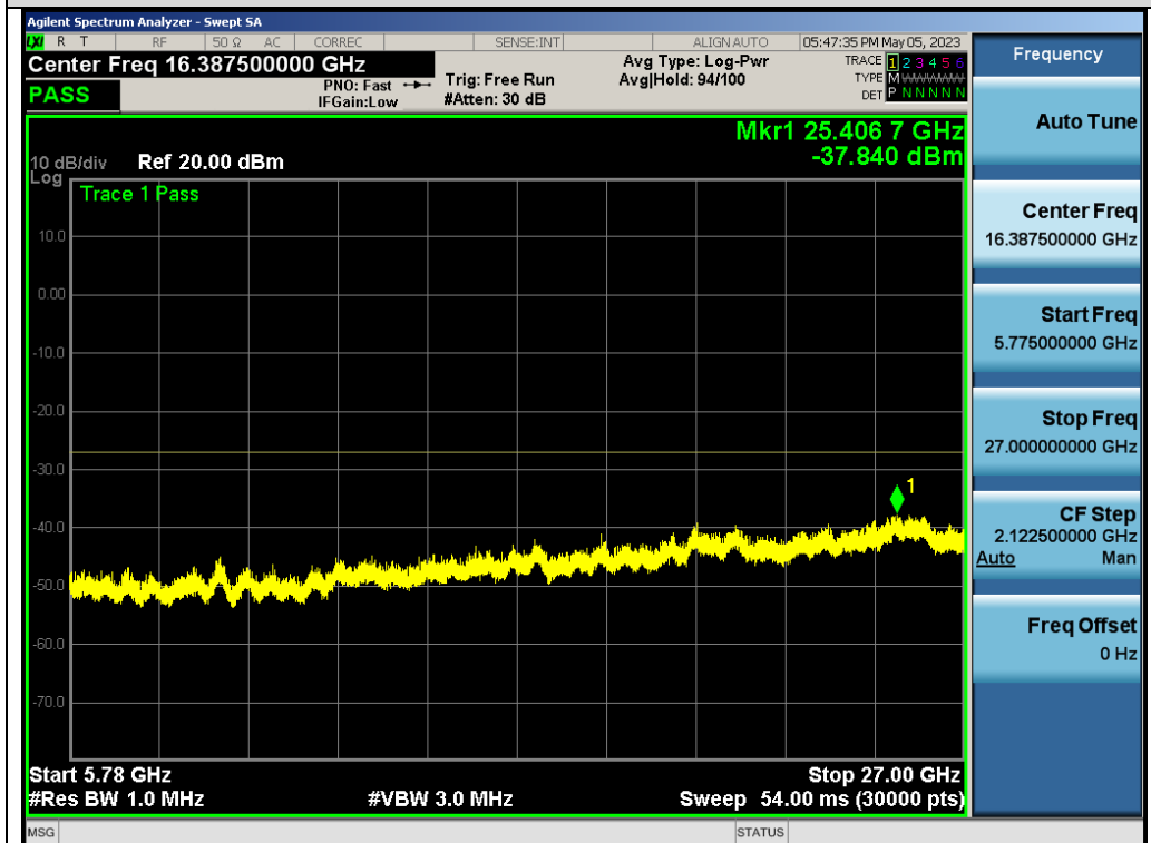
Test_Graph_802.11n40_ANT1_5510_MCS0_Frequency Band 4
