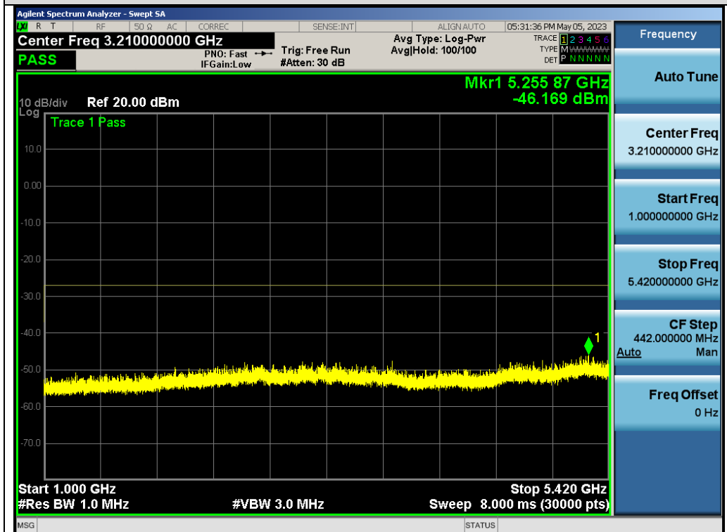
Test_Graph_802.11a_ANT1_5700_6Mbps_Frequency Band 2
