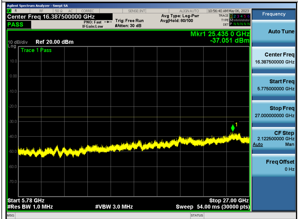
Test_Graph_802.11a_ANT2_5500_6Mbps_Frequency Band 4
