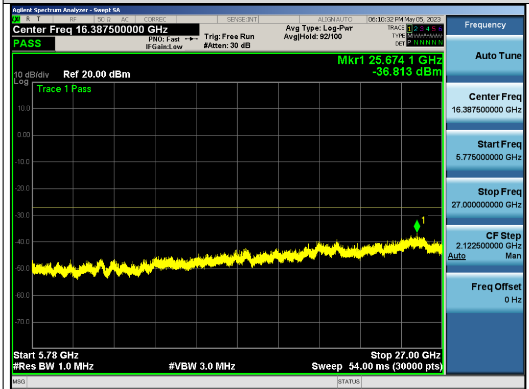
Test_Graph_802.11ac80_ANT1_5610_MCS0_Frequency Band 4
