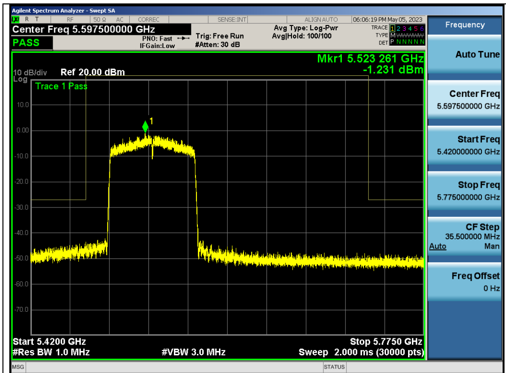
Test_Graph_802.11ac80_ANT1_5530_MCS0_Frequency Band 3
