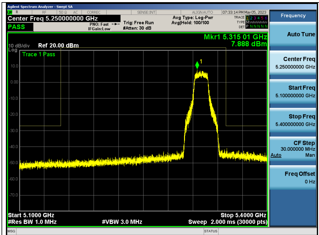
Test_Graph_802.11a_ANT2_5320_6Mbps_Frequency Band 3
