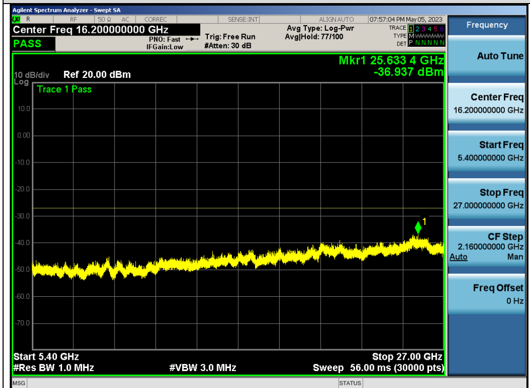
Test_Graph_802.11ac80_ANT2_5290_MCS0_Frequency Band 4
