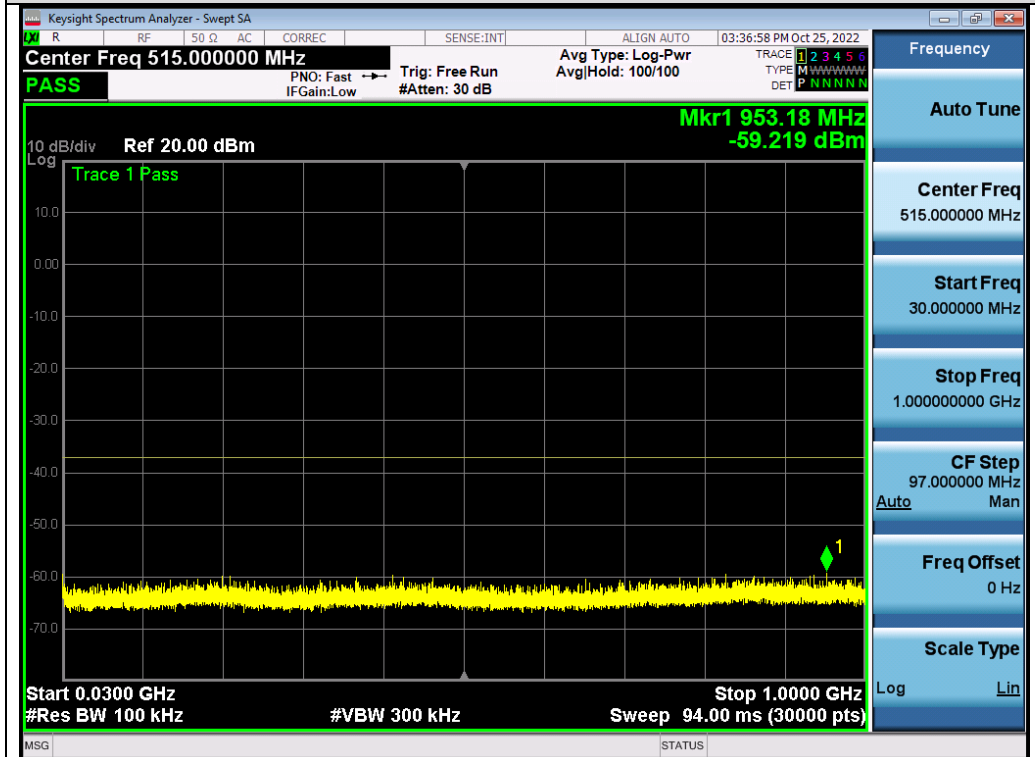
Test_Graph_802.11n40_ANT2_5670_MCS0_Frequency Band 1
