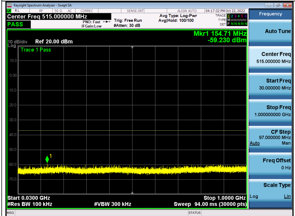
Test_Graph_802.11a_ANT2_5745_6Mbps_Frequency Band1
