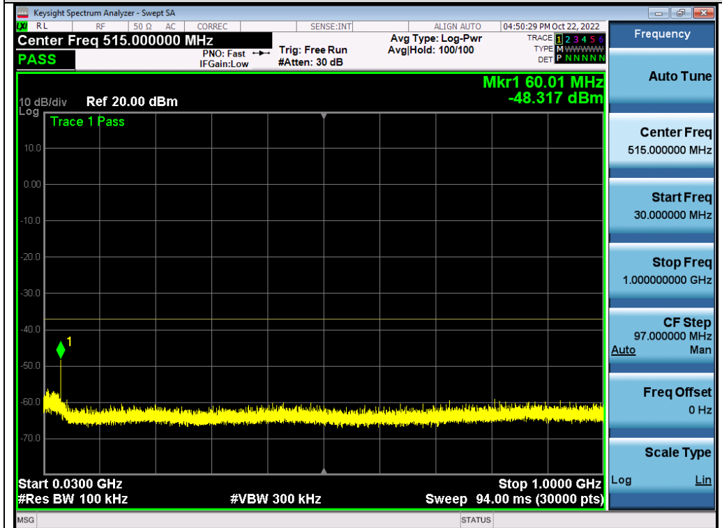
Test_Graph_802.11ac80_ANT2_5775_MCS9_Frequency Band1
