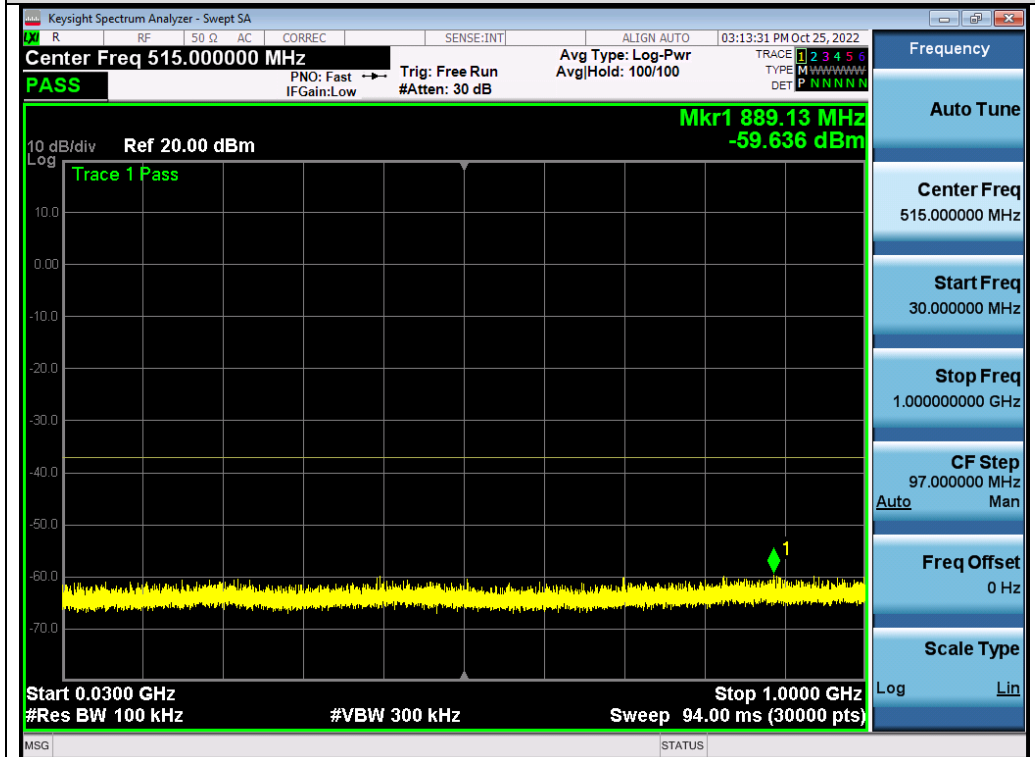
Test_Graph_802.11a_ANT2_5500_6Mbps_Frequency Band 1
