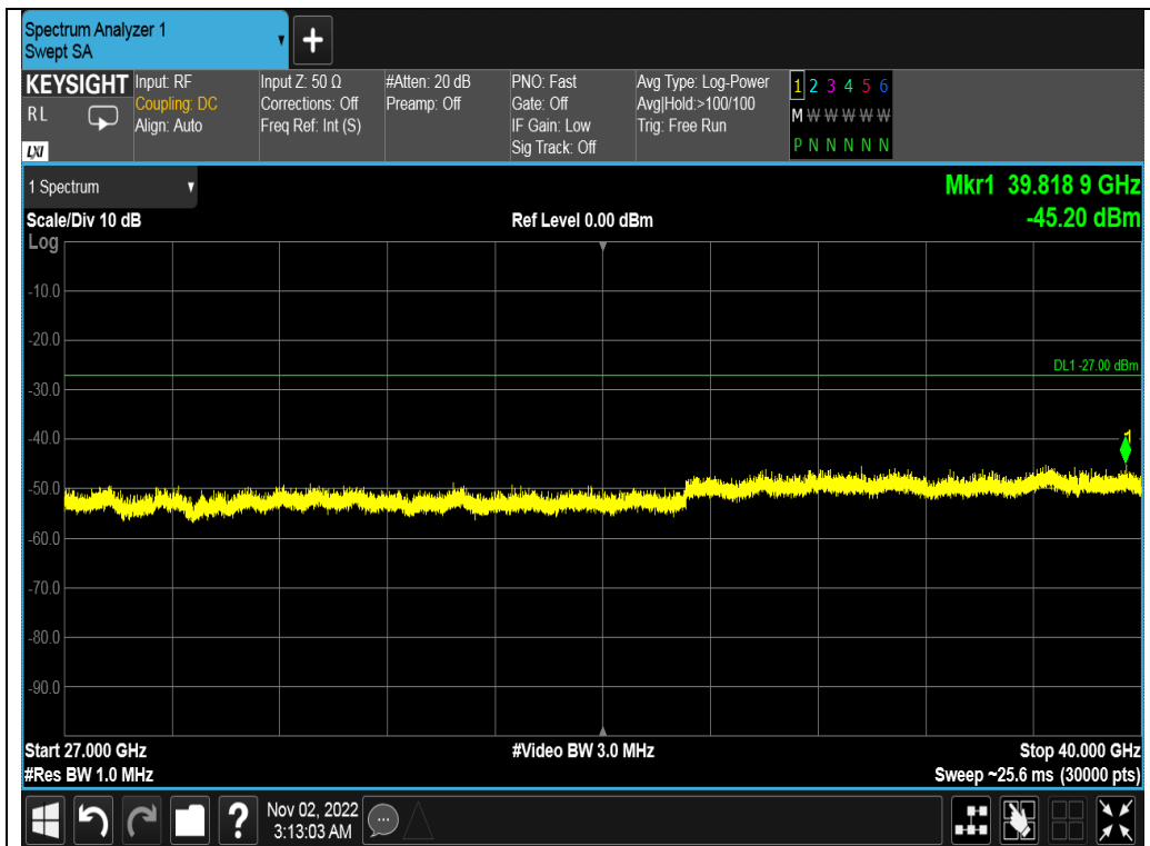
Test_Graph_802.11n40_ANT2_5795_MCS0_Frequency Band5
