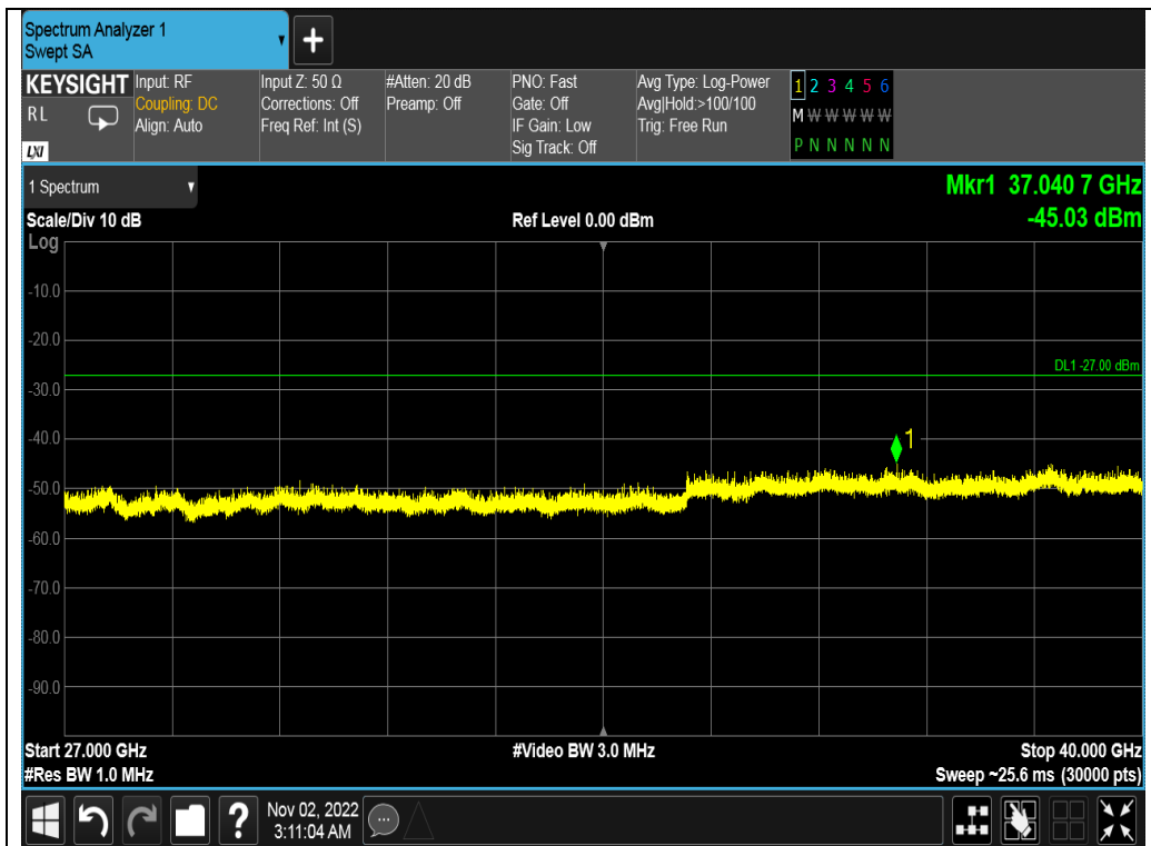
Test_Graph_802.11a_ANT2_5825_6Mbps_Frequency Band5
