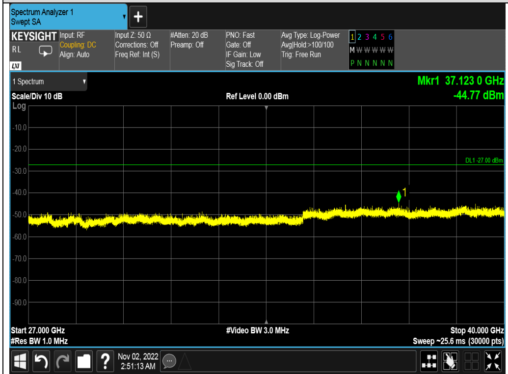
Test_Graph_802.11a_ANT2_5500_6Mbps_Frequency Band 5
