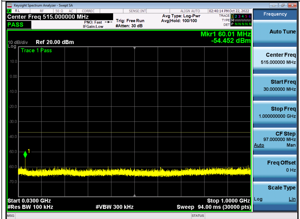
Test_Graph_802.11ac80_ANT1_5530_MCS9_Frequency Band 1
