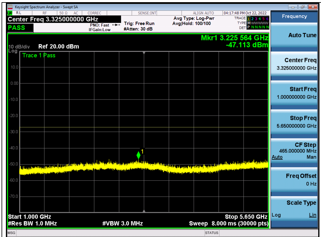
Test_Graph_802.11a_ANT2_5745_6Mbps_Frequency Band2
