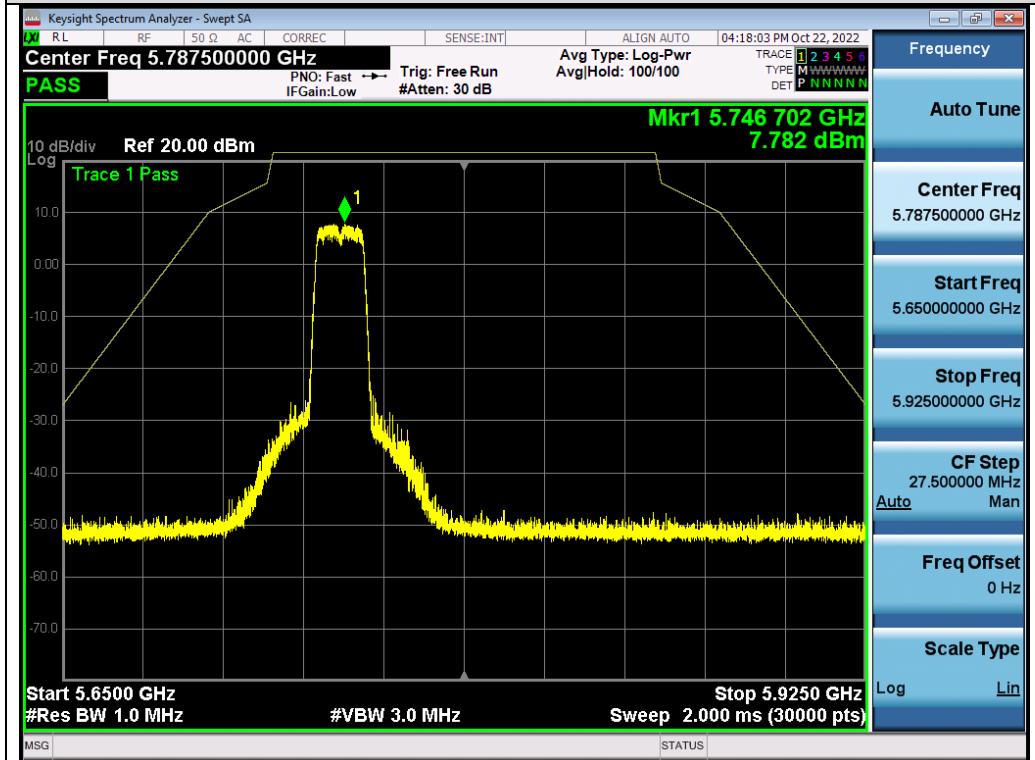
Test_Graph_802.11a_ANT2_5745_6Mbps_Frequency Band3
