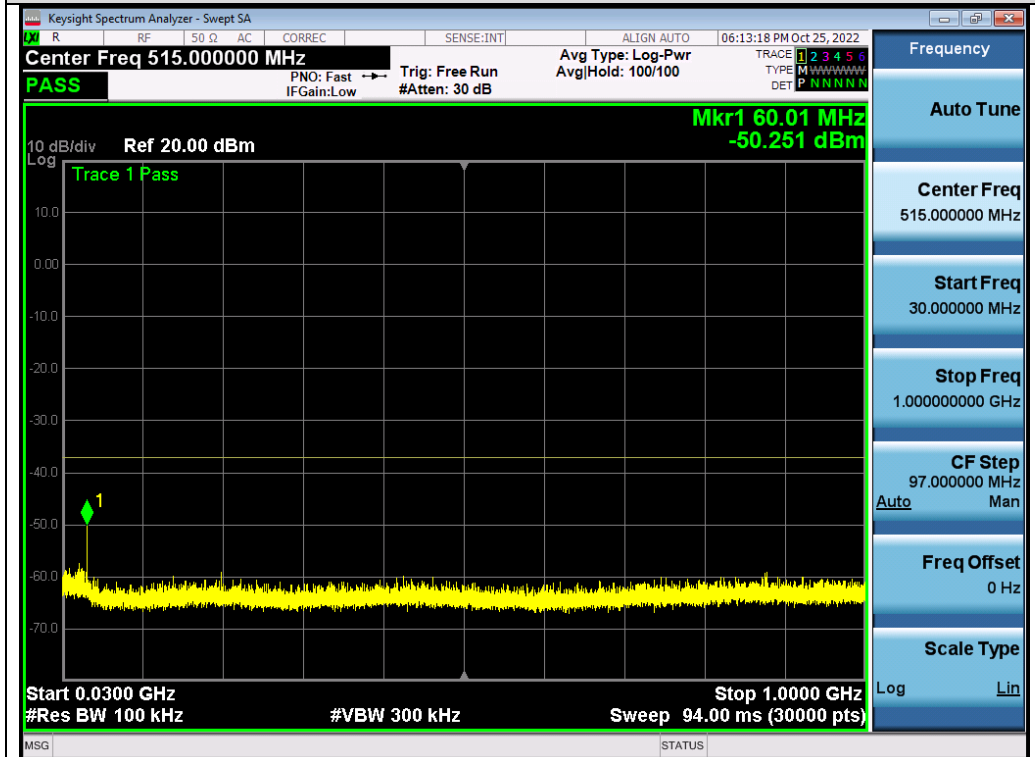
Test_Graph_802.11ac80_ANT2_5610_MCS9_Frequency Band 1
