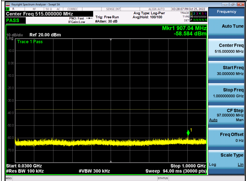
Test_Graph_802.11n40_ANT2_5510_MCS0_Frequency Band 1
