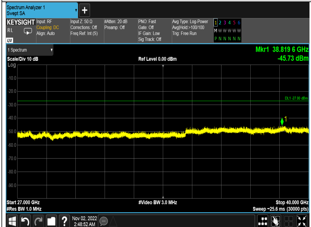
Test_Graph_802.11ac80_ANT1_5530_MCS9_Frequency Band 5
