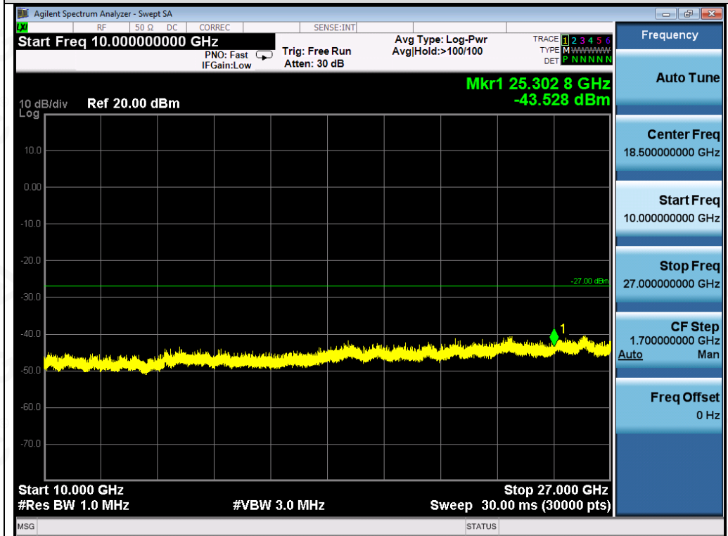
Test_Graph_802.11a_ANT1_5825_6Mbps_Frequency Band5
