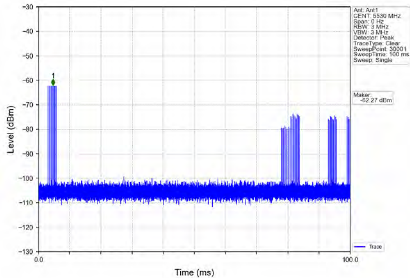
Signal Calibration 802.11ac(VHT80) 2A 5530MHz RadarType6 Trial0
