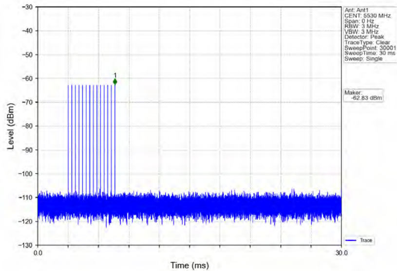
Signal Calibration 802.11ac(VHT80) 2A 5530MHz RadarType5 Trial0
