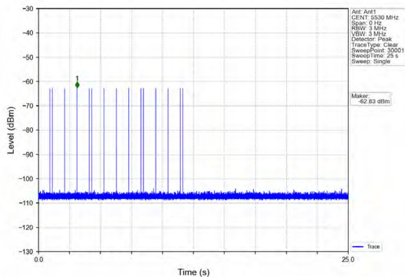
Signal Calibration 802.11ac(VHT80) 2A 5530MHz RadarType5 Trial0
