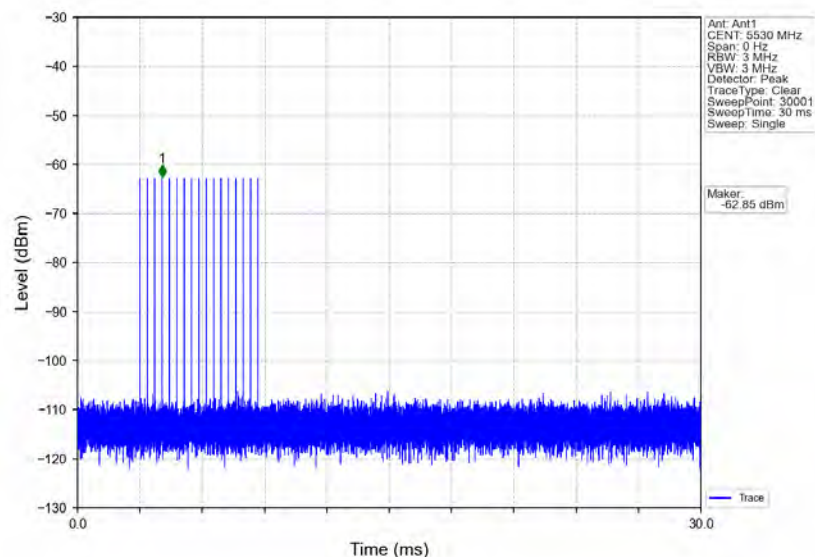
Signal Calibration 802.11ac(VHT80) 2A 5530MHz RadarType3 Trial0
