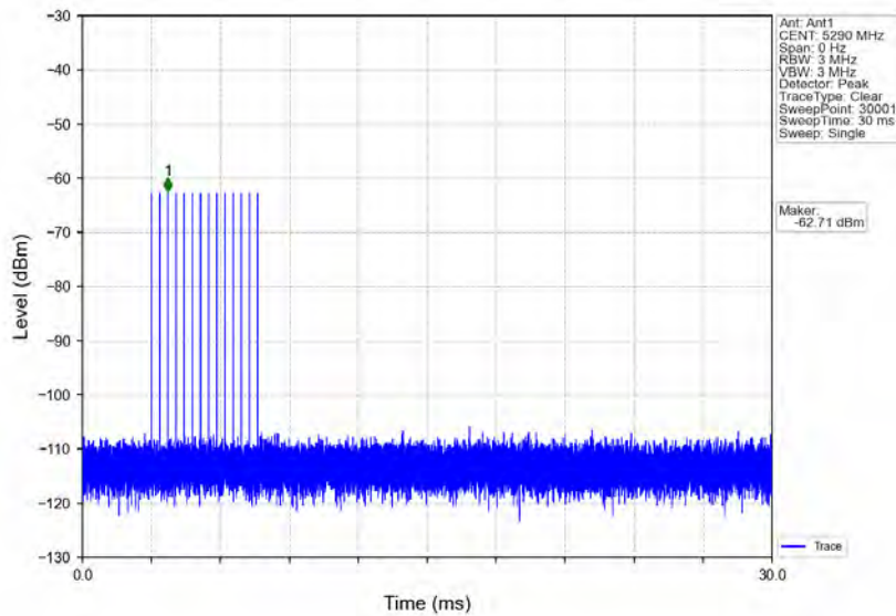
Signal Calibration 802.11ac(VHT80) 2C 5290MHz RadarType5 Trial0
