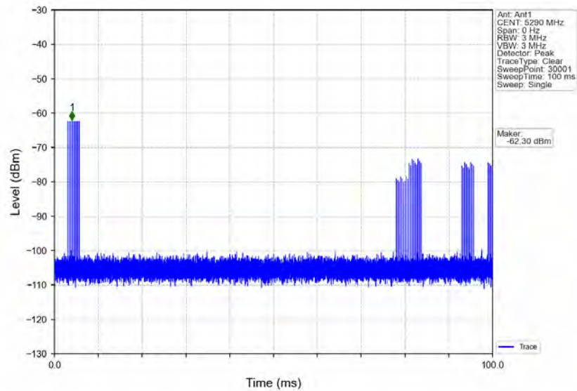
Signal Calibration 802.11ac(VHT80) 2C 5290MHz RadarType6 Trial0
