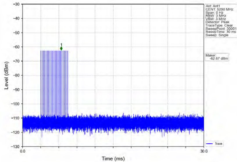
Signal Calibration 802.11ac(VHT80) 2C 5290MHz RadarType3 Trial0
